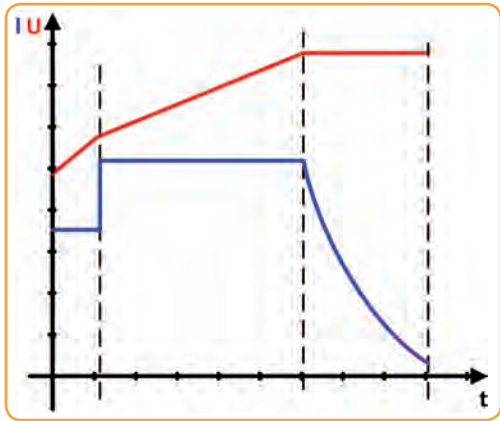
Charging profile for Lilo batteries
