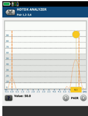
High Definition Time Domain Cross talk (HTDIX) shows the far end connection is clearly the issue
