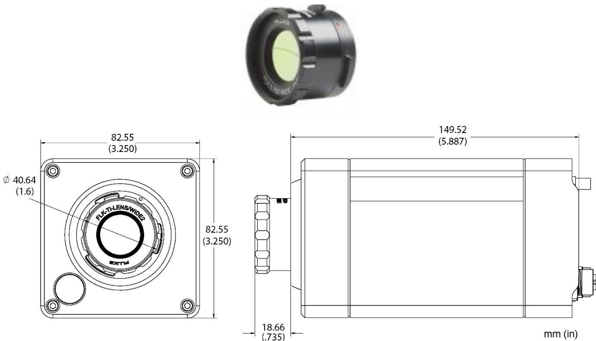
Figure 7-1: Wide Lens
