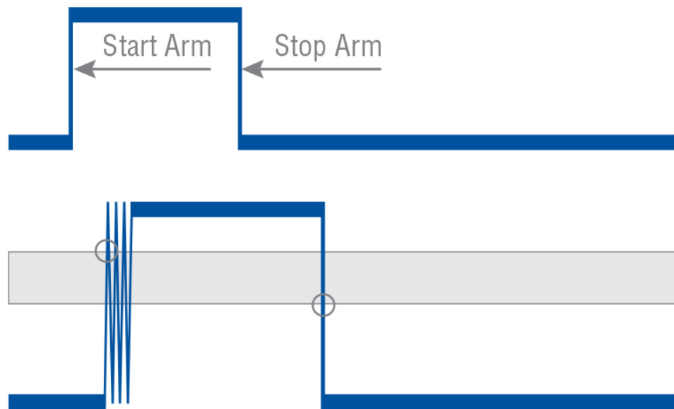
Fig. 4.23: Using start/stop arming as an external Hold-Off
