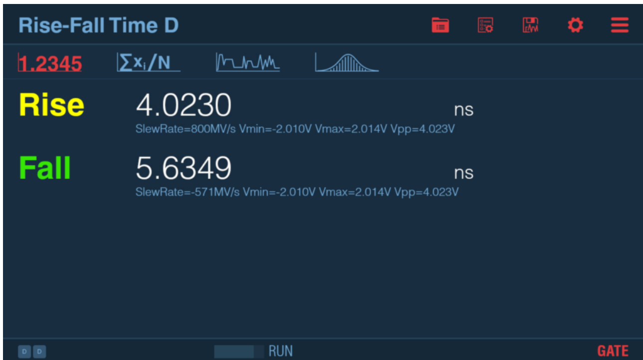
Fig. 5.18: Rise Time vs Rise-Fall Time
