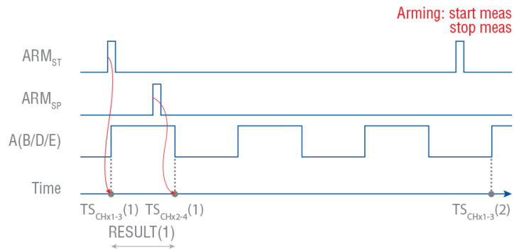
Fig. 4.19: Pulse width measurement with arming on sample and start and stop arming active, case 1
