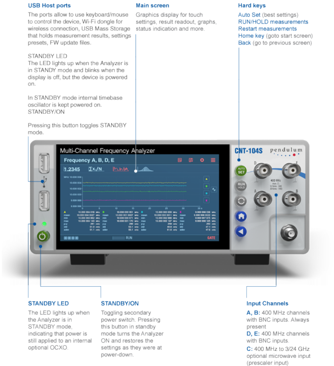
Fig. 3.1: Front panel of CNT-104S
