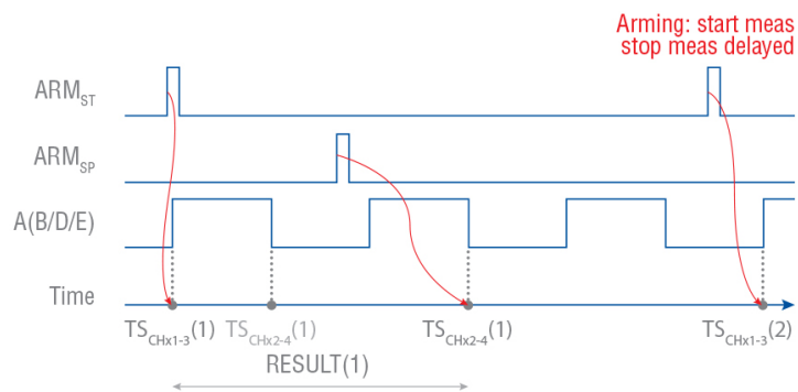
Fig. 4.20: Pulse width measurement with arming on sample, start and stop arming active, case 2
