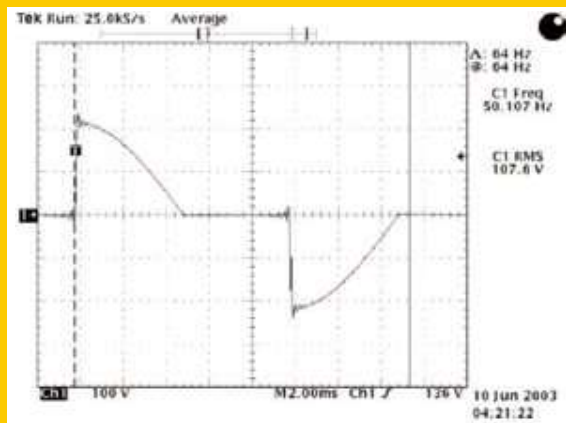
Phase-fired waveform
