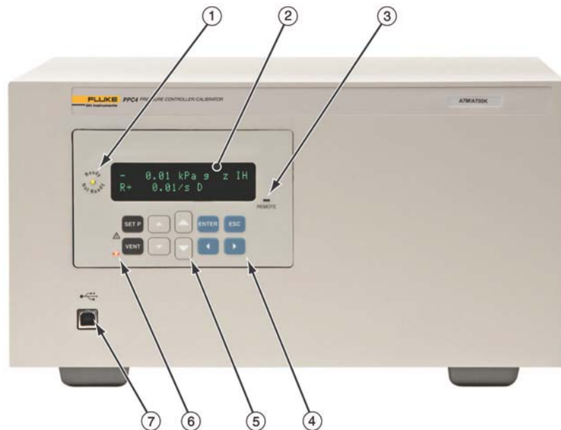
Figure 1. PPC4 advanced interface front panel
