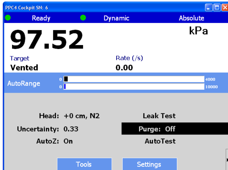
Figure 20. PPC4 Cockpit Main Display
