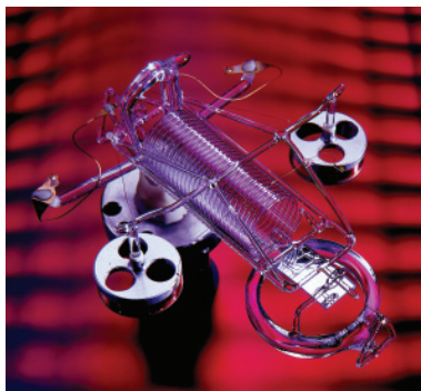
The 7250LP features a unique fused-quartz sensor. This rugged transducer offers unequalled precision and a stability of 0.0075% of reading per year. The media is in direct contact with the quartz, eliminating mechanical linkages and diaphragms, to provide the highest performance available in an automatic controller.
