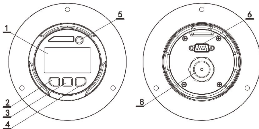
Figure 2 Basic Structure of ADT680P/680PEX
