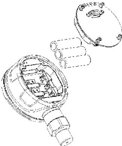
Figure 3 Install batteries
