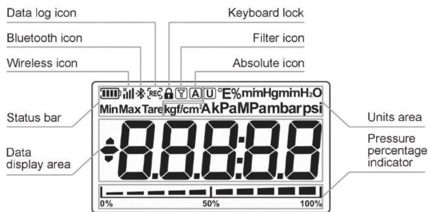
Figure 5 Main Display
