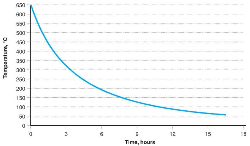
Figure 13 9260 Comparison Block Cool Down
