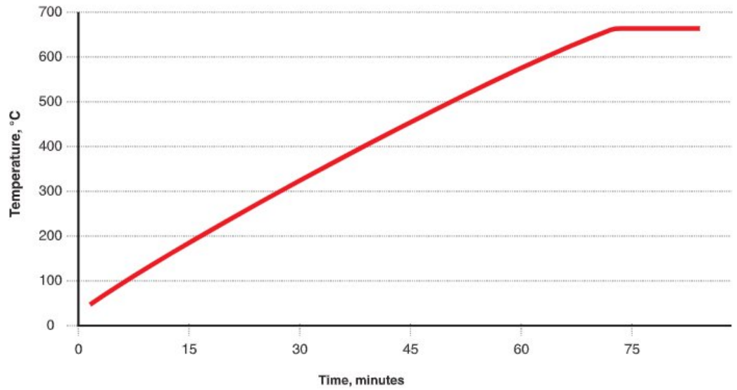
Figure 12 9260 Comparison Block Heating Up
