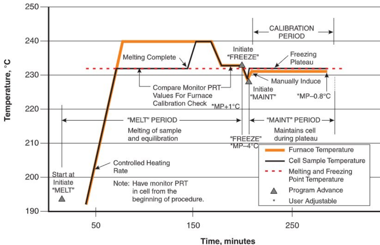
Figure 11 Freezing Point Realization
