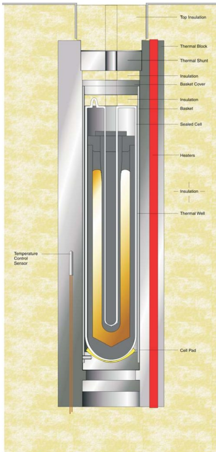
Figure 5 Thermal Block Assembly
