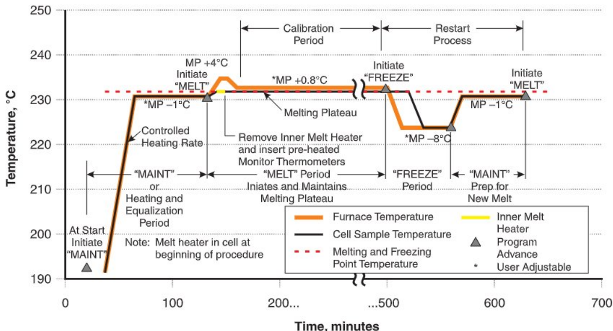
Figure 10 Melting Point Realization
