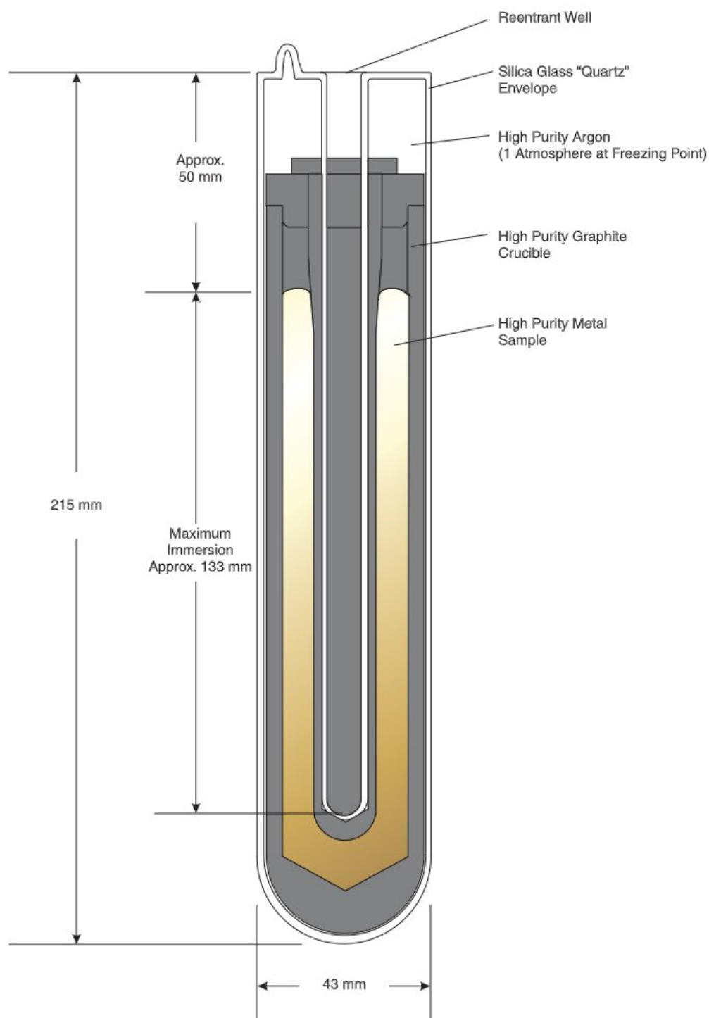
Figure 6 Typical Sealed Mini Fixed-Point Cell
