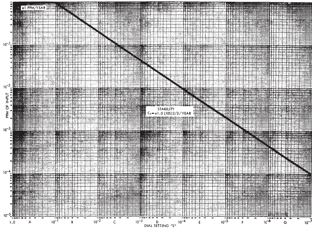
Figure 1-2. STABILITY
