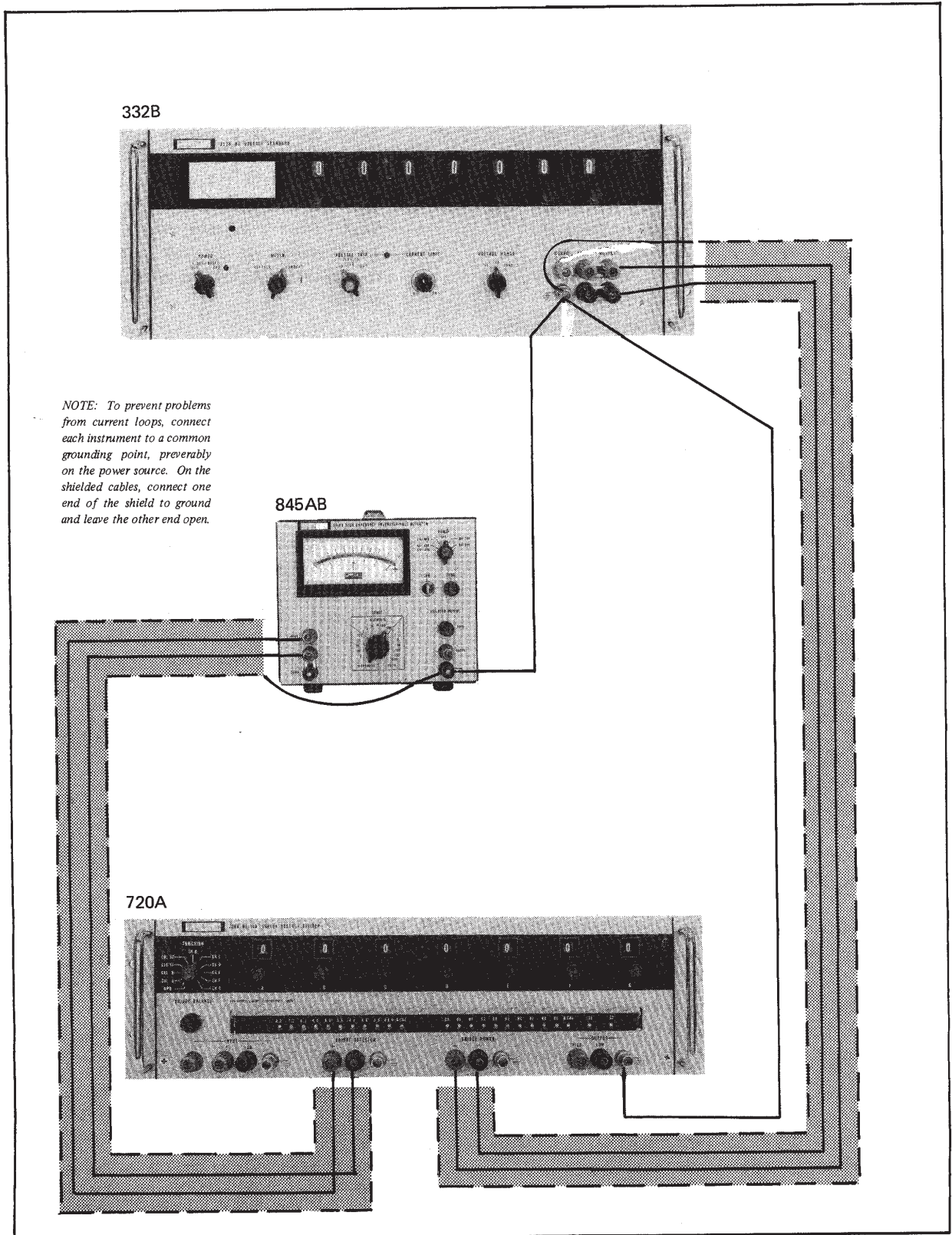
Figure 4-14. EQUIPMENT CONNECTIONS FOR SELF CALIBRATION.
