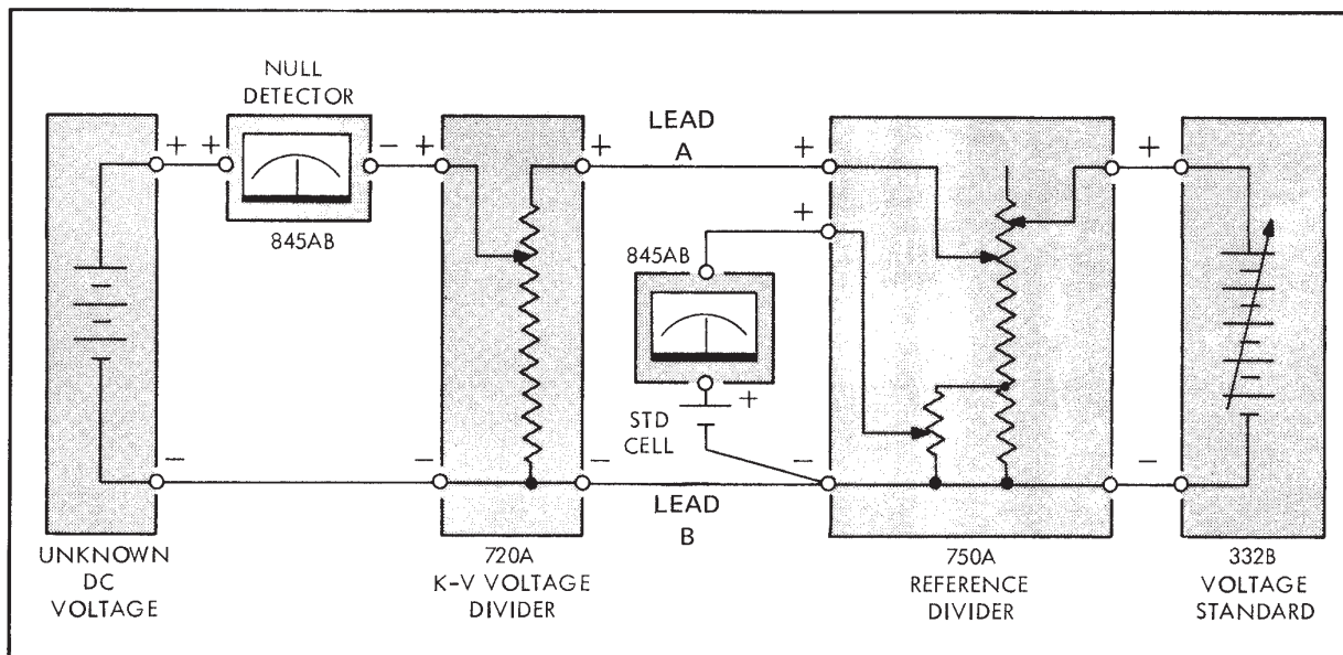
Figure 2-10. EQUIPMENT CONNECTIONS FOR VOLTAGE MEASUREMENTS (Sheet 2 of 2)
