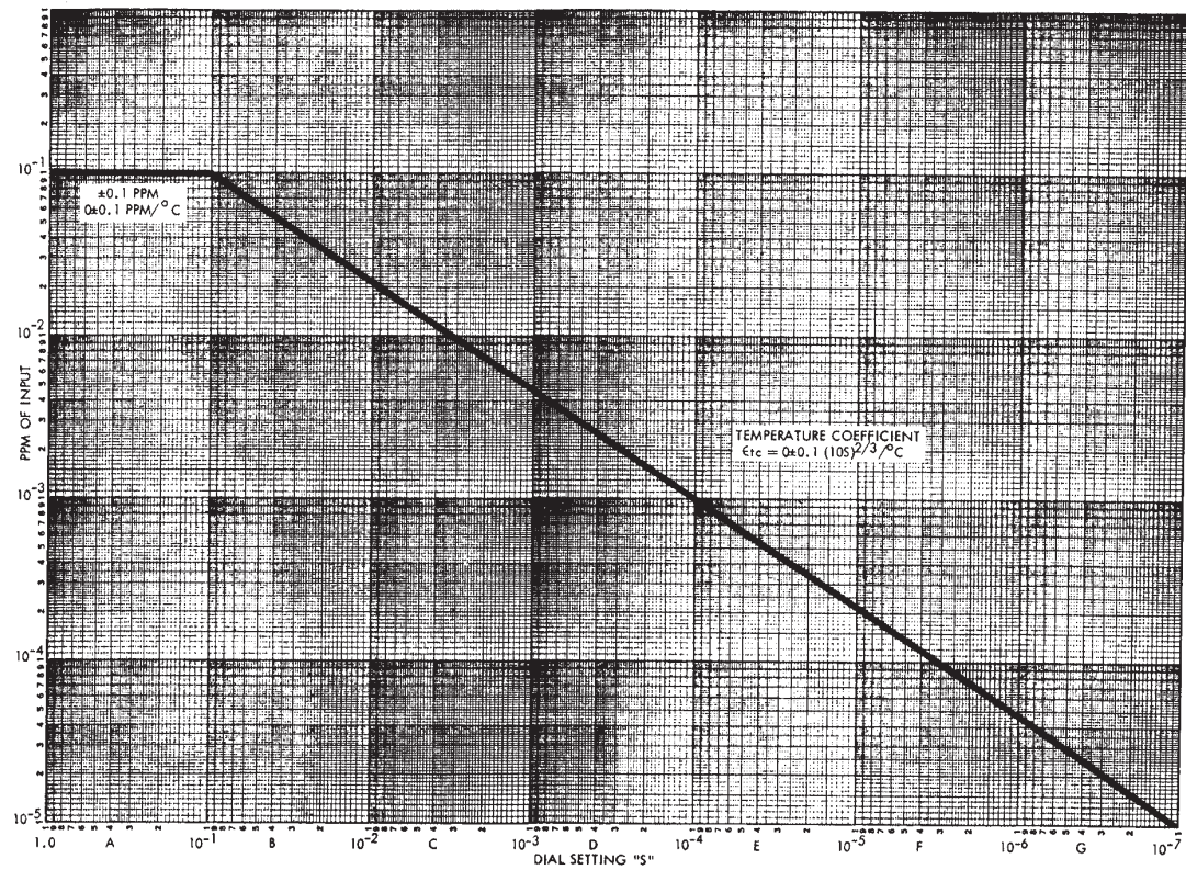
Figure 1-3. TEMPERATURE COEFFICIENT
