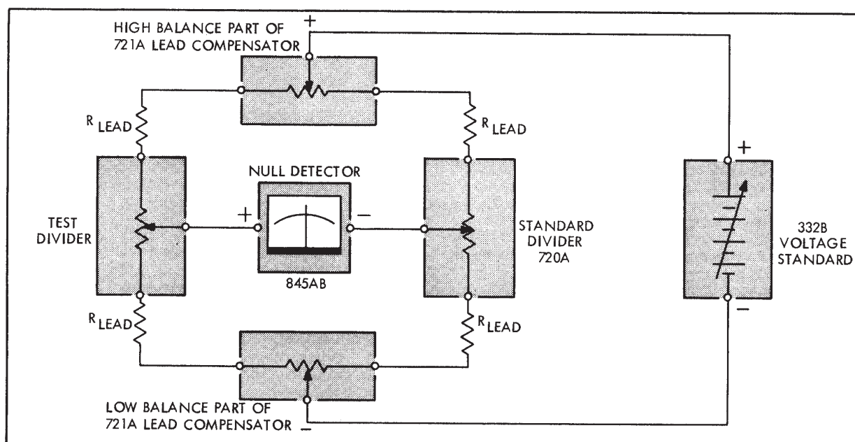
Figure 2-8. SIMPLIFIED SCHEMATIC DIAGRAM OF VOLTAGE DIVIDER CALIBRATION
