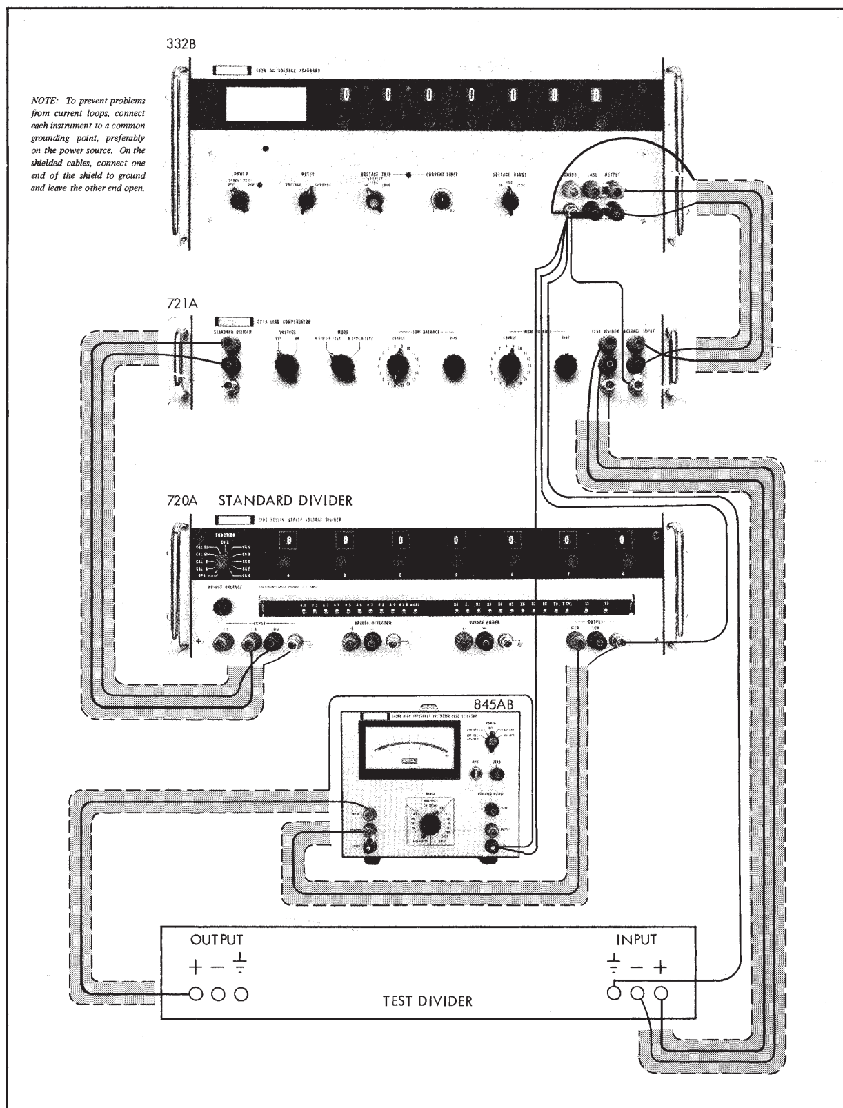
Figure 2-7. EQUIPMENT CONNECTIONS FOR CALIBRATING A VOLTAGE DIVIDER
