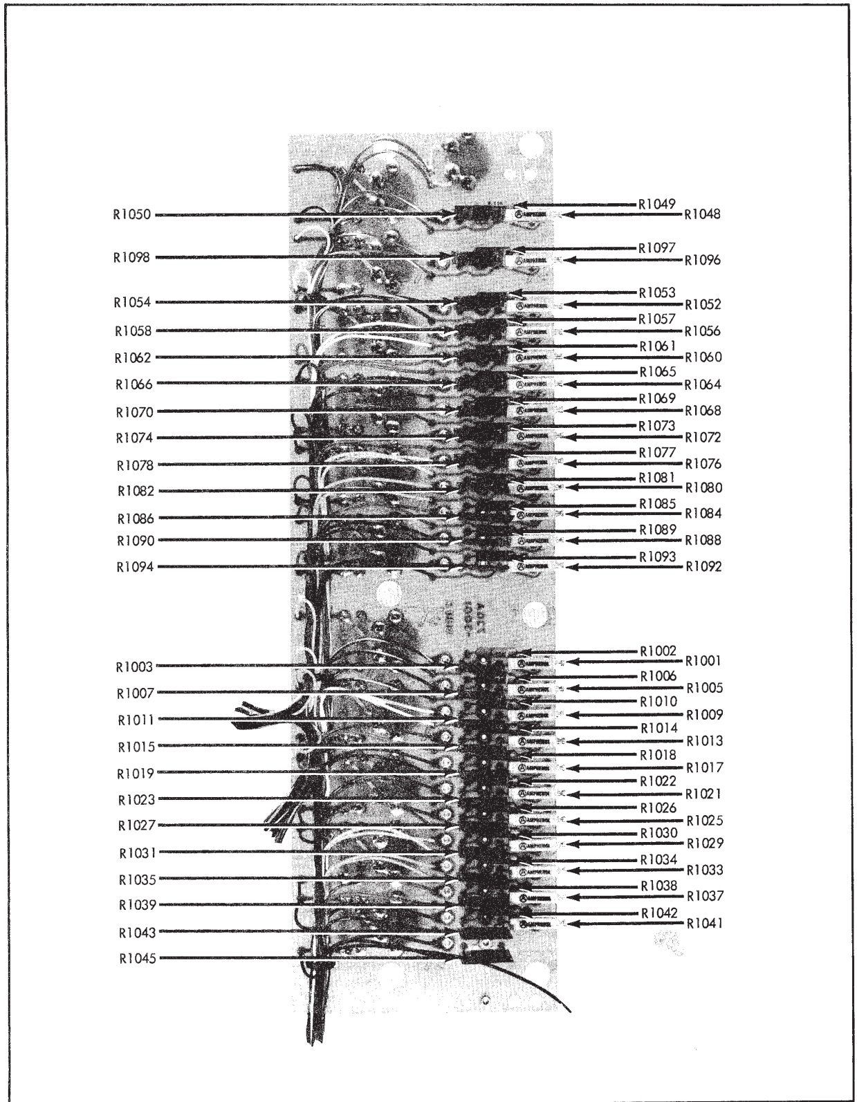
Figure 5-3. TRIMMER P/C ASSEMBLY (Sheet 2 of 2)
