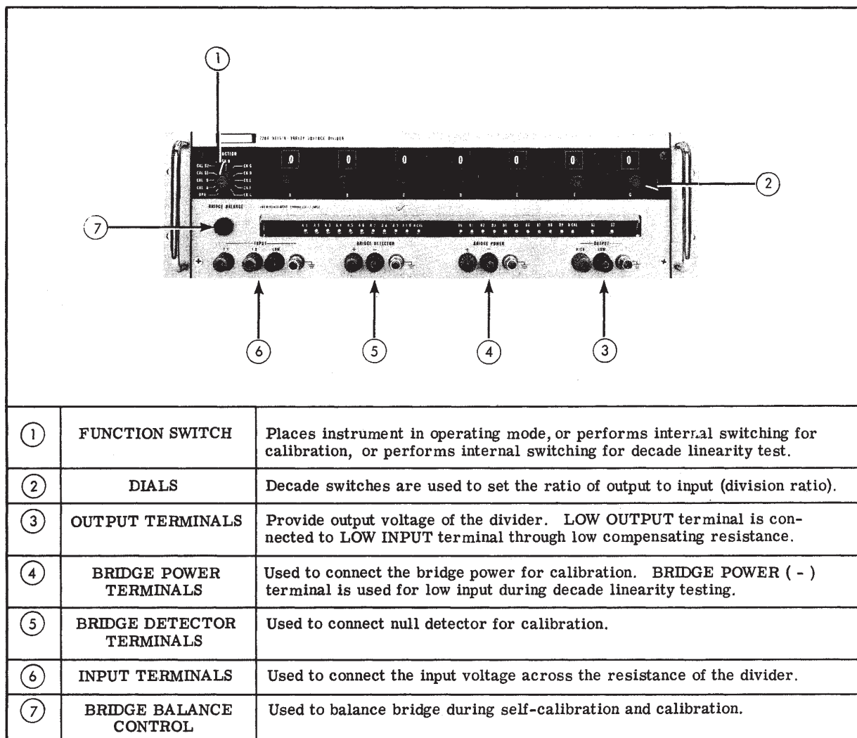
Figure 2-1. FUNCTIONS OF CONTROLS AND TERMINALS
