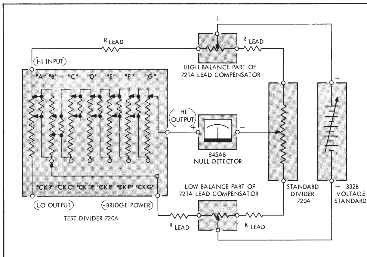
Figure 4-6. SIMPLIFIED SCHEMATIC DIAGRAM OF DECADE LINEARITY TEST
