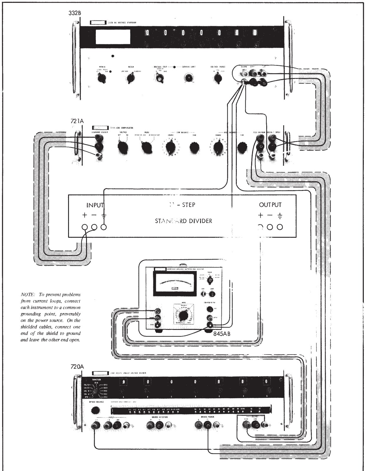
Figure 4-5. EQUIPMENT CONNECTIONS FOR DECADE LINEARITY TEST
