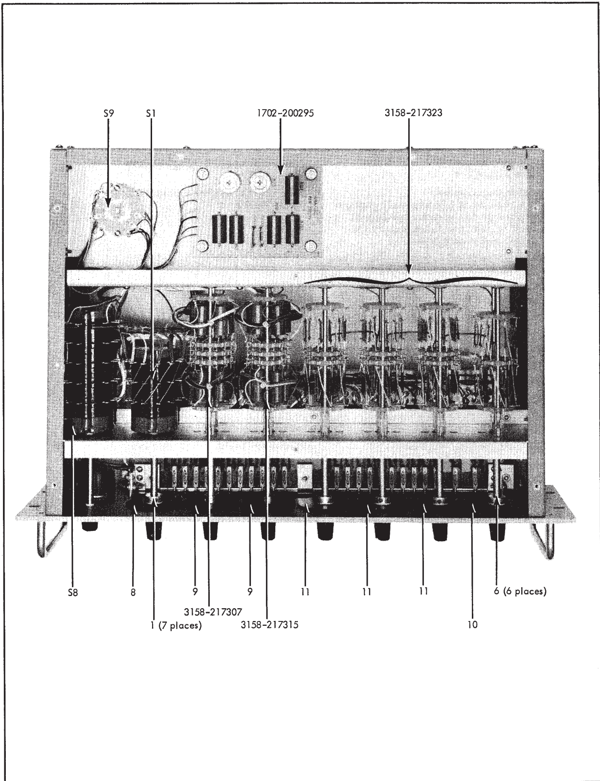
Figure 5-1. 720A KELVIN-VARLEY VOLTAGE DIVIDER (Sheet 1 of 2)
