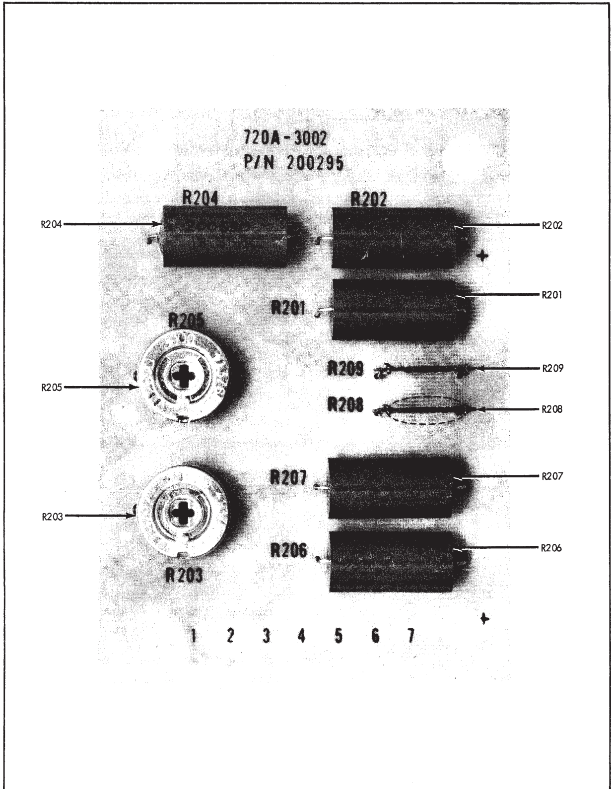
Figure 5-4. BRIDGE P/C ASSEMBLY
