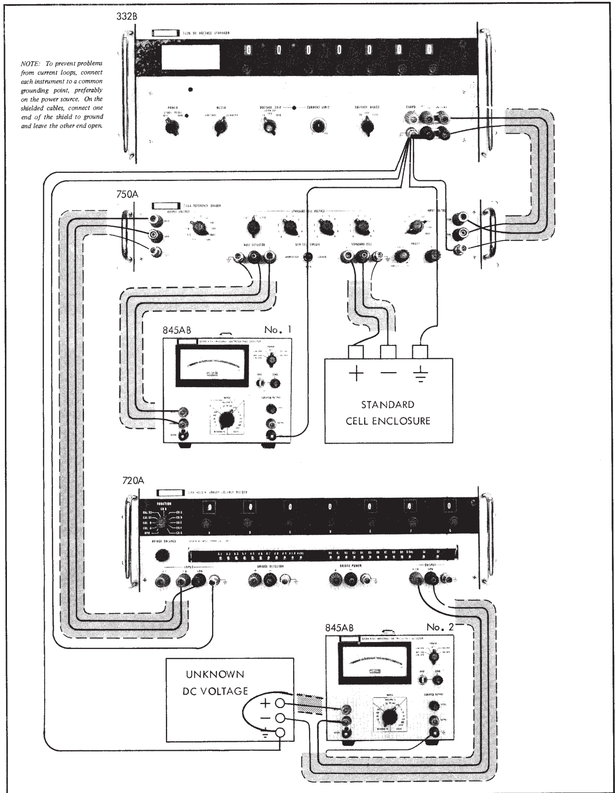
Figure 2-10. EQUIPMENT CONNECTIONS FOR VOLTAGE MEASUREMENTS (Sheet 1 of 2)
