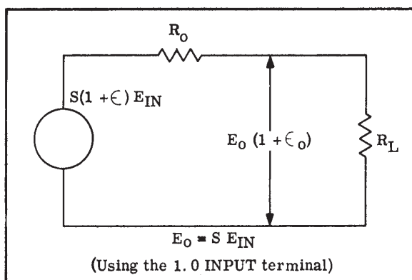
Figure 2-2. THEVININ EQUIVALENT CIRCUIT
