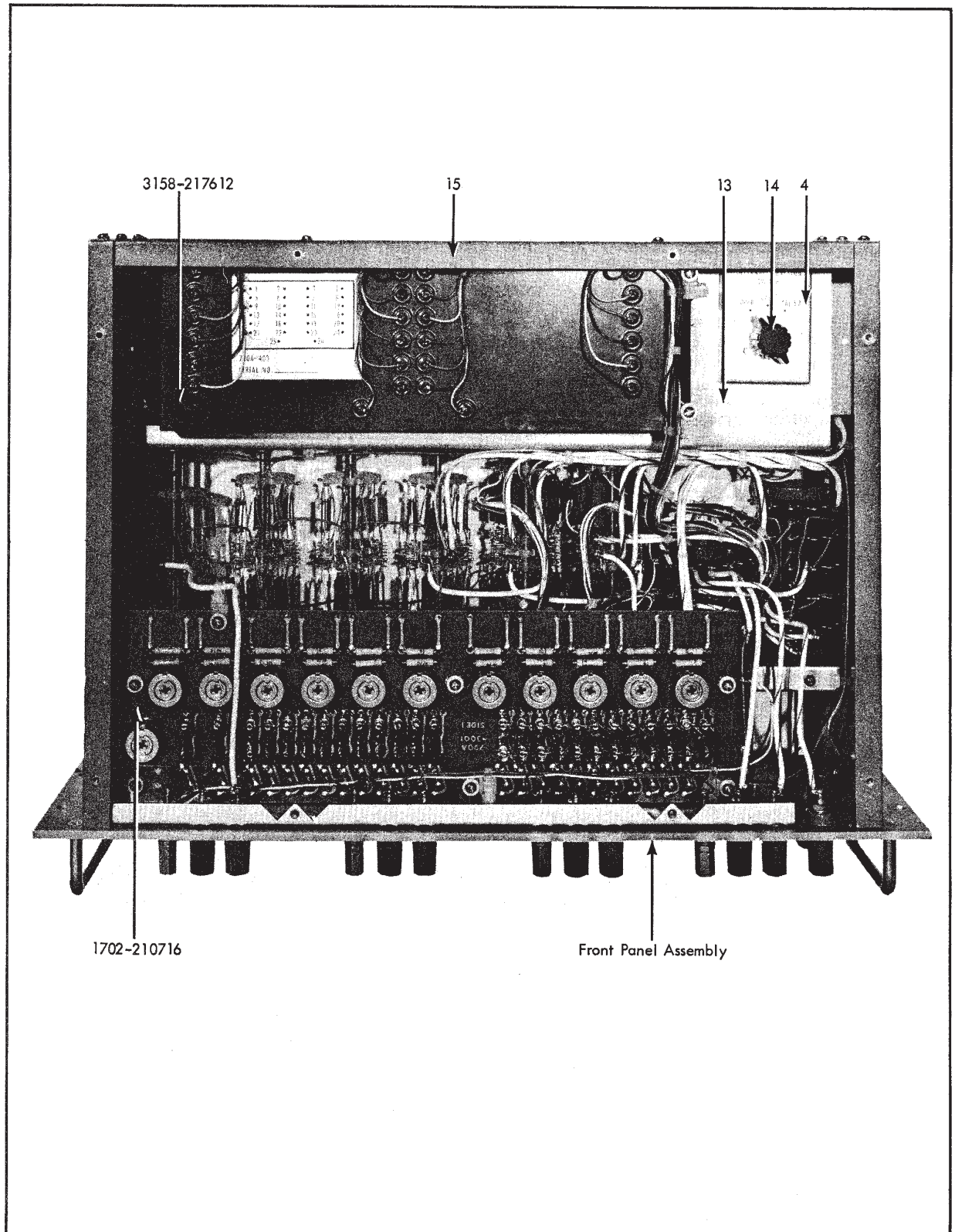
Figure 5-1. 720A KELVIN-VARLEY VOLTAGE DIVIDER (Sheet 2 of 2)
