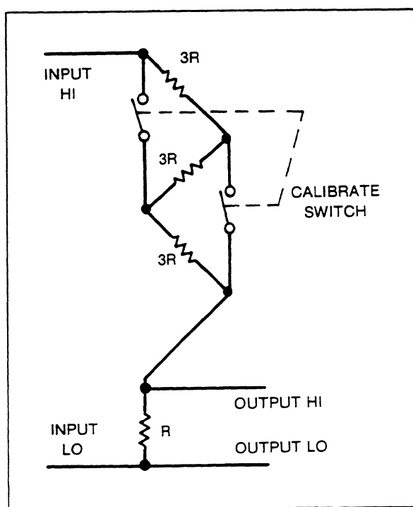
Figure 3-6. Calibrate Mode Switching (10:1)
