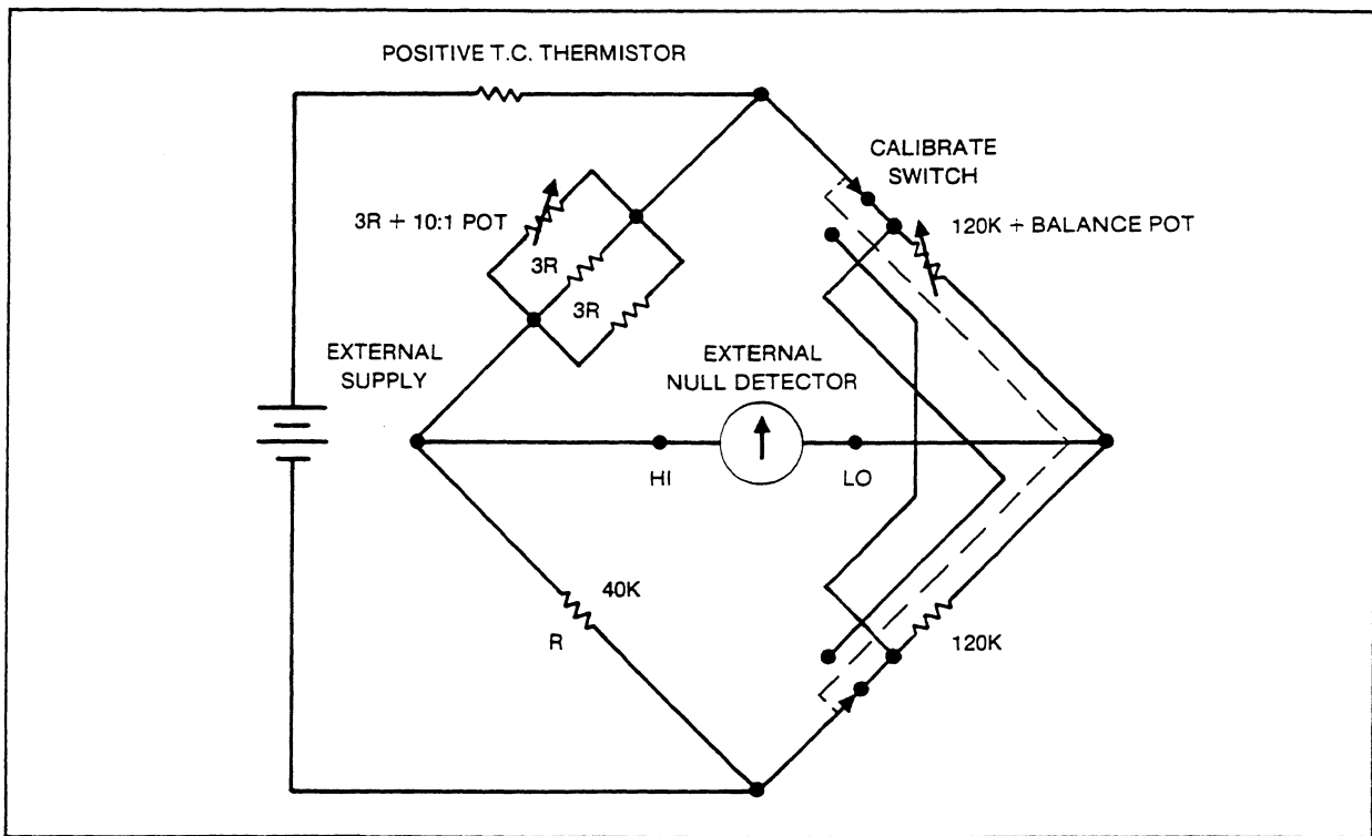
Figure 3-7. 10:1 Divider and Calibration Circuit
