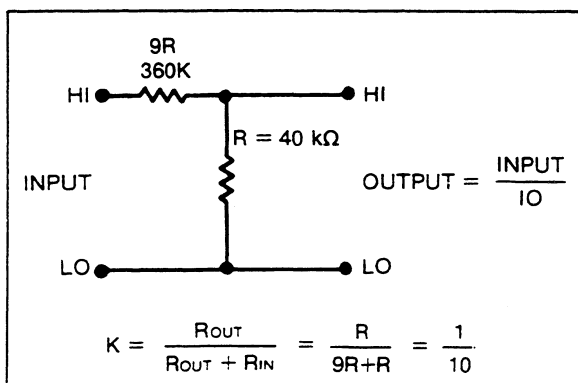
Figure 3-4. 10:1 Voltage Divider
