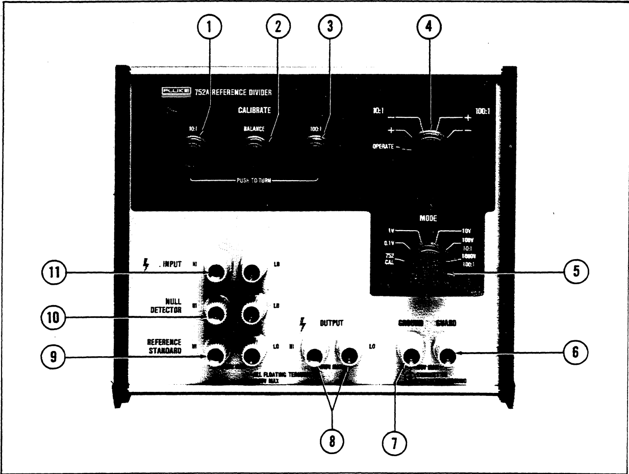
Figure 2-1. Front Panel Controls and Connectors
