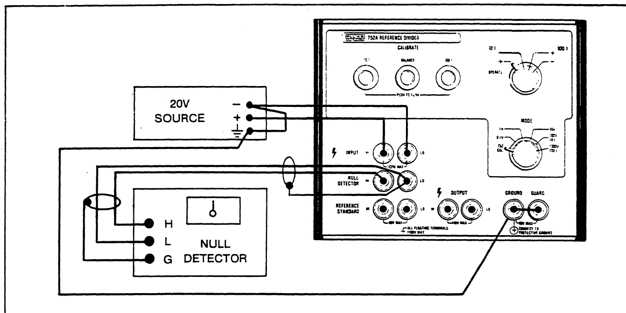
Figure 2-2. Self-Calibration Setup
