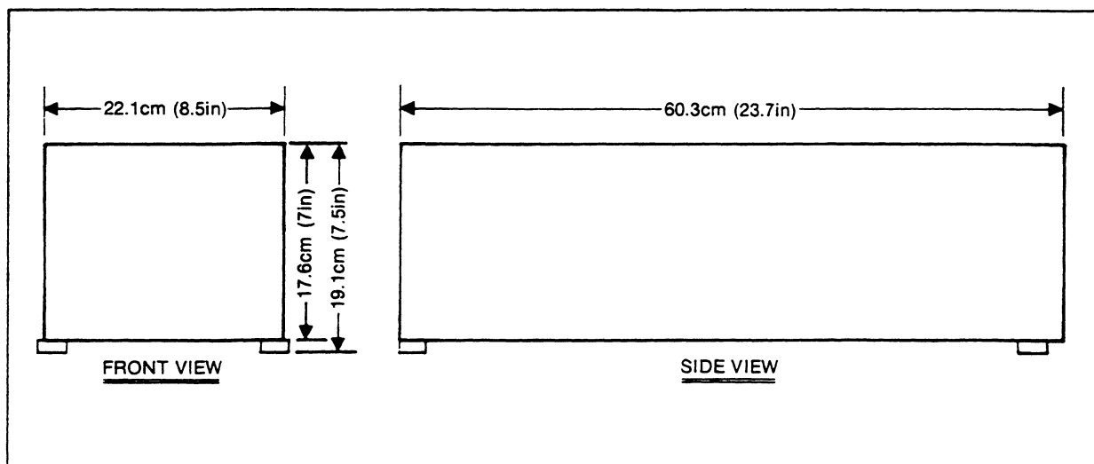
Figure 1-1. Model 752A External Dimensions
