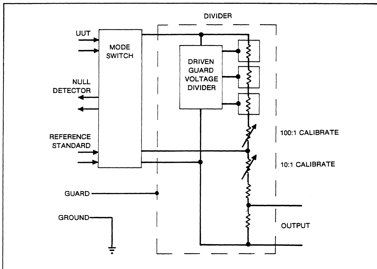
Figure 3-2. System Operation Block Diagram
