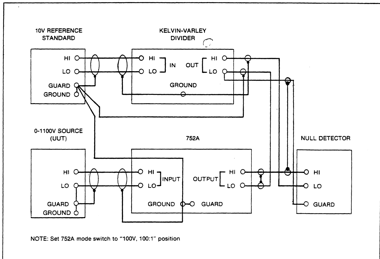
Figure 2-5. Stand-Alone Operation
