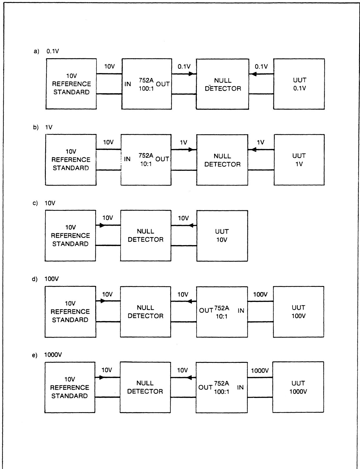
Figure 2-3. Mode Switch Configurations Block Diagram
