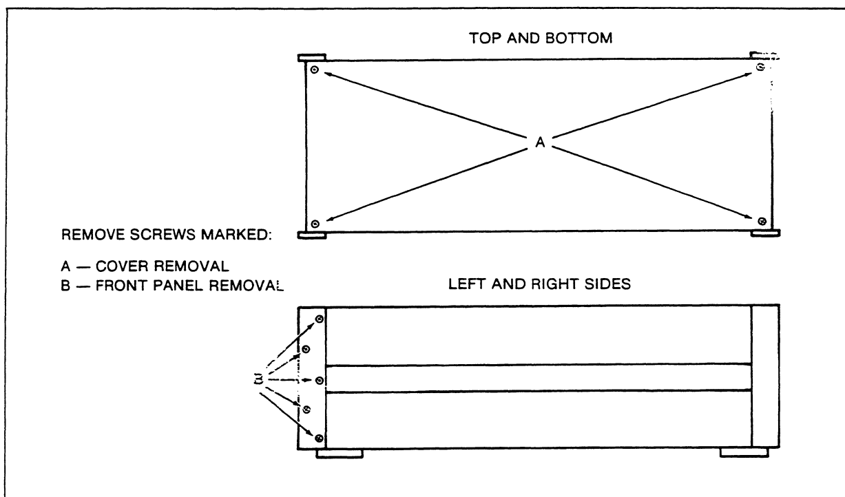
Figure 4-1. Cover Screw Locations
