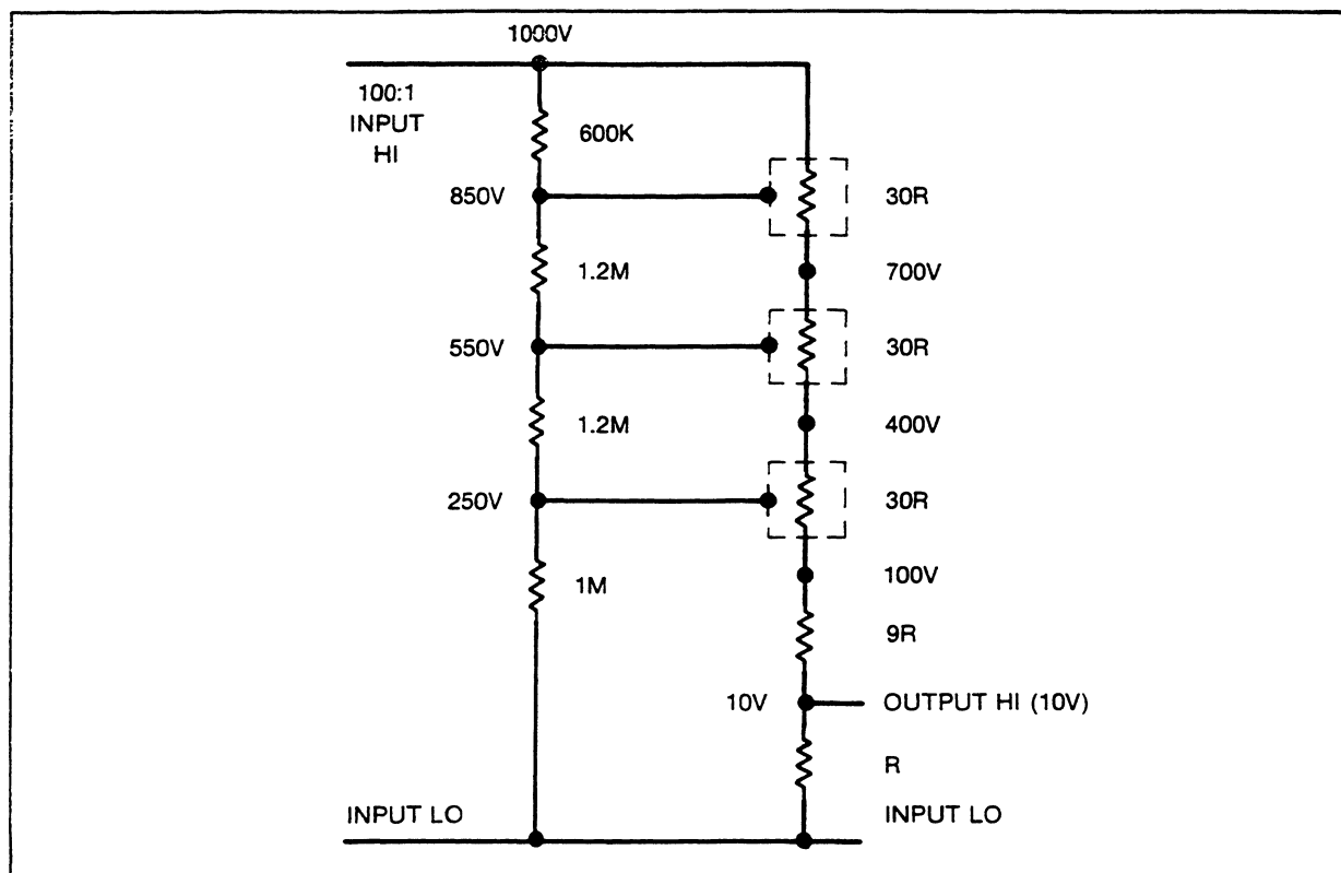
Figure 3-9. 100:1 Divider Driven Guard
