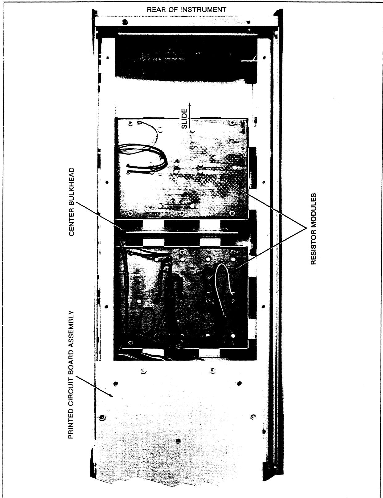
Figure 4-4. Resistor Module Access
