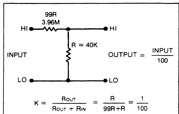
Figure 3-5. 100:1 Voltage Divider
