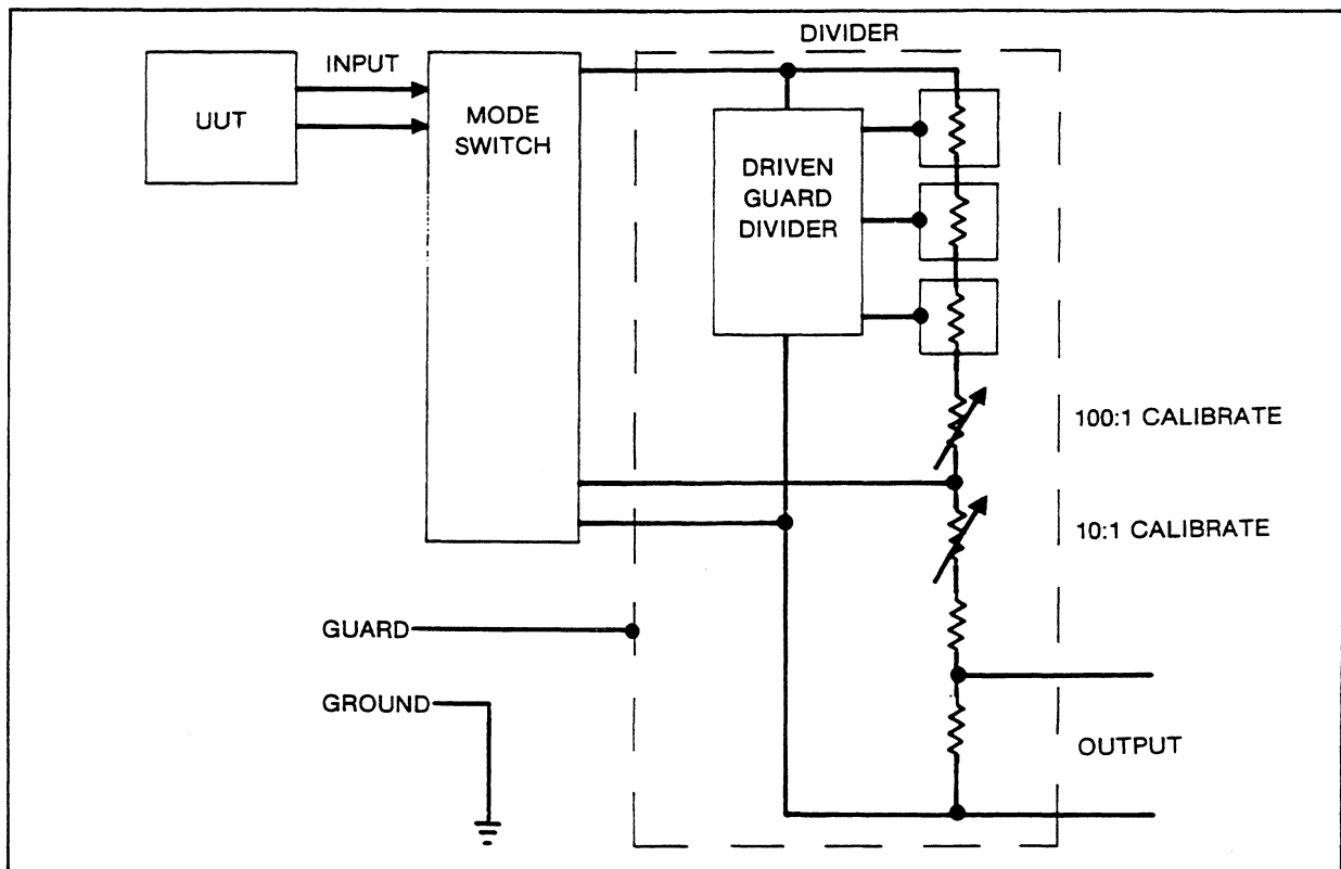
Figure 3-3. Stand-Alone Operation
