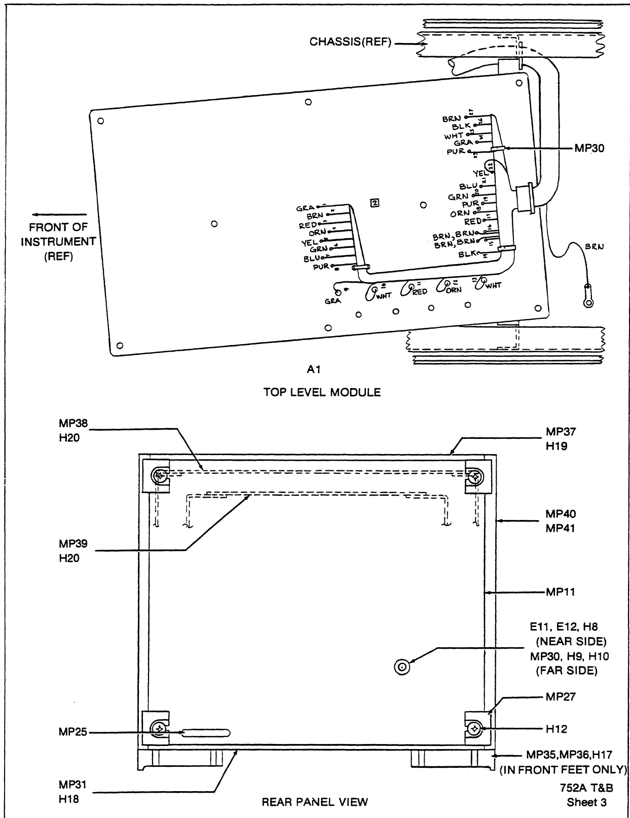
Figure 5-1. 752A Final Assembly (cont)
