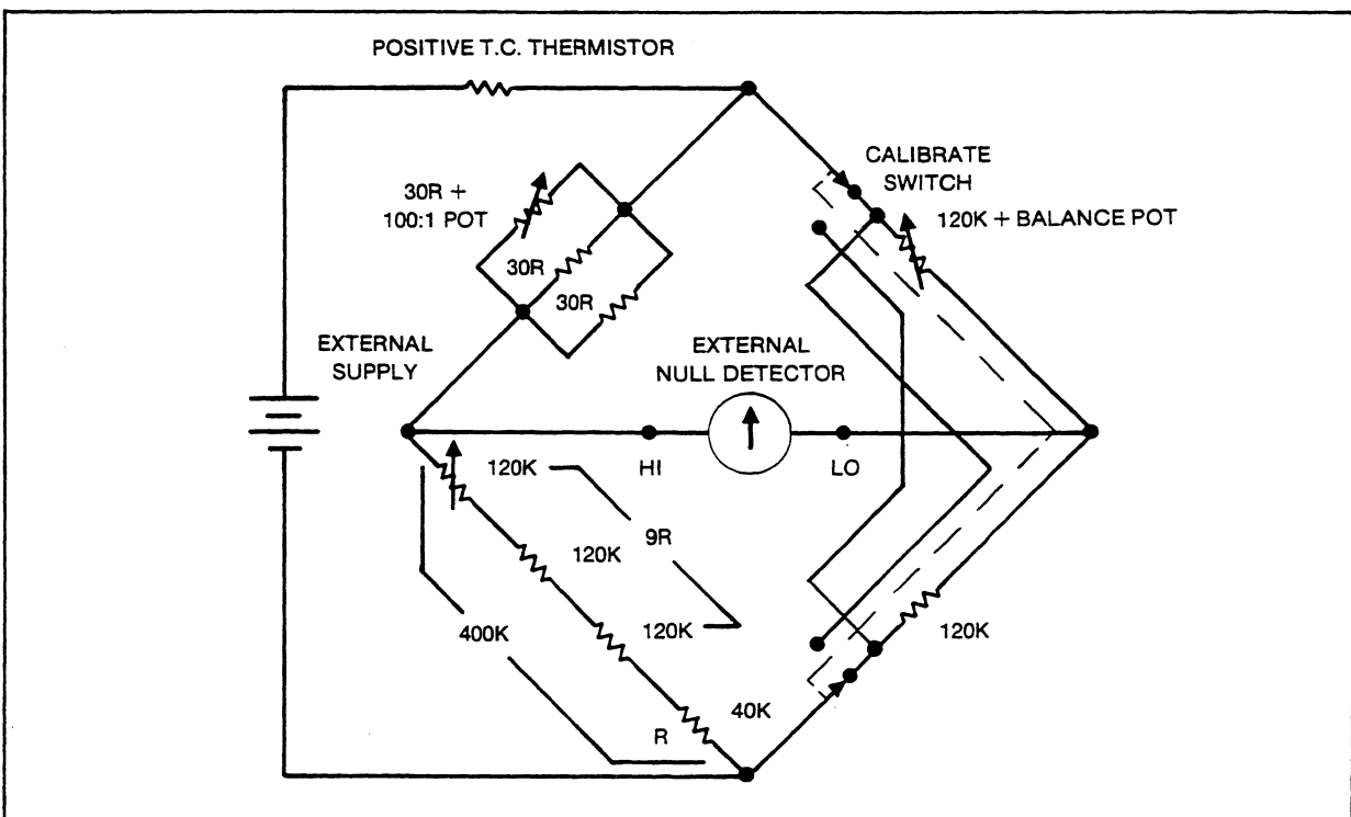
Figure 3-8. 100:1 Divider and Calibration Circuit
