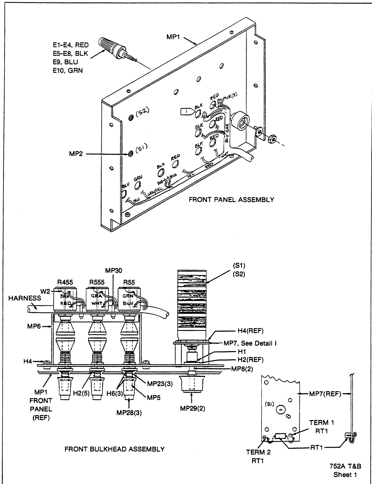
Figure 5-1. 752A Final Assembly
