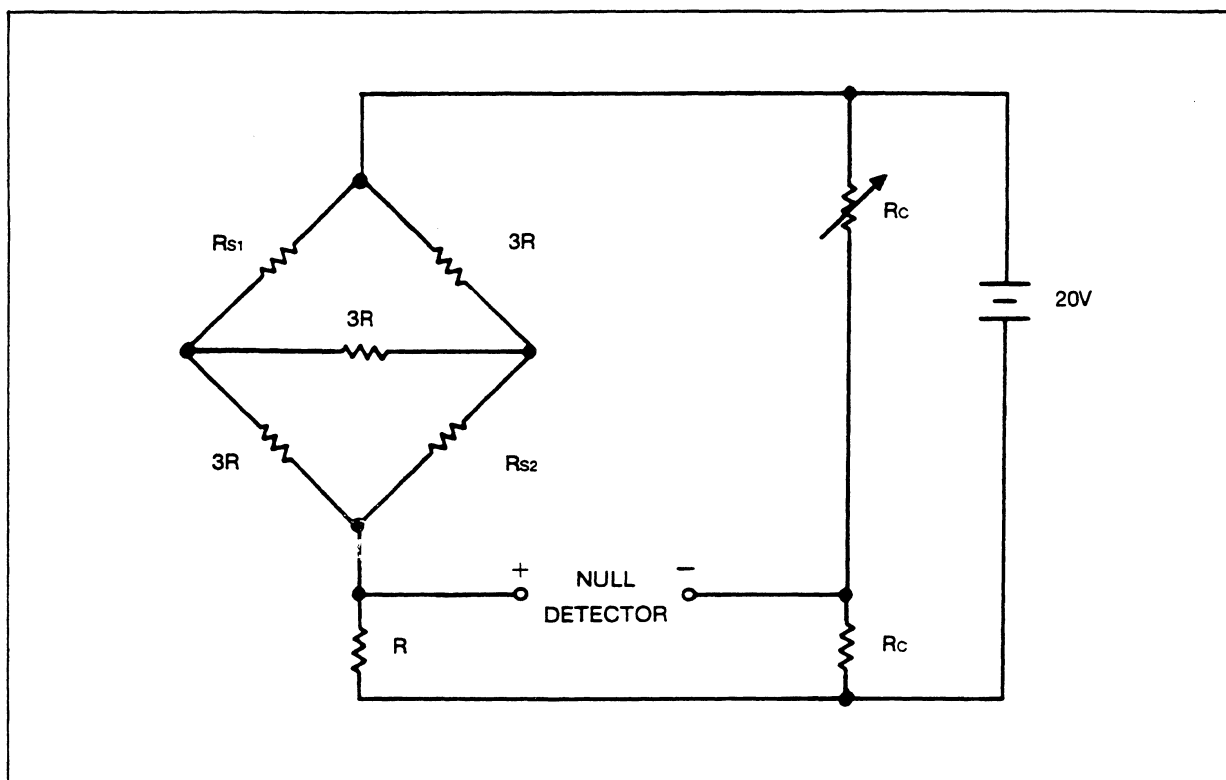
Figure 3-10. Simplified Schematic of 10:1 Calibration Circuit
