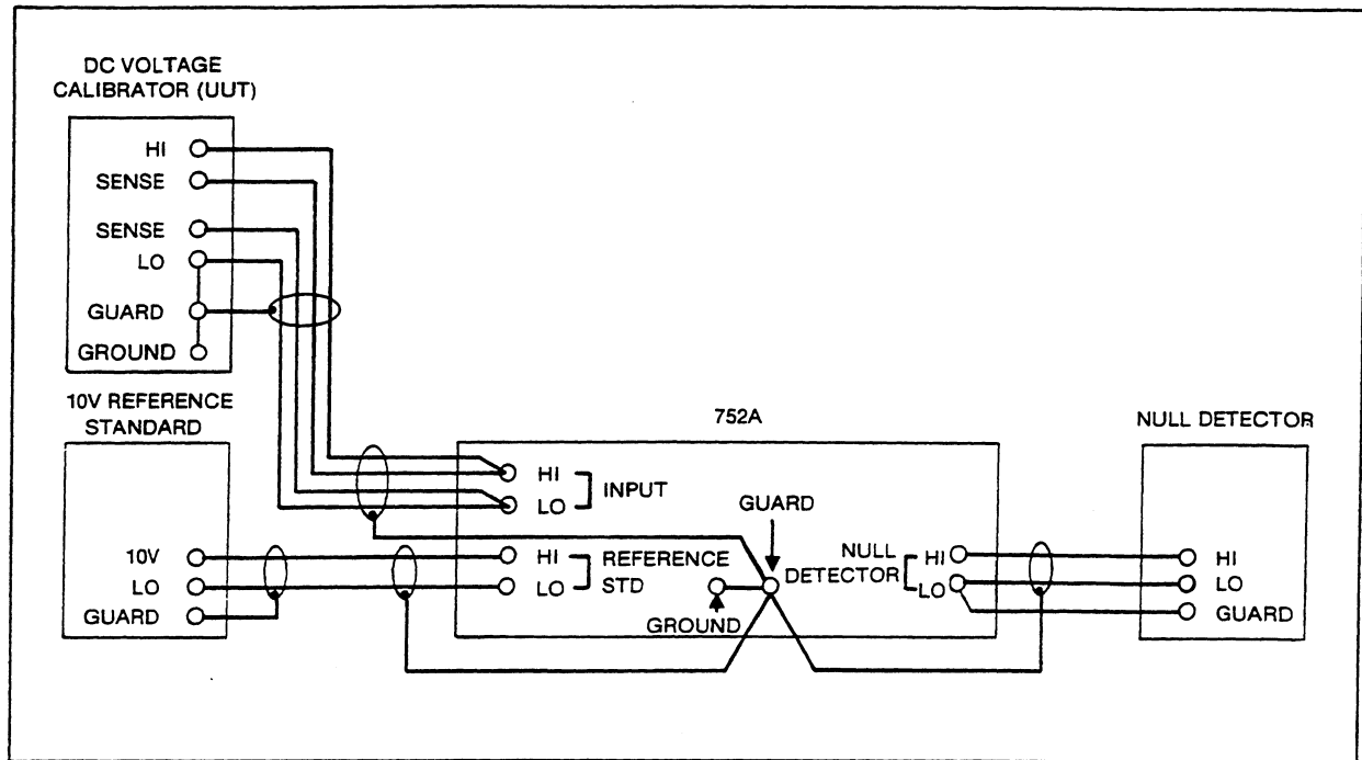
Figure 2-4. Calibration System Operation
