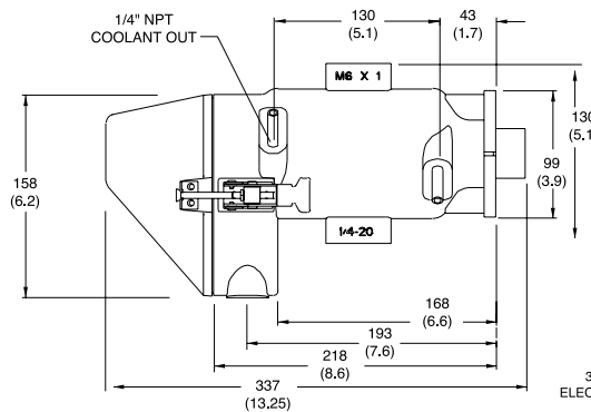
Modline 7 high temperature waterjacket
