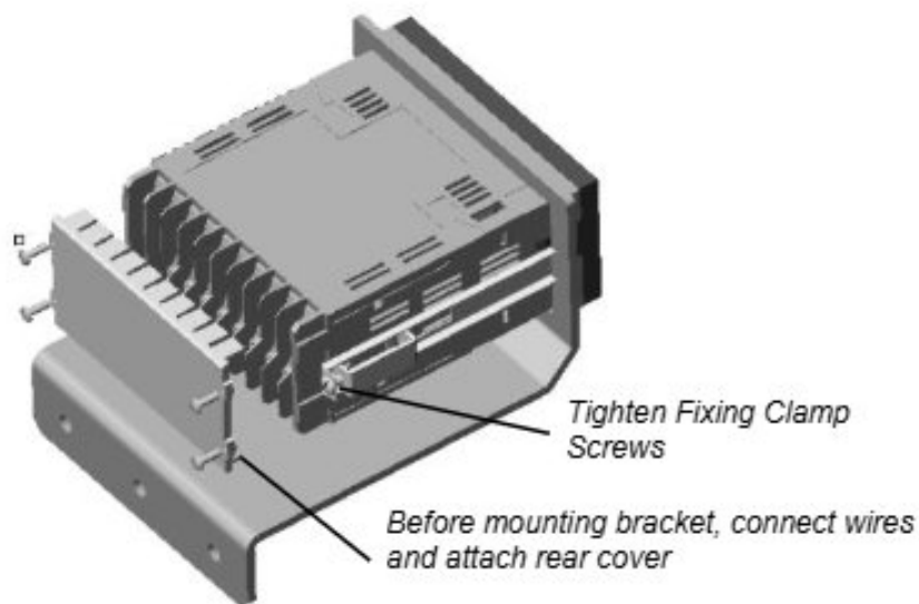
Figure 4: Completing the Installation
