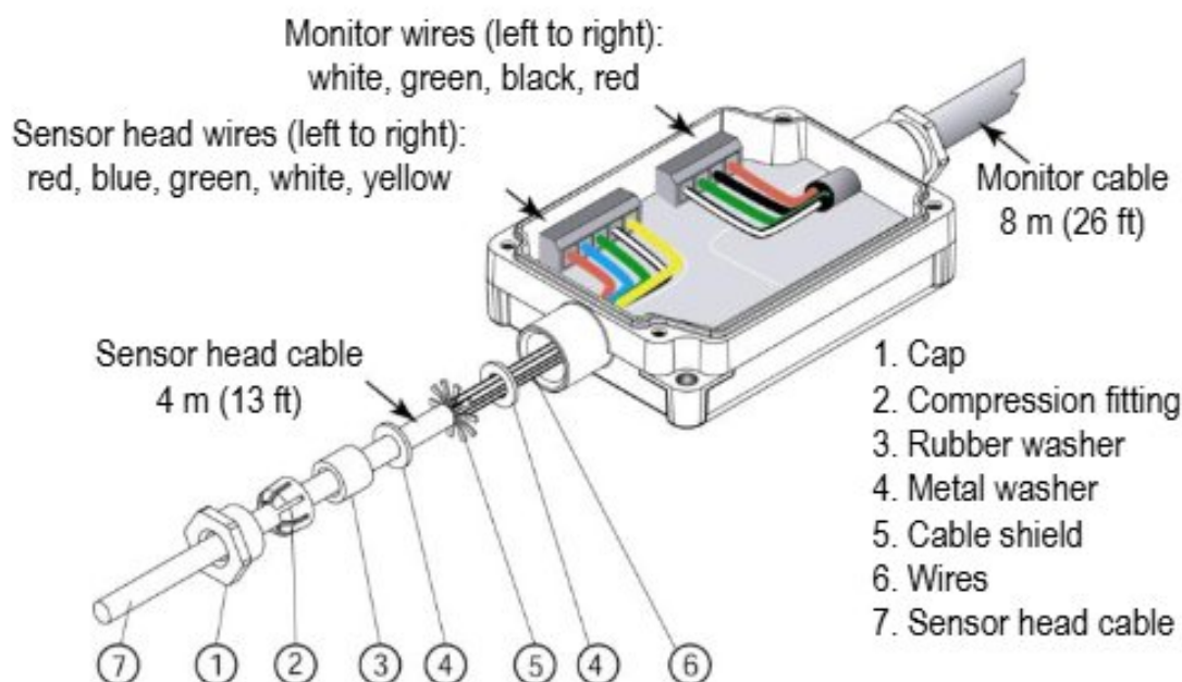
Figure 33: Laser Switching Box
