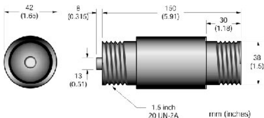
Figure 31: Dimensions for the GPS Head
