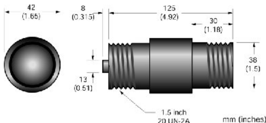
Figure 30: Dimensions for the GPR Head
