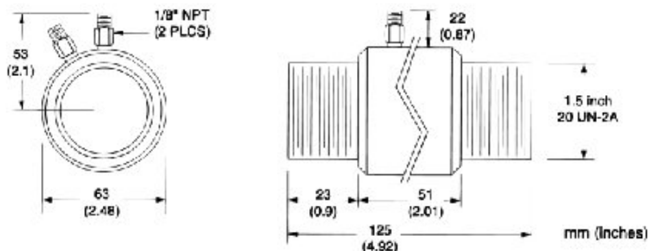
Figure 35: GPR Head with Air/Water-cooled Housing
