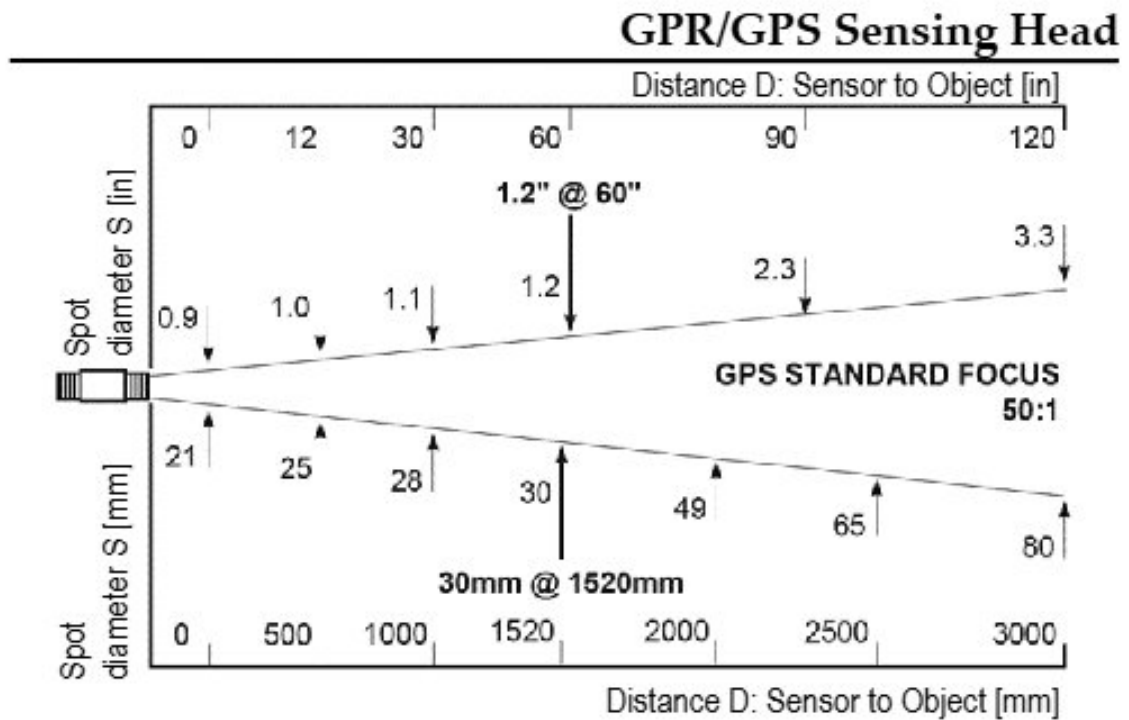
Figure 43: GPS Standard Focus Optics
