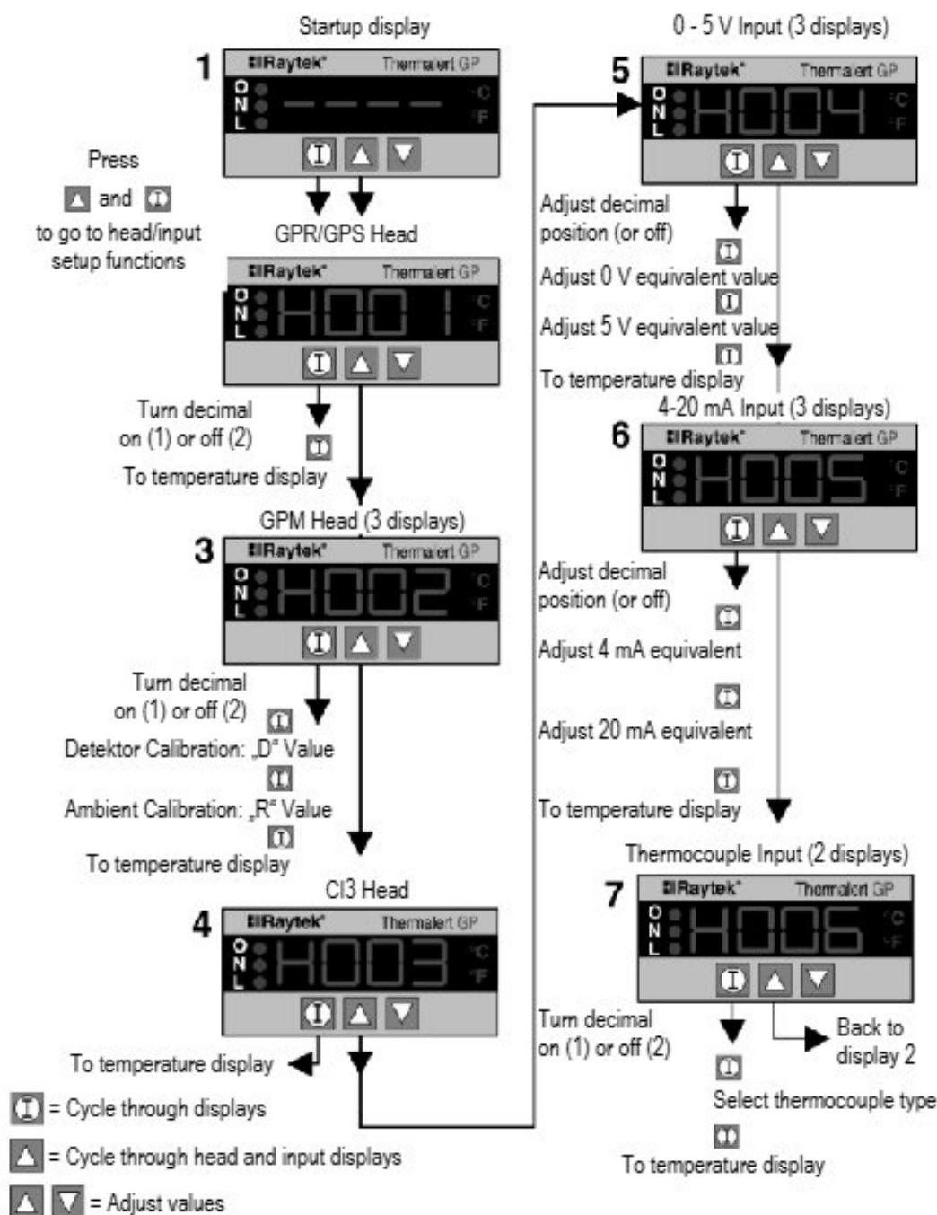
Figure 26: Head and Input Setup
