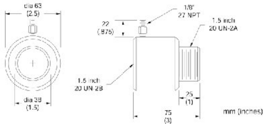
Figure 38: Air Purge Collar
