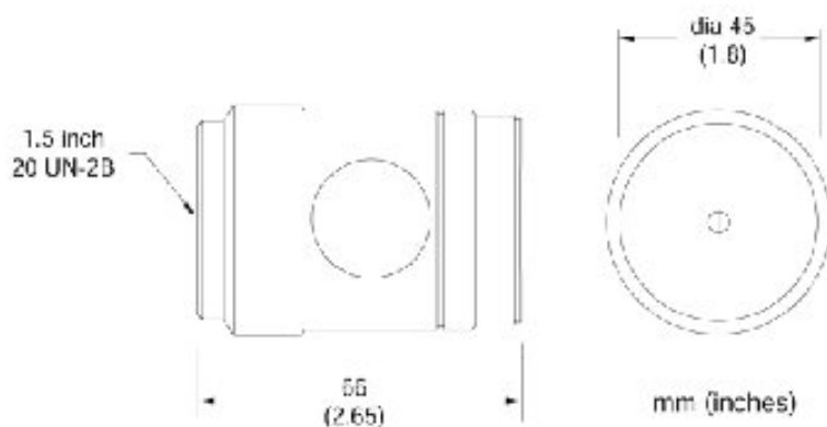
Figure 40: Sighting Viewer for GPR Head
