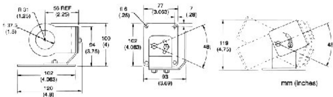
Figure 37: Adjustable Mounting Bracket
