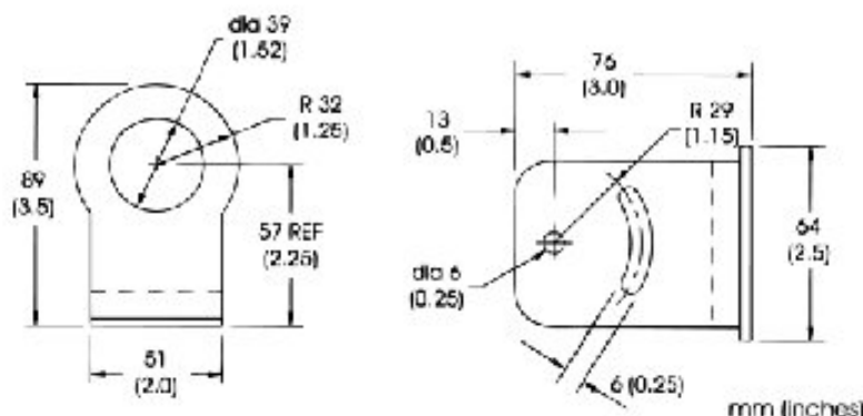
Figure 34: Fixed Mounting Bracket
