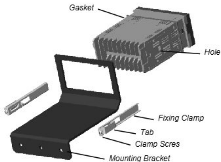
Figure 3: Mounting Bracket Accessory Installation
