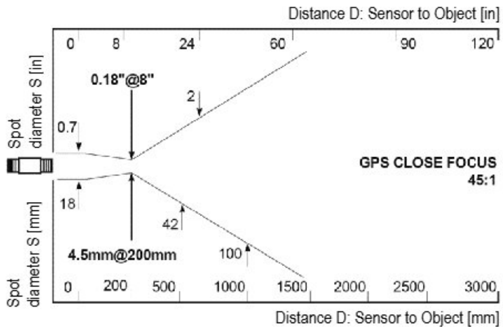
Figure 44: GPS Close Focus Optics
