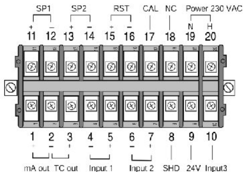
Figure 6: Terminal Block Layout
