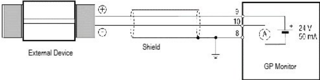
Figure 8: Installation 4 – 20 mA (2 Wires)
