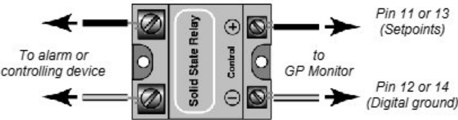
Figure 9: Relay Accessory Wiring
