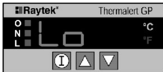
Figure 17: 4 mA Analog Output Display
