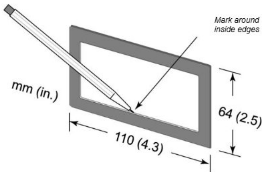
Figure 5: 1/8 DIN Cutout Template and Cosmetic Frame
