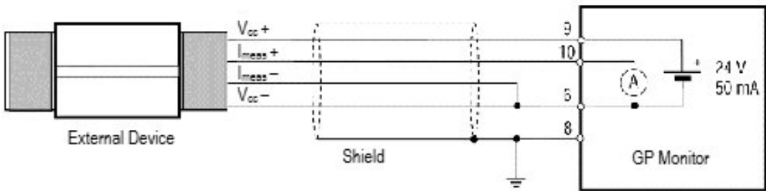
Figure 7: Installation 4 – 20 mA (4 Wires)
