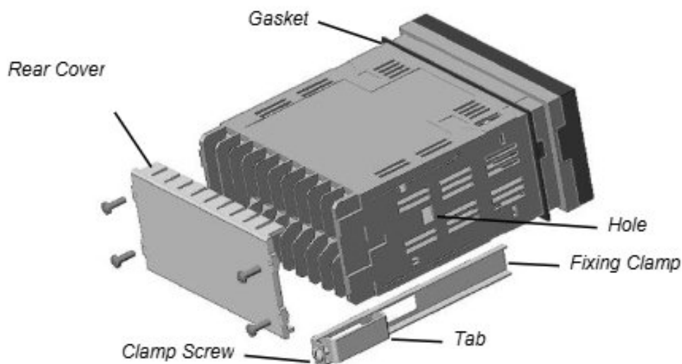
Figure 2: Mounting the Monitor
