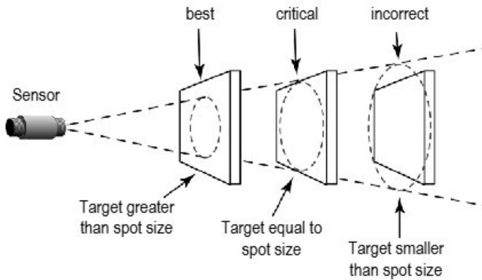
Figure 29: Proper Sensor Placement
