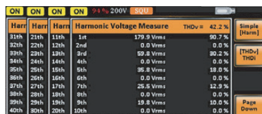
Voltage Harmonic
