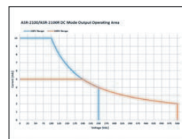
DC Output for ASR-2100/ASR-2100R
