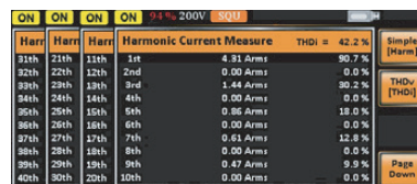
Current Harmonic
