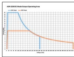
DC Output for ASR-3200
