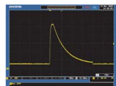
SEQ9: Load Dump with Tr_10ms, Td_40ms
