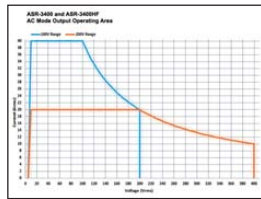
AC Output for ASR-3400/3400HF
