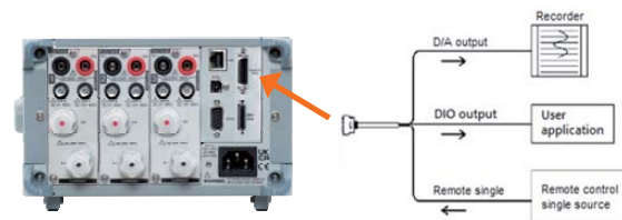
DA12 Interface Mechanism
