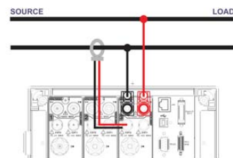
External Current Sensor Input
