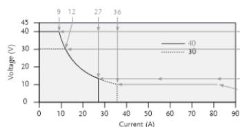
PSW 30V/40V Series Operating Area
