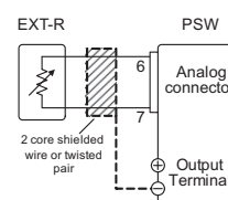
External Resistance control of the Voltage Output
