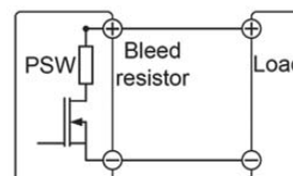
PSW-Multi Series Built-in Bleed Resistor
