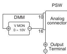
External DMM Monitoring of the Output Voltage
