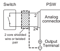
External Switch Control of the Output On/Off
