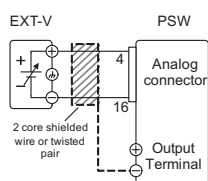
External Voltage Control of the Voltage Output
