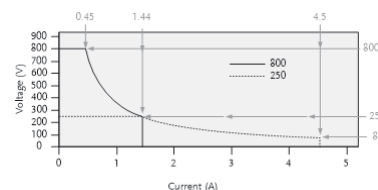
PSW 250V/800V Series Operating Area
