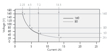
PSW 80V/160V Series Operating Area
