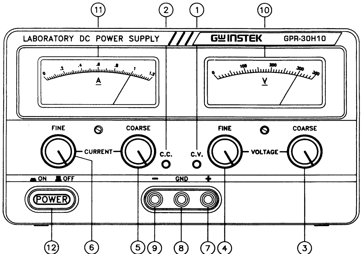
Fig. 4-2 Front Panel (Analog Type)
