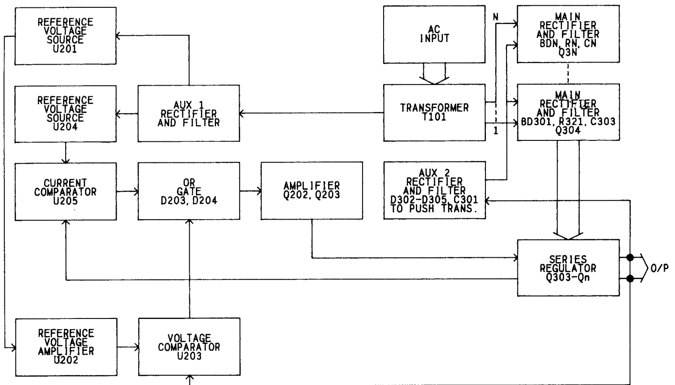
Fig. 2 Block Diagram (More than 100V)
