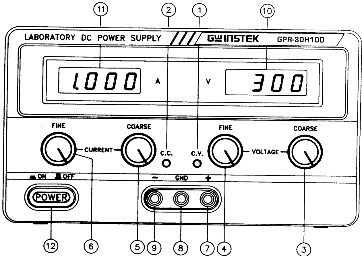
Fig. 4-1 Front Panel (Digital Type)
