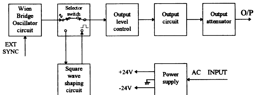
Fig.1 Block Diagram
