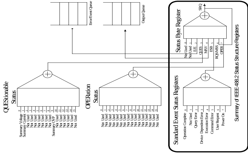
Figure 7. A graphic representation of the status registers and their connections.
