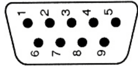
Figure 1 Pin assignments of the RS232 connector on the rear panel for DB-9-D
