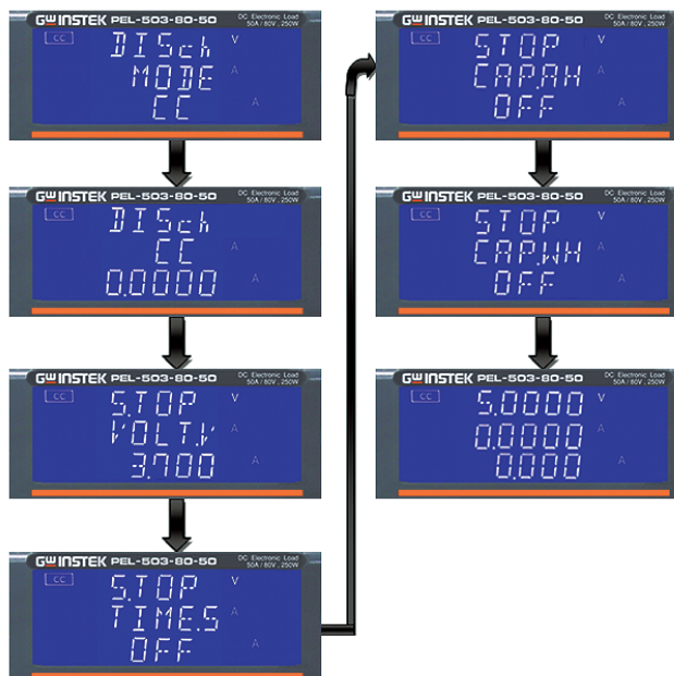
Battery Discharge Setting Processes
