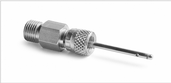
QTHA-PMS0-0.125-1.5
