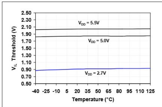
FIGURE 2-18: V_{IN} Low Threshold vs. Temperature and V_{DD} .
