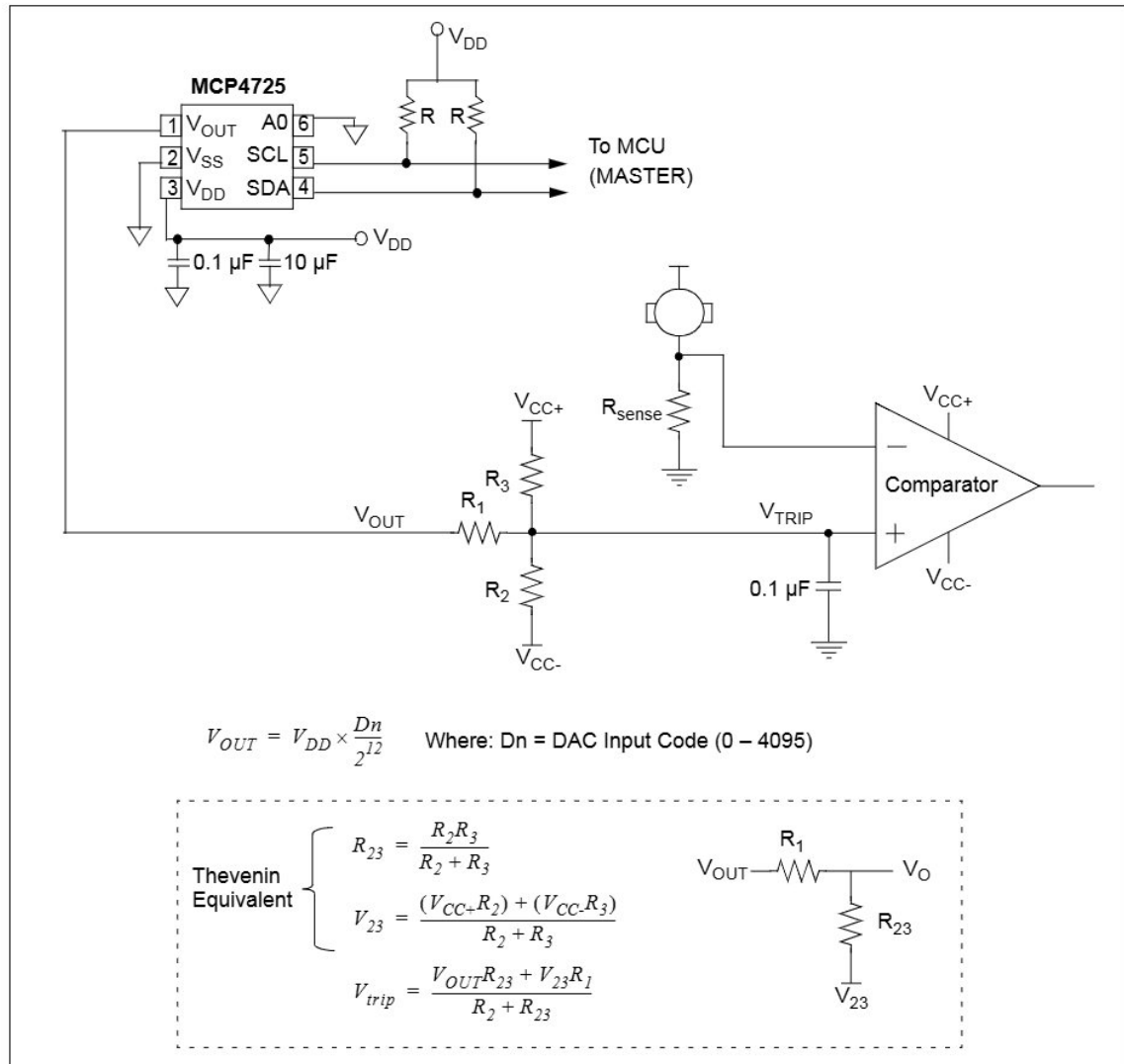
EXAMPLE 8-2: Single-Supply "Window" DAC.
