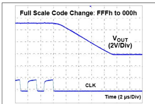
FIGURE 2-20: Full Scale Settling Time.
