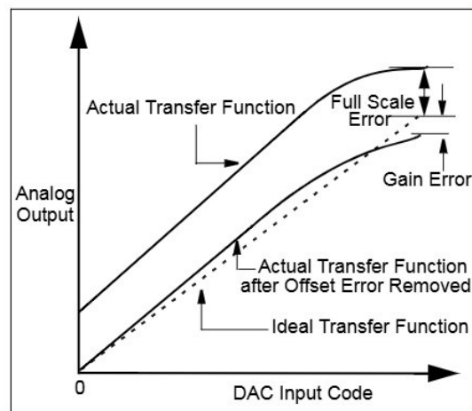
FIGURE 4-4: Gain Error and Full Scale Error.
