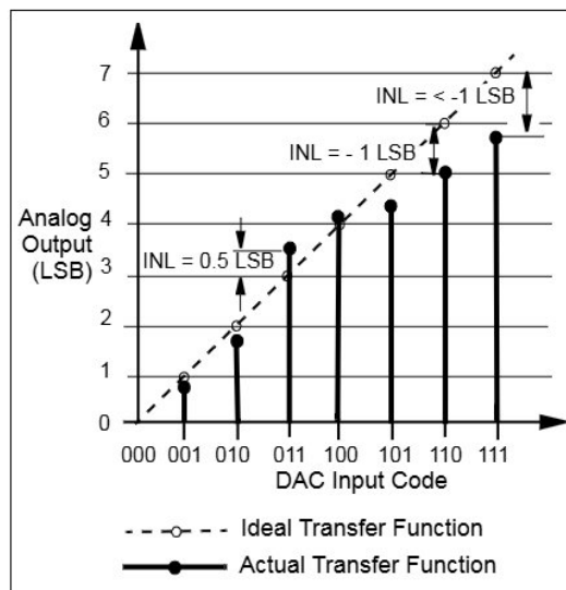
FIGURE 4-1: INL Accuracy.
