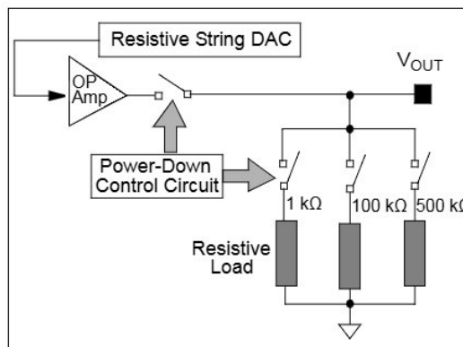
FIGURE 5-1: Output Stage for Power-Down Mode.
