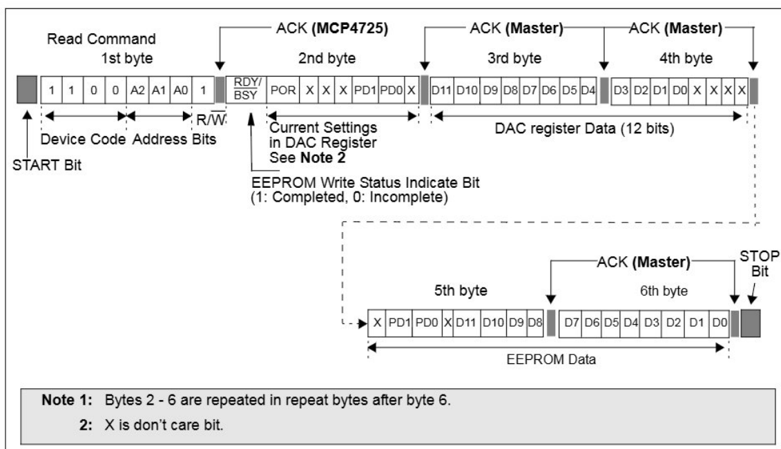
FIGURE 6-3: Read Command and Output Data Format.
