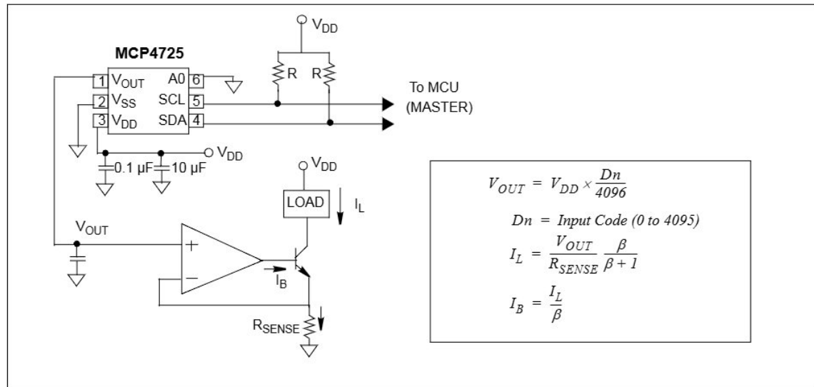
FIGURE 8-3: Digitally Controllable Current Source.
