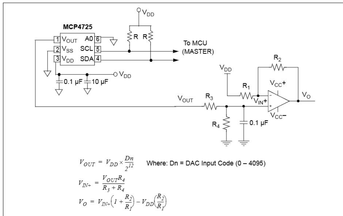
EXAMPLE 8-3: Digitally-Controlled Bipolar Voltage Source.
