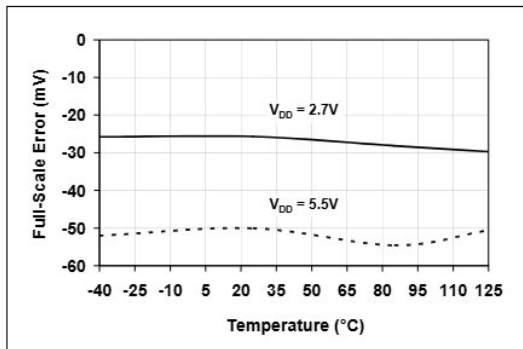
FIGURE 2-9: Full Scale Error vs. Temperature (Code = 4095d).
