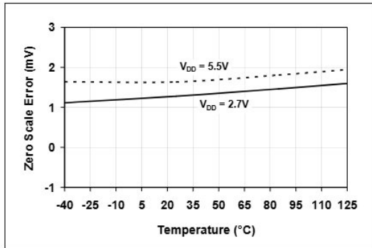
FIGURE 2-8: Zero Scale Error vs. Temperature (Code = 000d).
