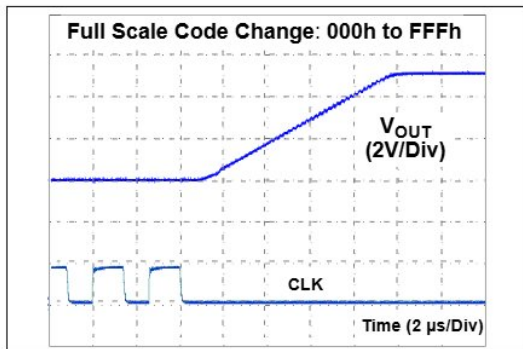
FIGURE 2-19: Full Scale Settling Time.
