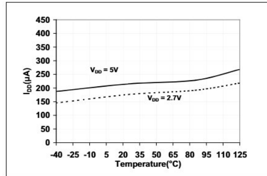
FIGURE 2-11: I_{DD} vs. Temperature.
