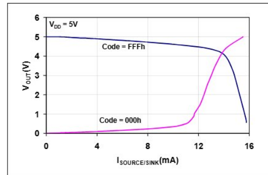
FIGURE 2-16: Source and Sink Current Capability.
