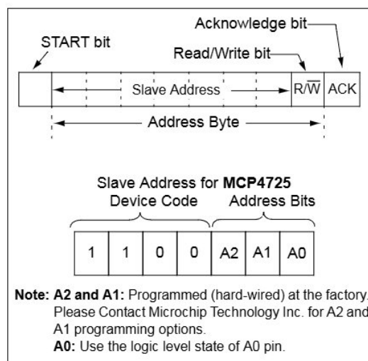
FIGURE 7-1: Device Addressing.
