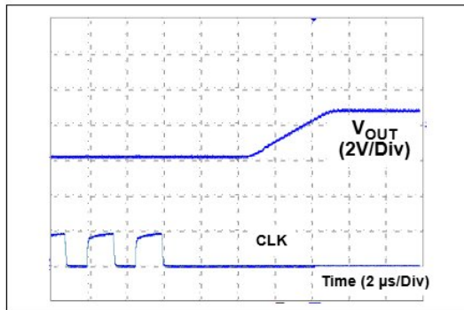
FIGURE 2-24: Exiting Power Down Mode.
