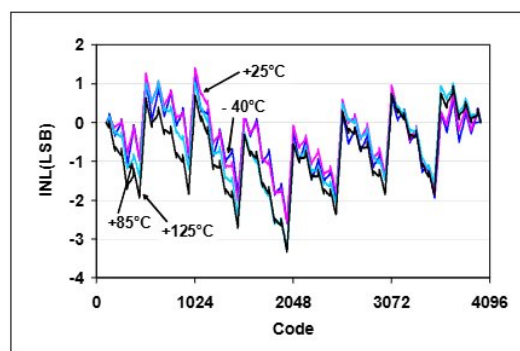
FIGURE 2-6: INL vs. Code and Temperature ( V_{DD} = 5.5\text{V} ).
