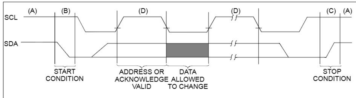
FIGURE 7-3: Data Transfer Sequence On The Serial Bus.
