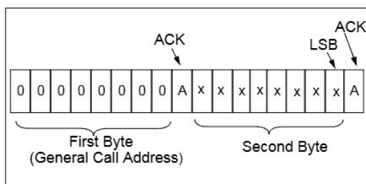
FIGURE 7-2: General Call Address Format.
