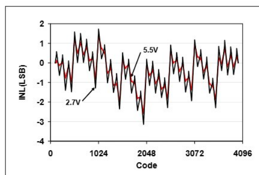
FIGURE 2-5: INL vs. Code.
