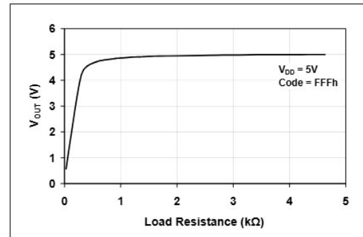
FIGURE 2-15: V_{OUT} vs. Resistive Load.
