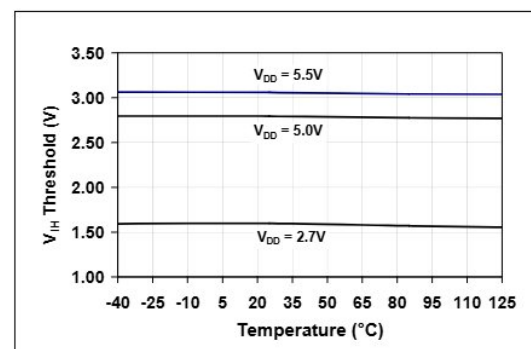
FIGURE 2-17: V_{IN} High Threshold vs. Temperature and V_{DD} .
