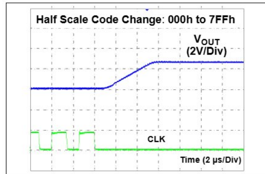
FIGURE 2-21: Half Scale Settling Time.
