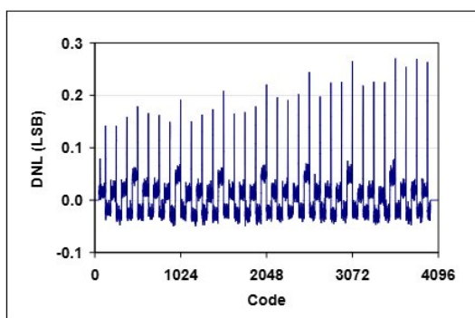
FIGURE 2-3: DNL vs. Code ( V_{DD} = 2.7\text{V} ).
