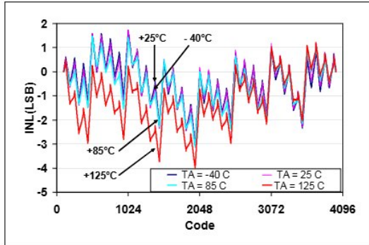
FIGURE 2-7: INL vs. Code and Temperature ( V_{DD} = 2.7\text{V} ).
