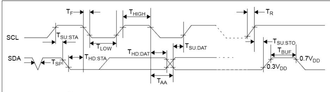
FIGURE 7-4: I 2 C Bus Timing Data.
