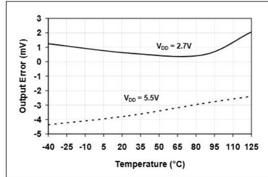
FIGURE 2-10: Output Error vs. Temperature (Code = 4000d).
