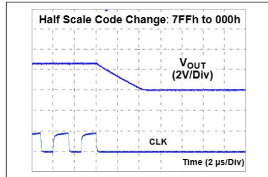
FIGURE 2-22: Half Scale Settling Time.
