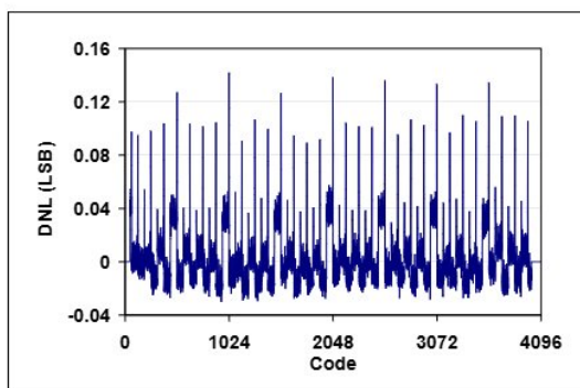
FIGURE 2-1: DNL vs. Code ( V_{DD} = 5.5\text{V} ).
