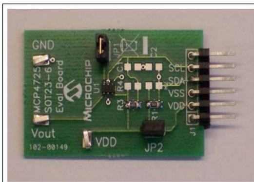
FIGURE 9-1: MCP4725 SOT-23-6 Evaluation Board.
