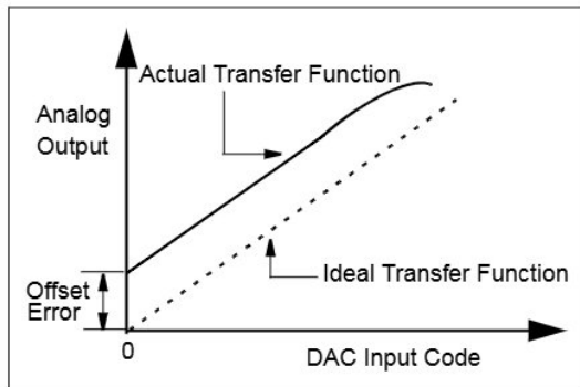
FIGURE 4-3: Offset Error.
