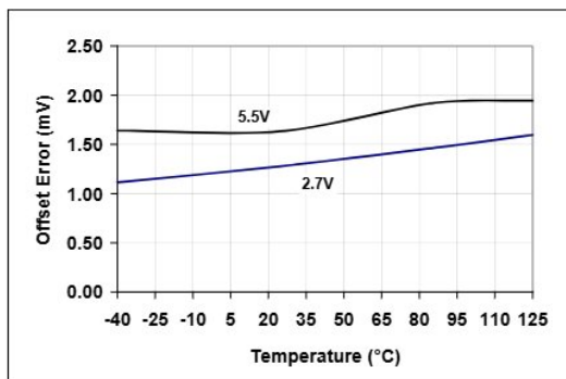
FIGURE 2-14: Offset Error vs. Temperature and V_{DD} .
