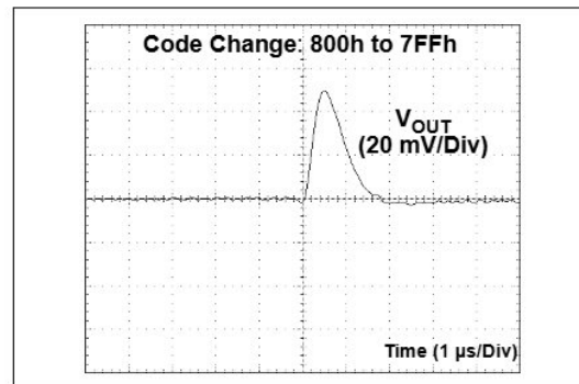
FIGURE 2-23: Code Change Glitch.
