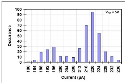
FIGURE 2-12: I_{DD} Histogram.
