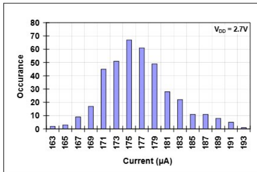
FIGURE 2-13: I_{DD} Histogram.
