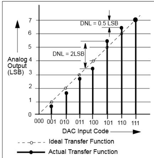
FIGURE 4-2: DNL Accuracy.
