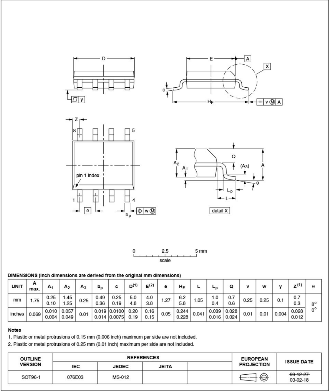
Fig 16. Package outline SOT96-1 (SO8)
