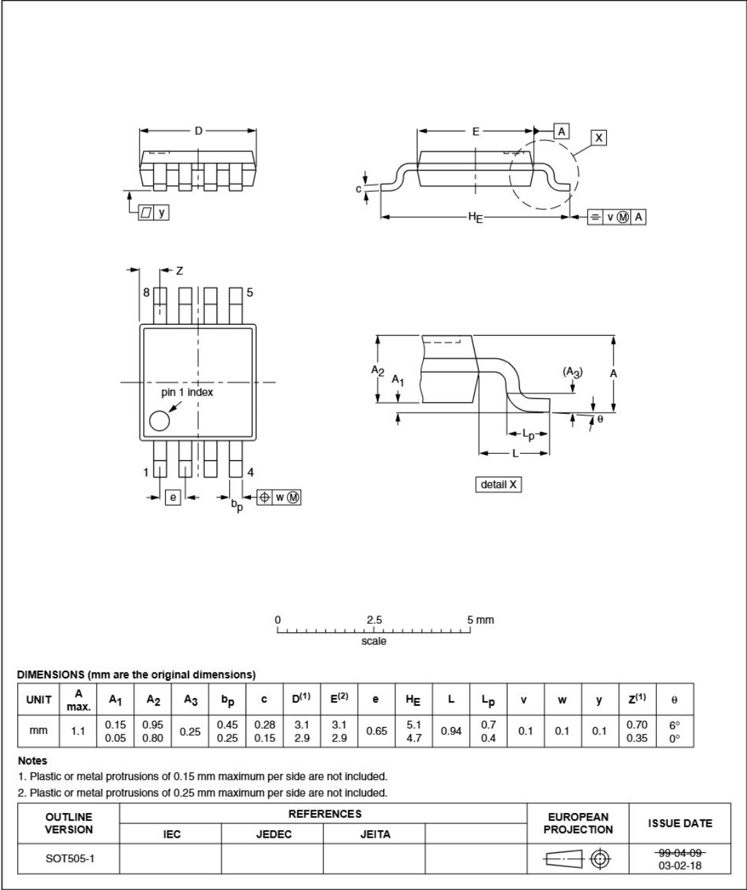
Fig 17. Package outline SOT505-1 (TSSOP8)
