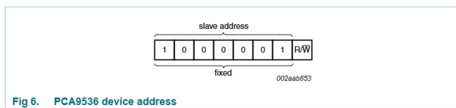
Fig 6. PCA9536 device address
