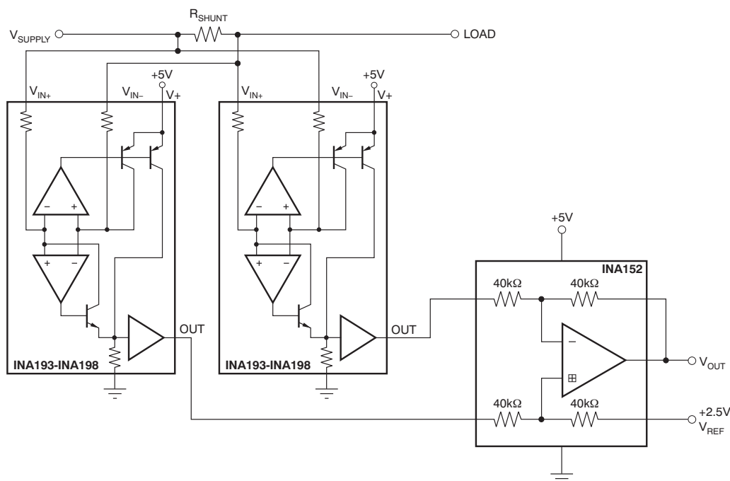
Figure 29. Bi-Directional Current Monitoring
