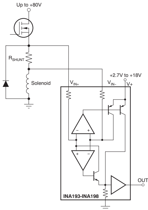
Figure 23. Inductive Current Monitor Including Flyback
