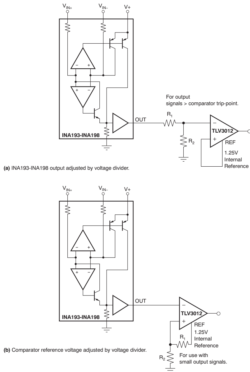
Figure 24. INA193-INA198 with Comparator
