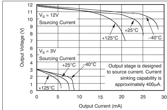
Figure 7. Positive Output Voltage Swing vs Output Current
