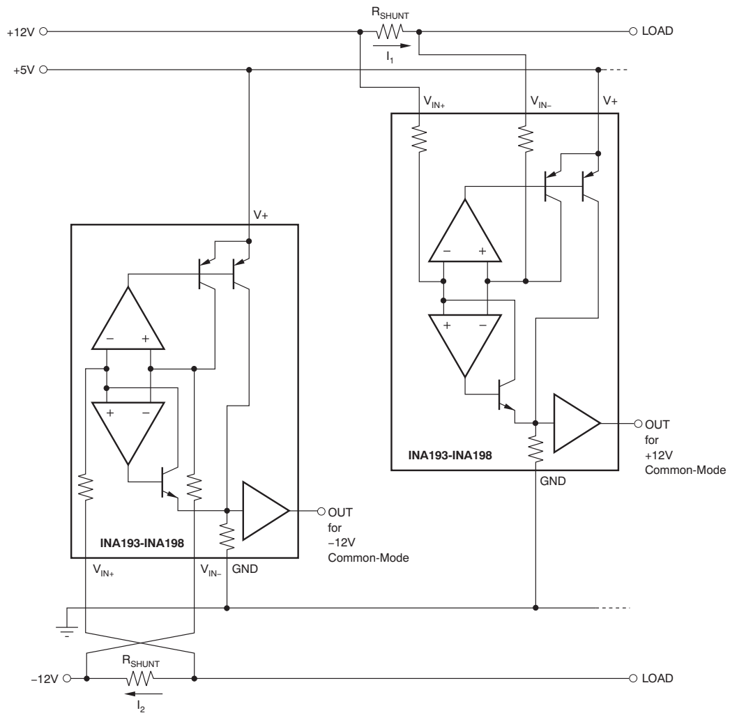
Figure 22. Monitor Bipolar Output Power-Supply Current
