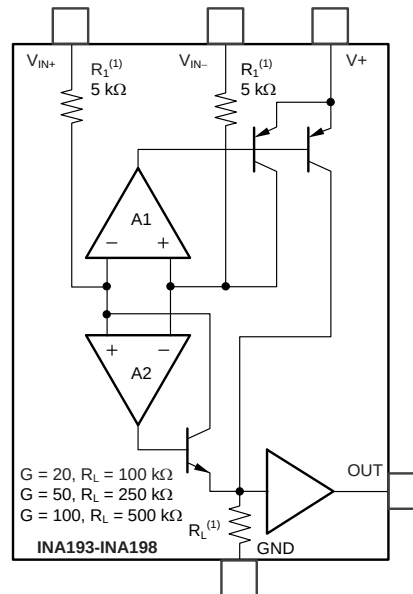
Figure 21. INA193-INA198 Simplified Circuit Diagram
