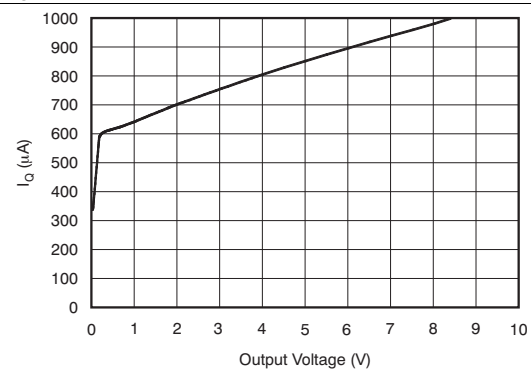
Figure 8. Quiescent Current vs Output Voltage
