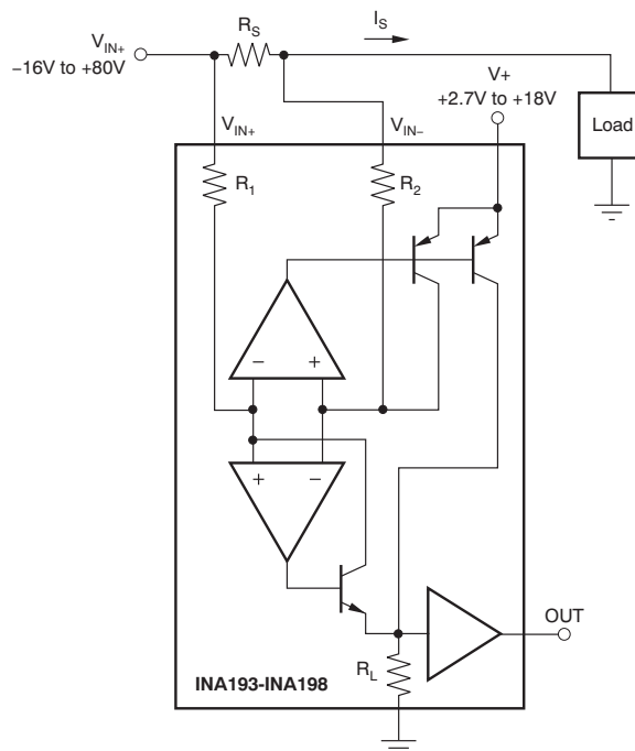
Figure 20. INA193-INA198 Basic Connection
