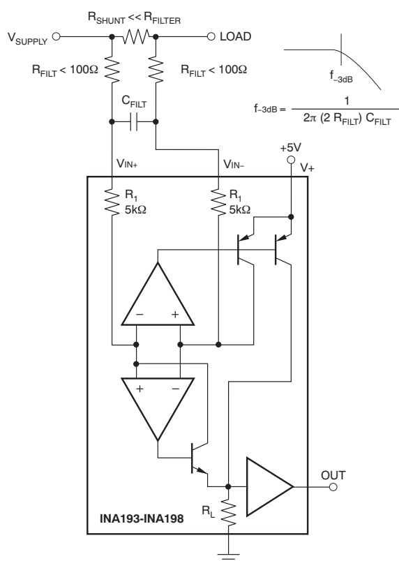
Figure 25. Input Filter (Gain Error – 1.5% To –2.2%)
