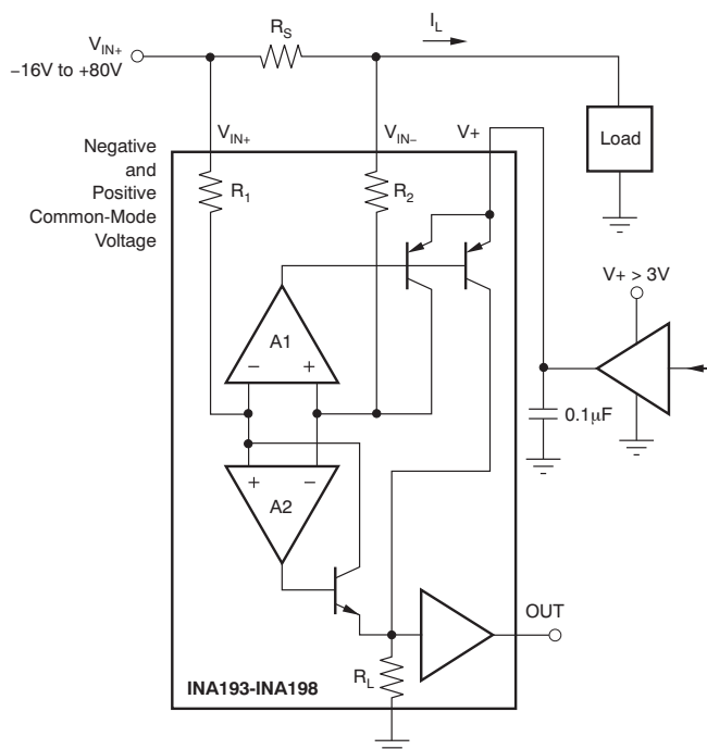
Figure 28. INA193-INA198 Example Shutdown Circuit
