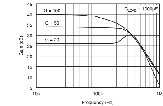
Figure 1. Gain vs Frequency
