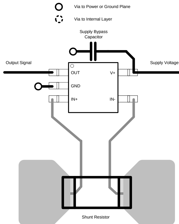
Figure 31. Recommended Layout
