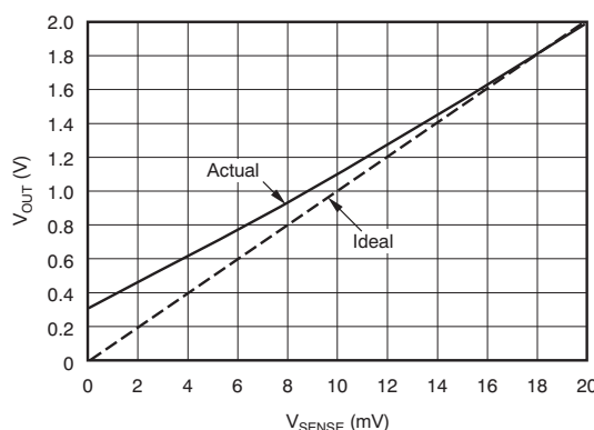
Figure 26. Example for Low V_{SENSE} Cases 1 and 3 (INA195, INA198: Gain = 100)
