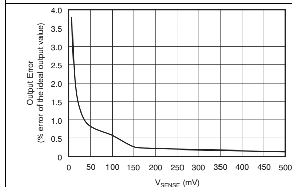
Figure 5. Output Error vs V_{SENSE}
