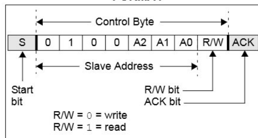
FIGURE 1-2: I 2 C™ CONTROL BYTE FORMAT
