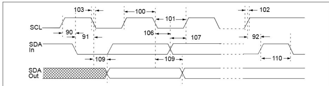
FIGURE 2-4: I 2 C™ BUS DATA TIMING
