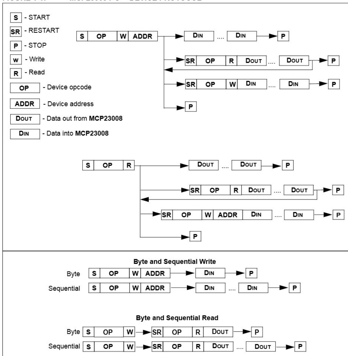
FIGURE 1-1: MCP23008 I 2 C™ DEVICE PROTOCOL
