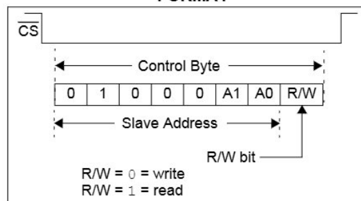
FIGURE 1-3: SPI CONTROL BYTE FORMAT
