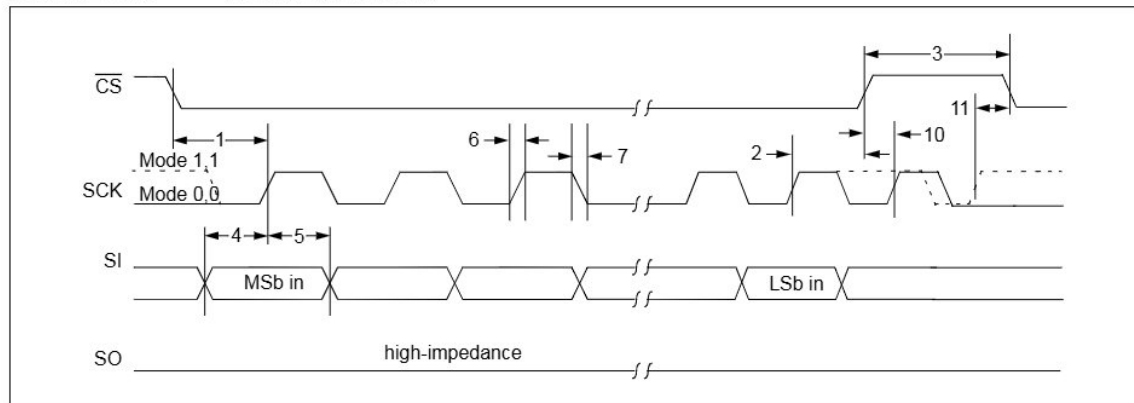
FIGURE 2-5: SPI INPUT TIMING
