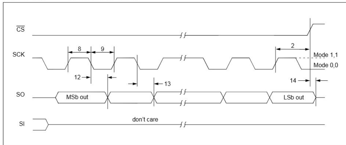
FIGURE 2-6: SPI OUTPUT TIMING
