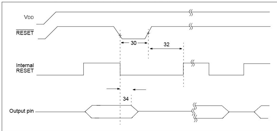
FIGURE 2-2: RESET AND DEVICE RESET TIMER TIMING
