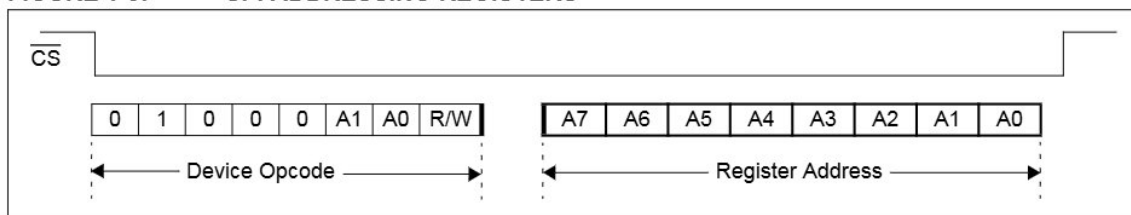
FIGURE 1-5: SPI ADDRESSING REGISTERS
