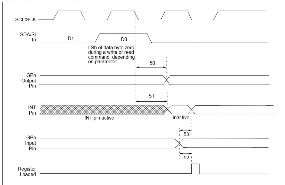
FIGURE 2-7: GPIO AND INT TIMING
