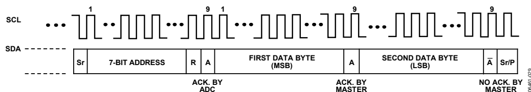
Figure 28. Mode of Operation, Single-Channel Conversion
