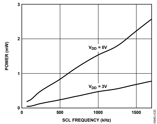
Figure 17. Power vs. SCL Frequency, V_{\text{REF}} = 2.5\text{V}
