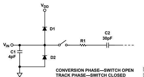
Figure 21. Equivalent Analog Input Circuit
