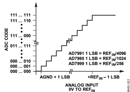
Figure 20. AD7991/AD7995/AD7999 Transfer Characteristics
