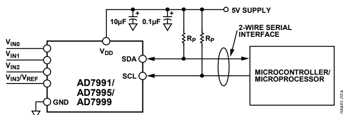
Figure 22. AD7991/AD7995/AD7999 Typical Connection Diagram
