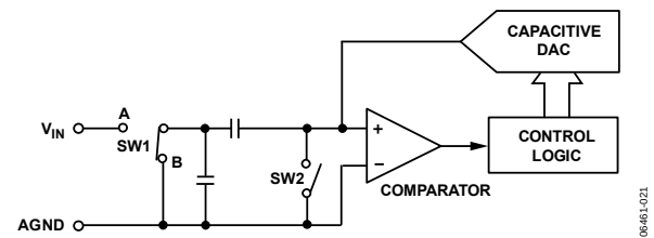
Figure 19. ADC Conversion Phase
