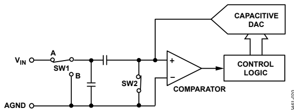
Figure 18. ADC Acquisition Phase
