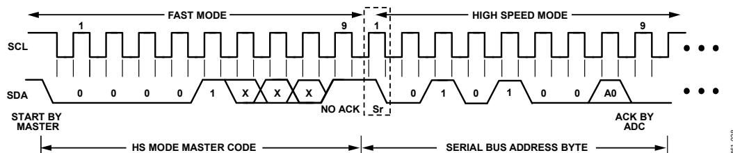
Figure 26. Placing the Part into High Speed Mode
