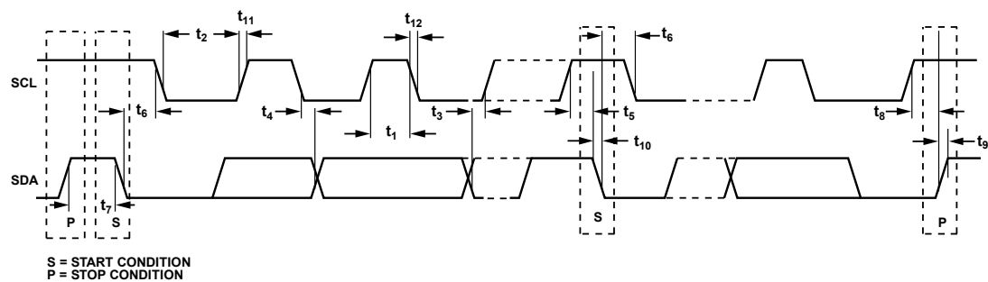
Figure 2. 2-Wire Serial Interface Timing Diagram
