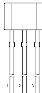
Package UA, 3-Pin SIP Pin-out Diagram
