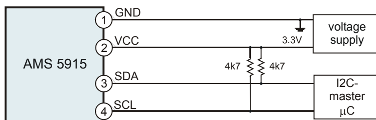
Figure 2: Principle electric circuitry
