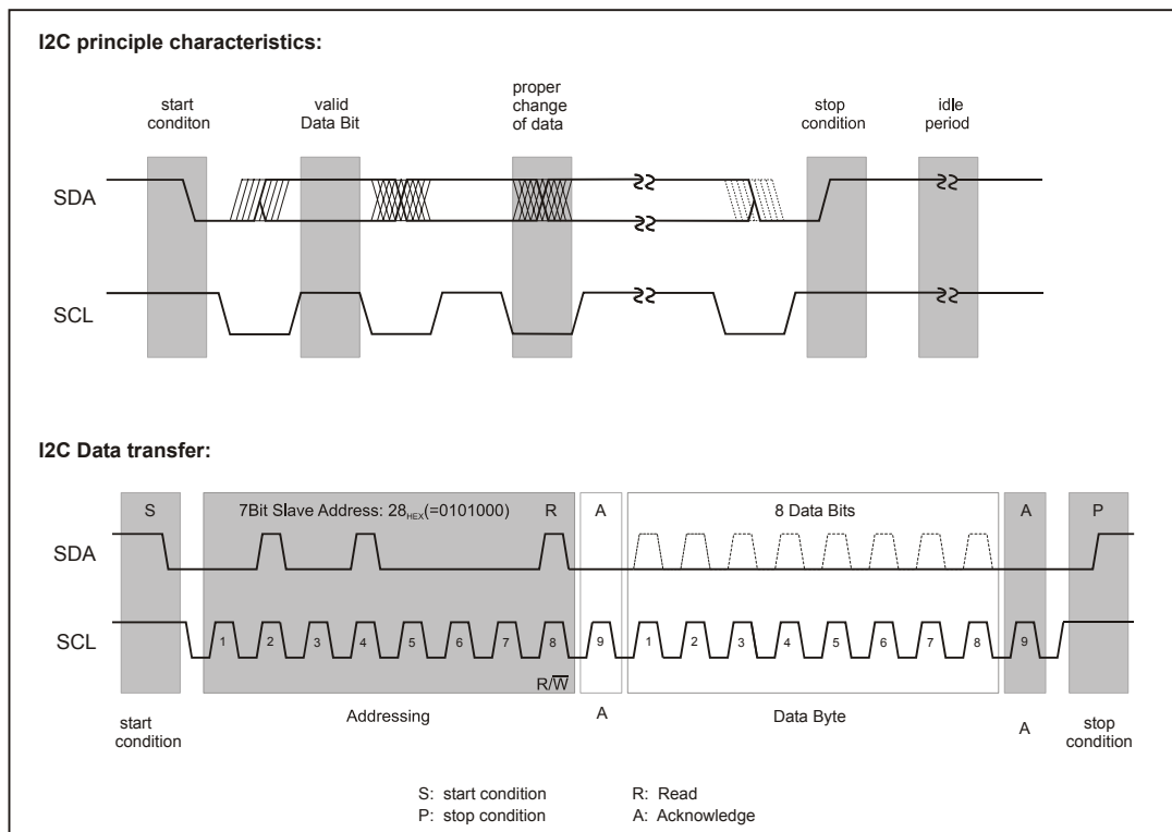
Figure 3: Standard I2C protocol
