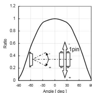
Fig.5 Directional Characteristics 2
