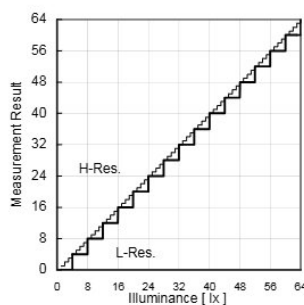
Fig.2 Illuminance - Measurement Result 1
