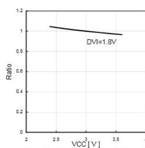
Fig.11 Measurement Result VCC Dependency
