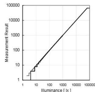
Fig.3 Illuminance - Measurement Result 2
