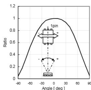
Fig.4 Directional Characteristics 1
