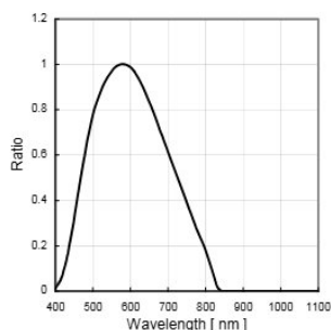
Fig.1 Spectral Response
