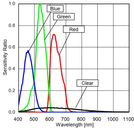
Figure 1. RGB Spectral Response
