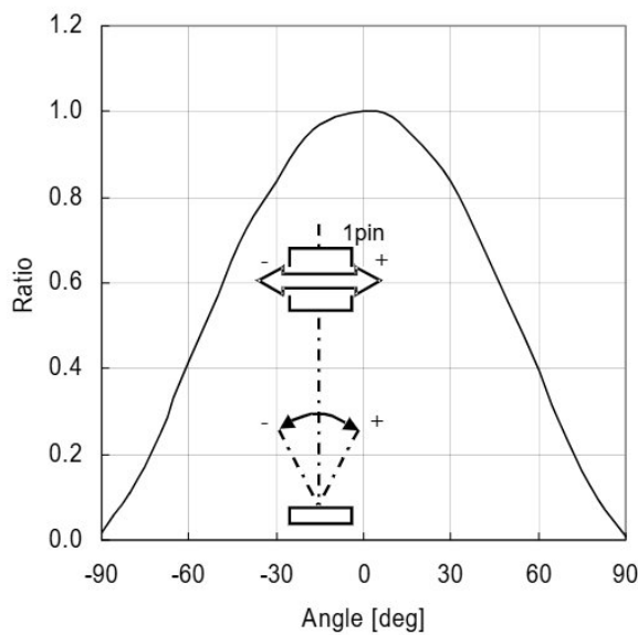
Figure 3. Directional Characteristics 1
