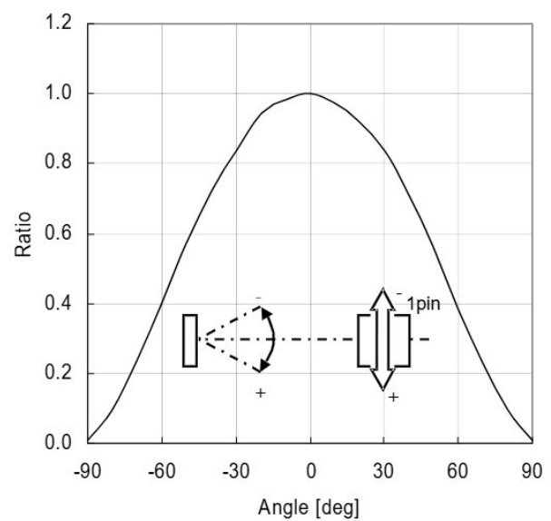
Figure 4. Directional Characteristics 2
