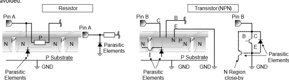
Figure xx. Example of monolithic IC structure
