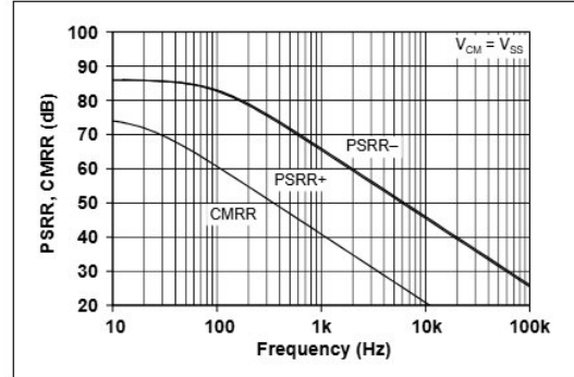
FIGURE 2-10: PSRR, CMRR vs. Frequency.
