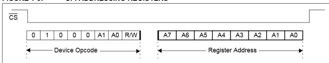
FIGURE 1-5: SPI ADDRESSING REGISTERS
