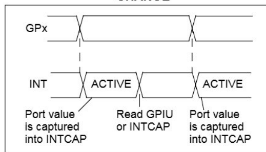
FIGURE 1-6: INTERRUPT-ON-PIN-CHANGE
