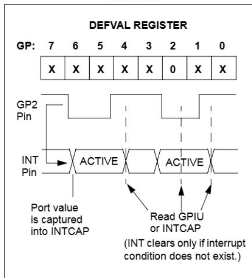
FIGURE 1-7: INTERRUPT-ON-CHANGE FROM REGISTER DEFAULT
