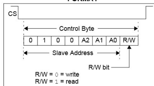
FIGURE 1-3: SPI CONTROL BYTE FORMAT
