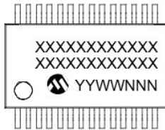
28-Lead SSOP
