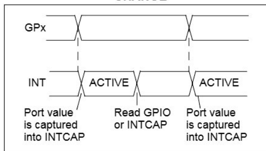
FIGURE 1-6: INTERRUPT-ON-PIN CHANGE
