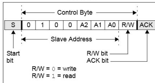
FIGURE 1-2: I 2 C™ CONTROL BYTE FORMAT
