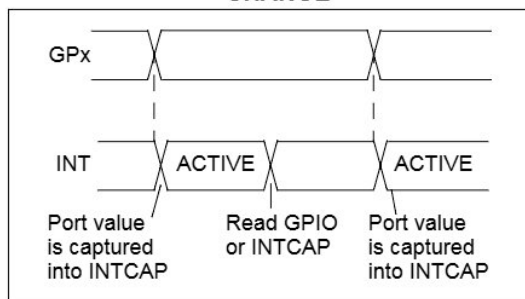
FIGURE 1-6: INTERRUPT-ON-PIN CHANGE
