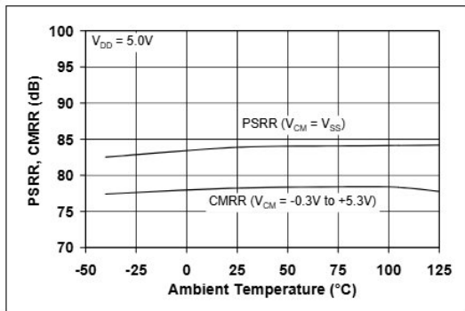
FIGURE 2-9: CMRR, PSRR vs. Ambient Temperature.
