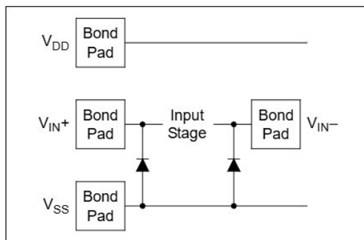
FIGURE 4-1: Simplified Analog Input ESD Structures.
