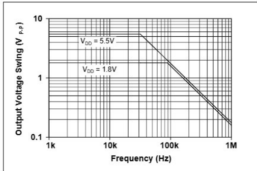
FIGURE 2-19: Output Voltage Swing vs. Frequency.
