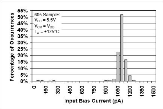
FIGURE 2-8: Input Bias Current at +125^\circ\text{C} .
