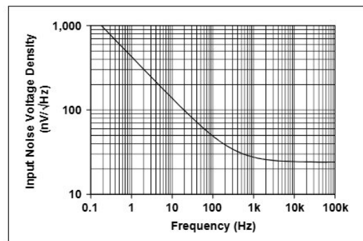
FIGURE 2-12: Input Noise Voltage Density vs. Frequency.
