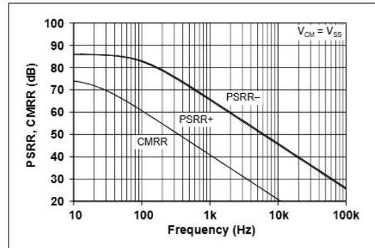
FIGURE 2-10: PSRR, CMRR vs. Frequency.
