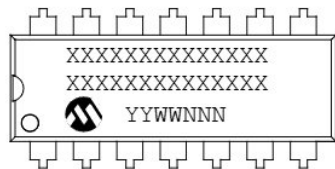
14-Lead PDIP (300 mil) (MCP6004)
