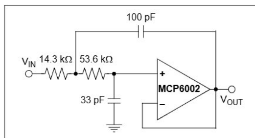
FIGURE 4-8: Active Second-Order Low-Pass Filter.
