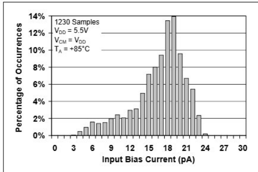
FIGURE 2-7: Input Bias Current at +85^\circ\text{C} .
