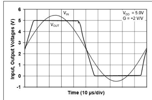
FIGURE 2-21: The MCP6001/2/4 Show No Phase Reversal.
