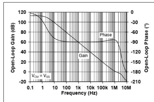
FIGURE 2-11: Open-Loop Gain, Phase vs. Frequency.
