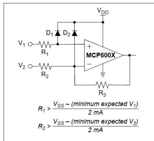
FIGURE 4-2: Protecting the Analog Inputs.
