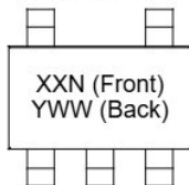
5-Lead SC-70 (MCP6001)
