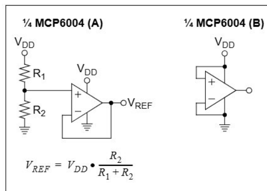
FIGURE 4-5: Unused Op Amps.
