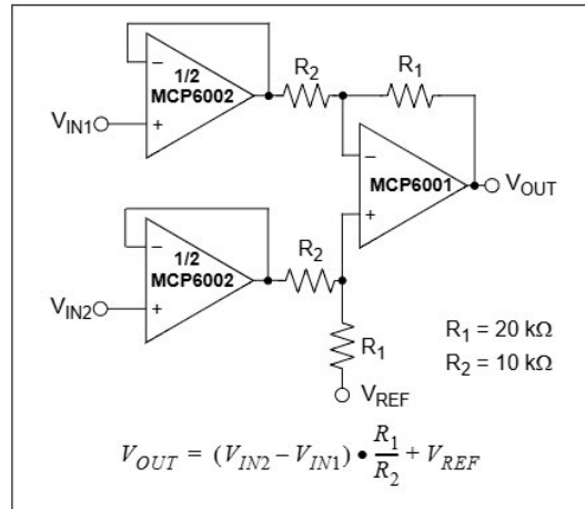
FIGURE 4-7: Instrumentation Amplifier with Unity-Gain Buffer Inputs.
