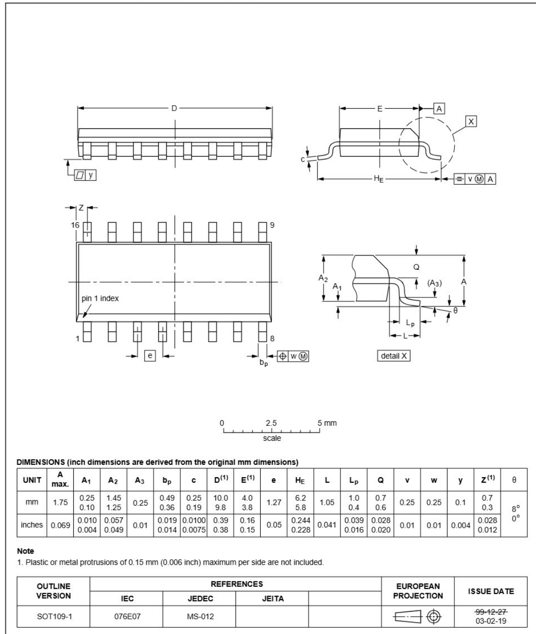
Fig 23. Package outline SOT109-1 (SO16)
