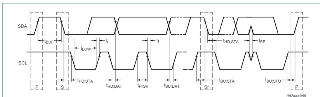
Fig 20. Definition of timing
