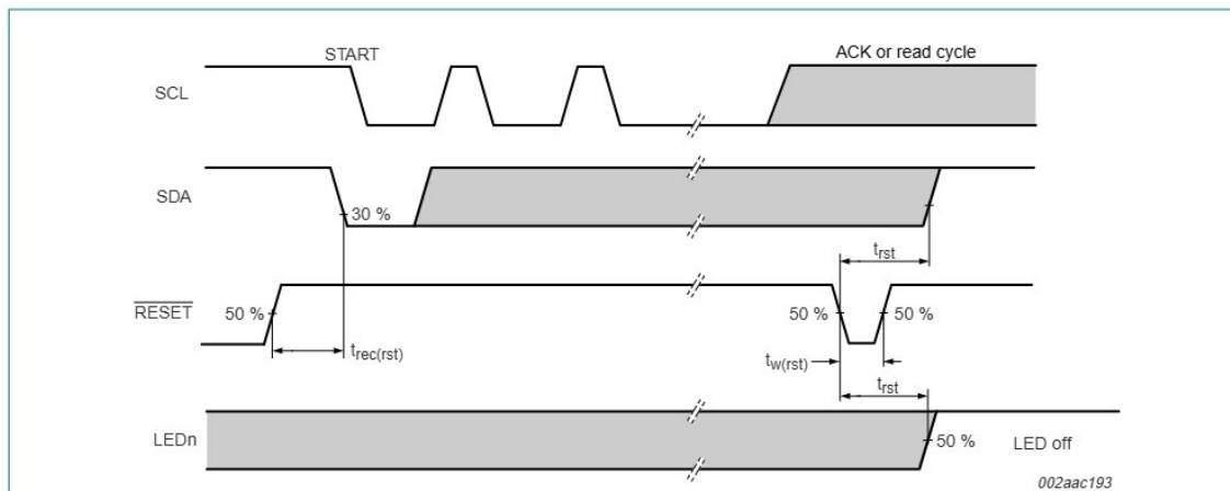
Fig 19. Definition of RESET timing
