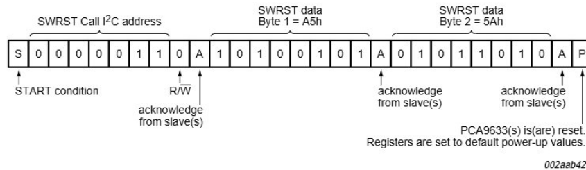
Fig 21. Software Reset (SWRST) Call sequence
