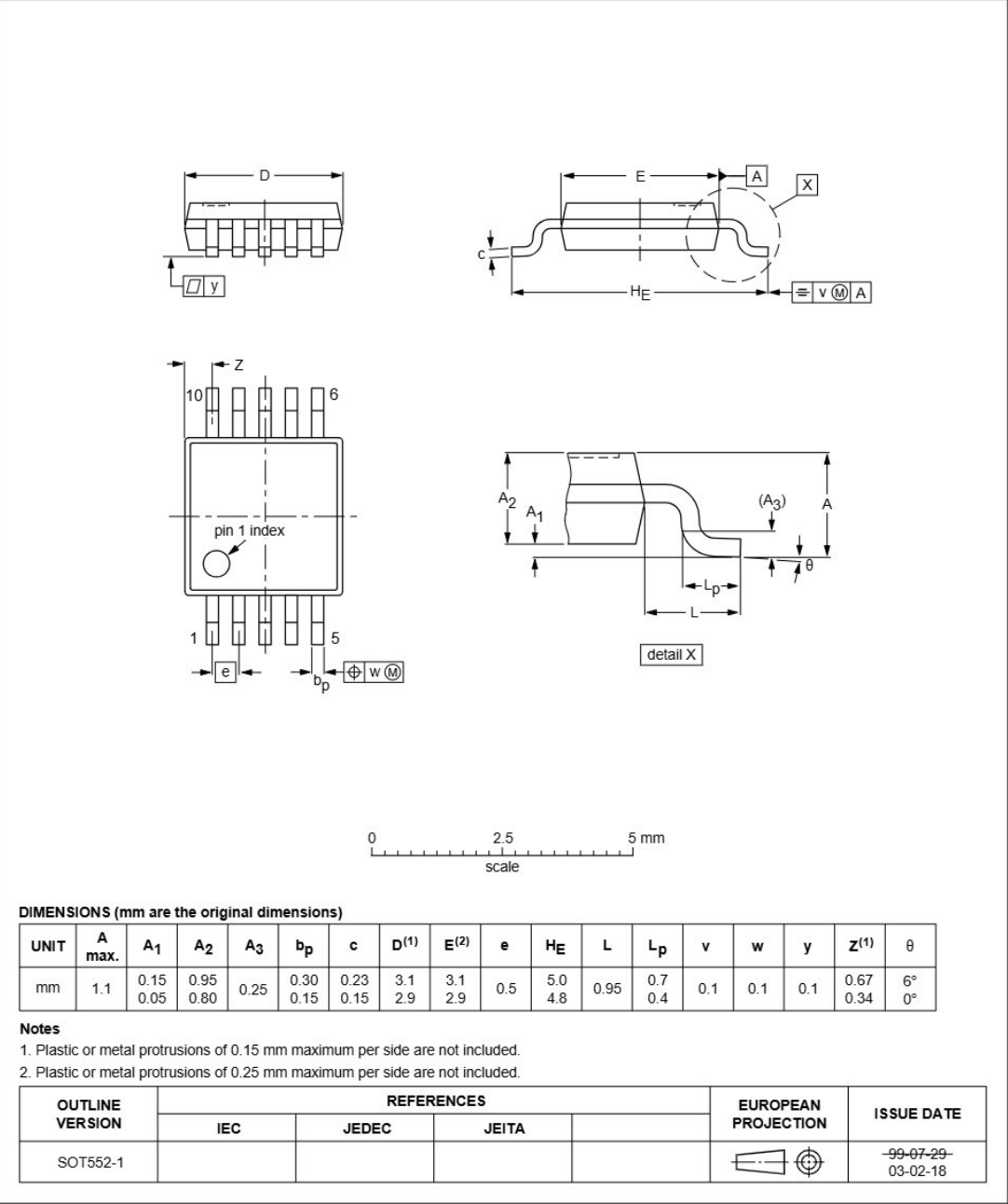
Fig 28. Package outline SOT552-1 (TSSOP10)
