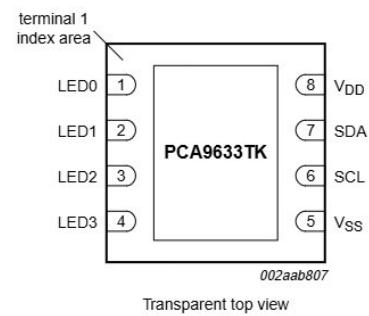
Fig 7. Pin configuration for HVSON8
