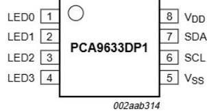
Fig 2. Pin configuration for TSSOP8
