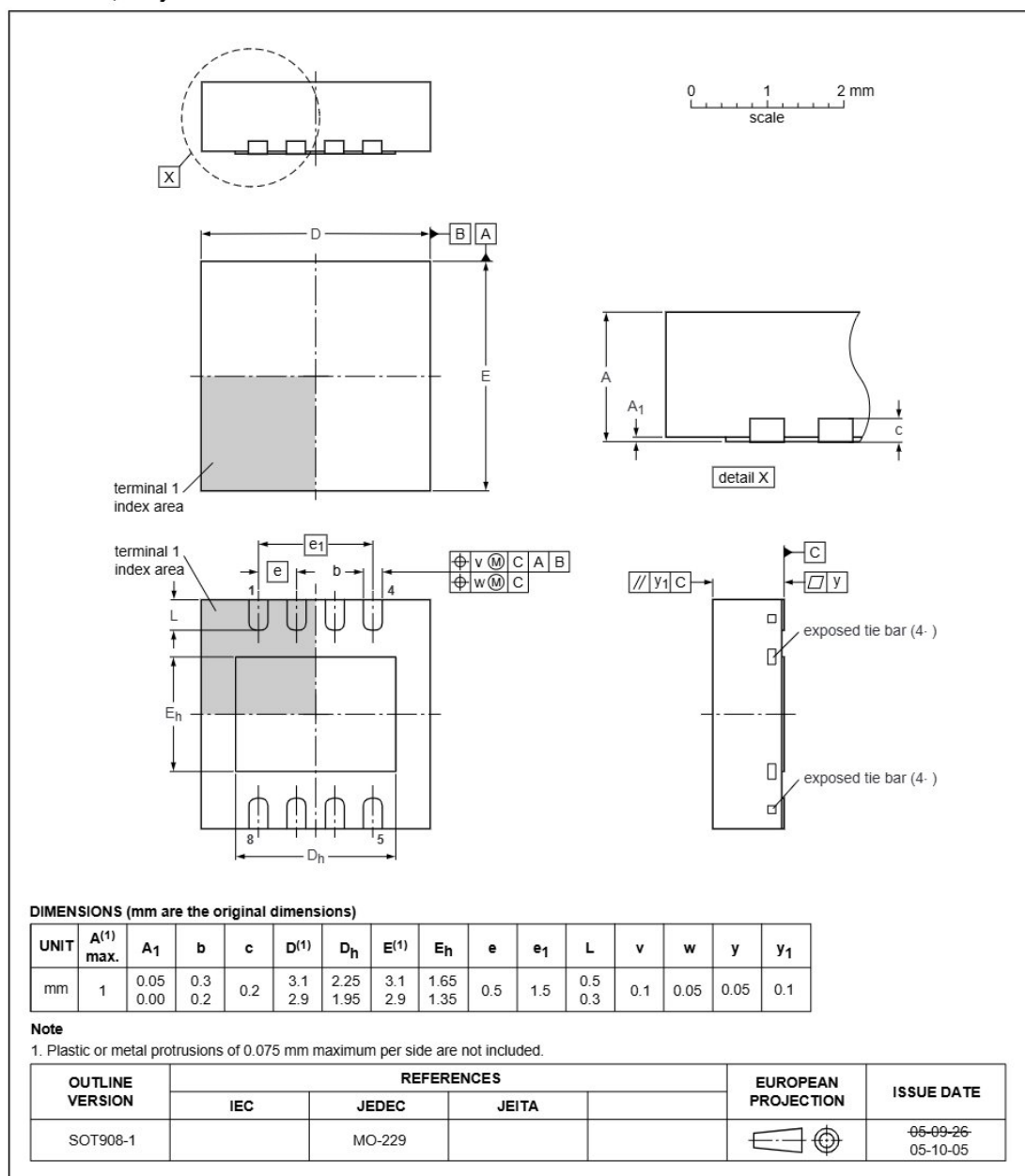
Fig 31. Package outline SOT908-1 (HVSON8)
