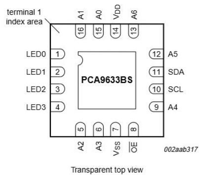
Fig 6. Pin configuration for HVQFN16
