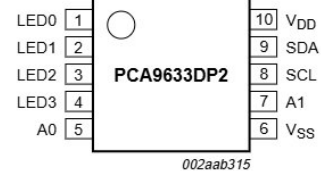
Fig 3. Pin configuration for TSSOP10
