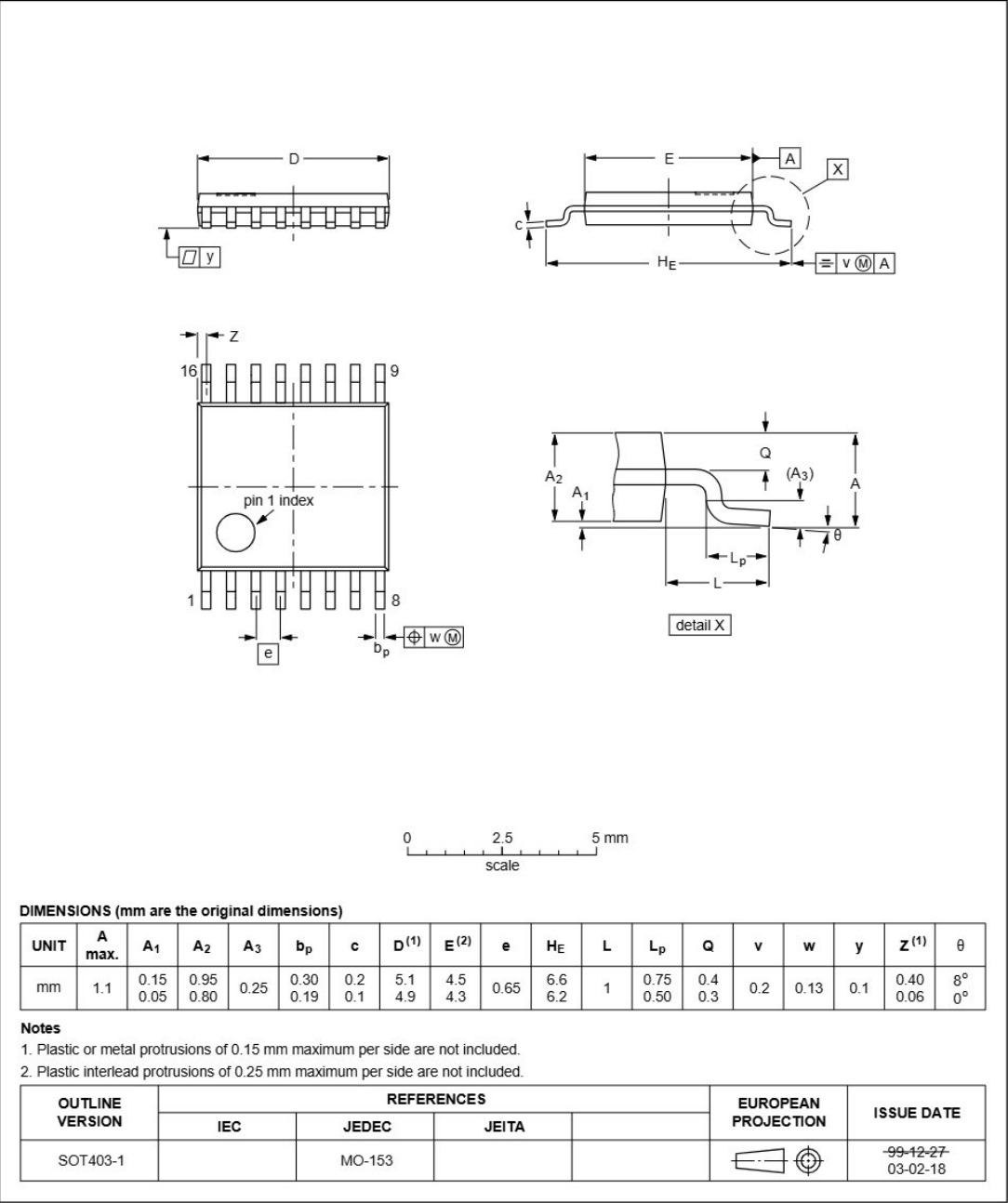
Fig 29. Package outline SOT403-1 (TSSOP16)
