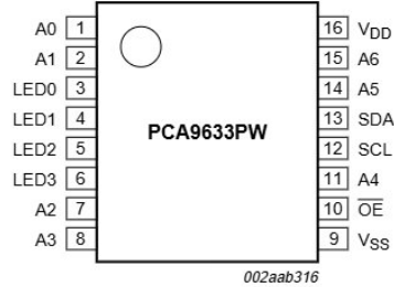
Fig 4. Pin configuration for TSSOP16
