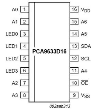
Fig 5. Pin configuration for SO16
