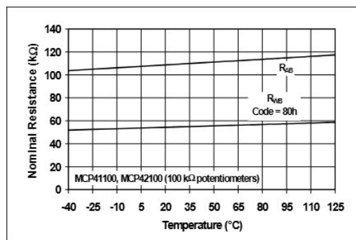
FIGURE 2-6: Nominal Resistance 100 k \Omega vs. Temperature.
