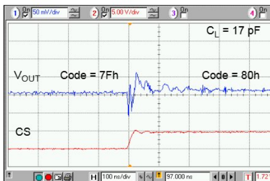
FIGURE 2-15: One Position Settling Time.
