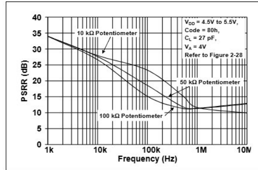
FIGURE 2-22: Power Supply Rejection Ratio vs. Frequency.
