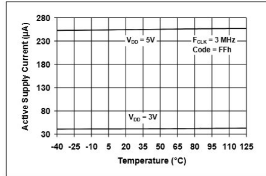
FIGURE 2-10: Active Supply Current vs. Temperature.
