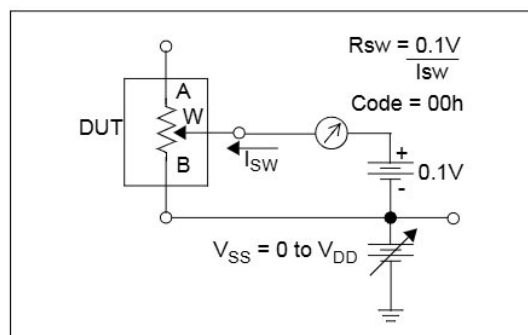
FIGURE 2-27: Wiper Resistance Test Circuit.
