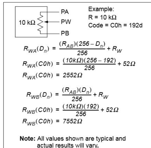
FIGURE 4-10: Example Resistance calculations.
