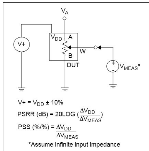
FIGURE 2-28: Power Supply Sensitivity Test Circuit (PSS, PSRR).
