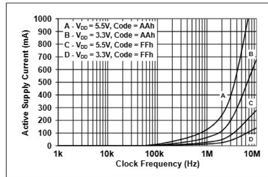
FIGURE 2-11: Active Supply Current vs. Clock Frequency.
