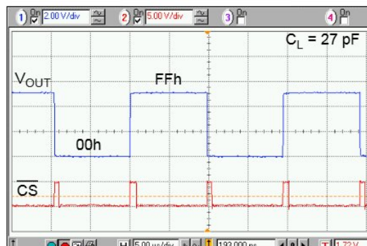
FIGURE 2-16: Full-Scale Settling Time.
