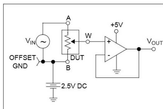
FIGURE 2-29: Gain vs. Frequency Test Circuit.
