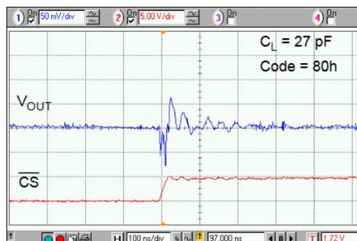
FIGURE 2-17: Digital Feed through vs. Time.
