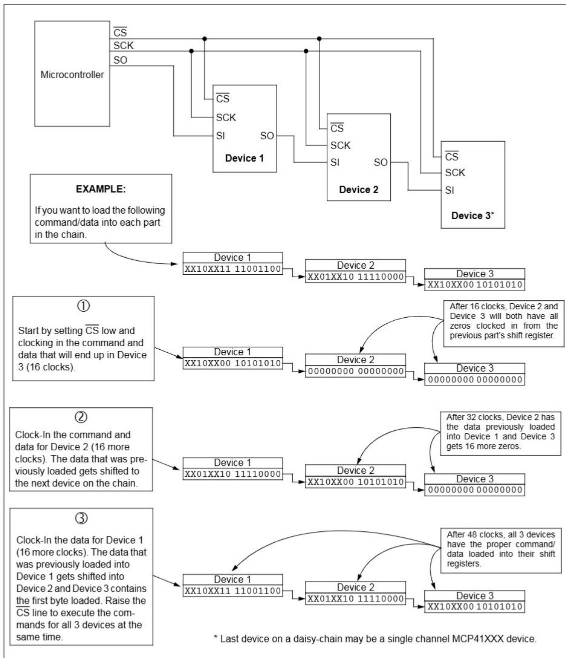
FIGURE 5-4: Daisy-Chain Configuration.
