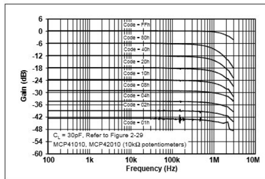
FIGURE 2-18: Gain vs. Frequency for 10 k \Omega Potentiometer.
