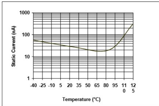
FIGURE 2-9: Static Current vs. Temperature.
