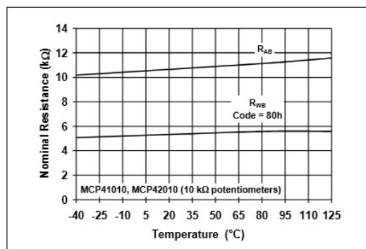
FIGURE 2-4: Nominal Resistance 10 k \Omega vs. Temperature.
