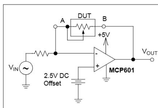
FIGURE 2-30: Capacitance Test Circuit.
