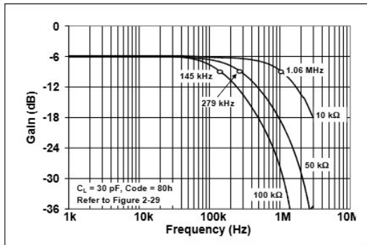
FIGURE 2-21: -3 dB Bandwidths.
