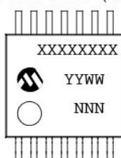
14-Lead TSSOP (4.4mm) *
