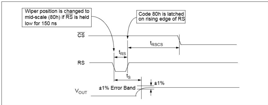
FIGURE 1-2: Reset Timing.
