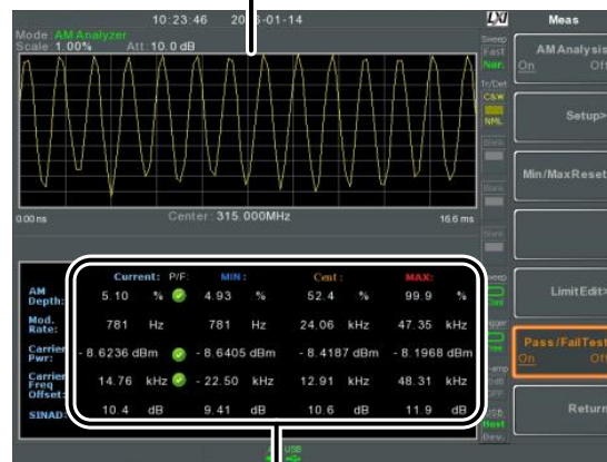
AM modulation measurements
