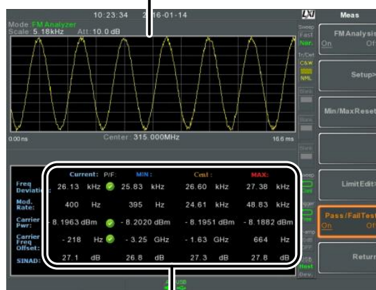
FM modulation measurements
