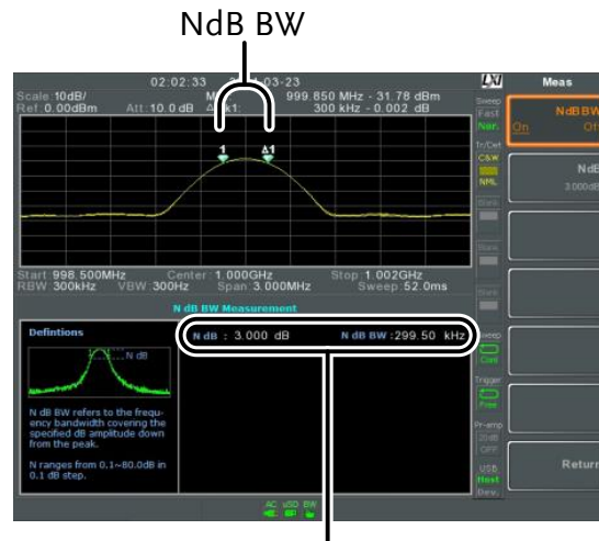
N dB BW Measurement
