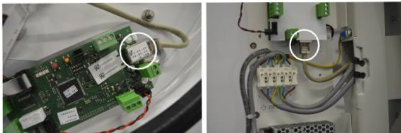
RJ45 Ethernet port: Single-sided (left) and Double-sided (right)
