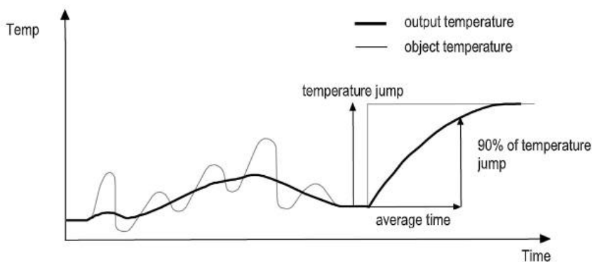
Figure 35: Averaging
