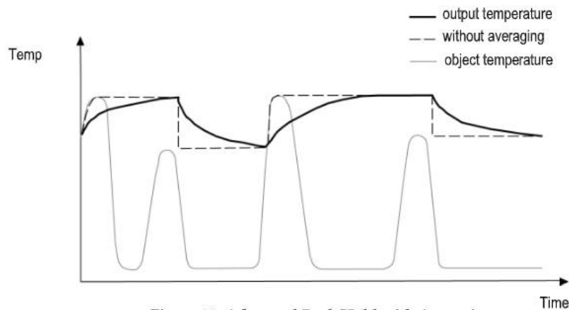
Figure 39: Advanced Peak Hold with Averaging
