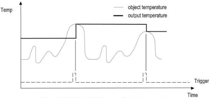
Figure 30: FTC3 for Holding the Output Temperature
