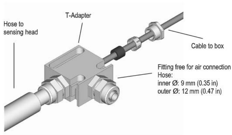
Figure 60: Connecting the T-Adapter
