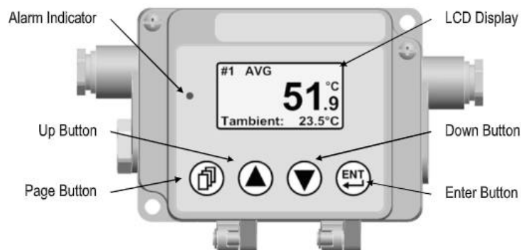
Figure 32: Control Panel for the Comm Box (metal)
