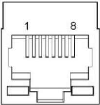
Figure 89: RJ45 Connector Socket and Pin Assignment
