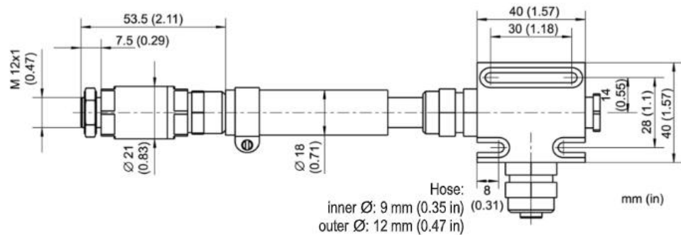
Figure 63: Dimensions of Air Cooling System
