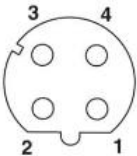
Figure 88: M12 Connector Socket and Pin Assignment
