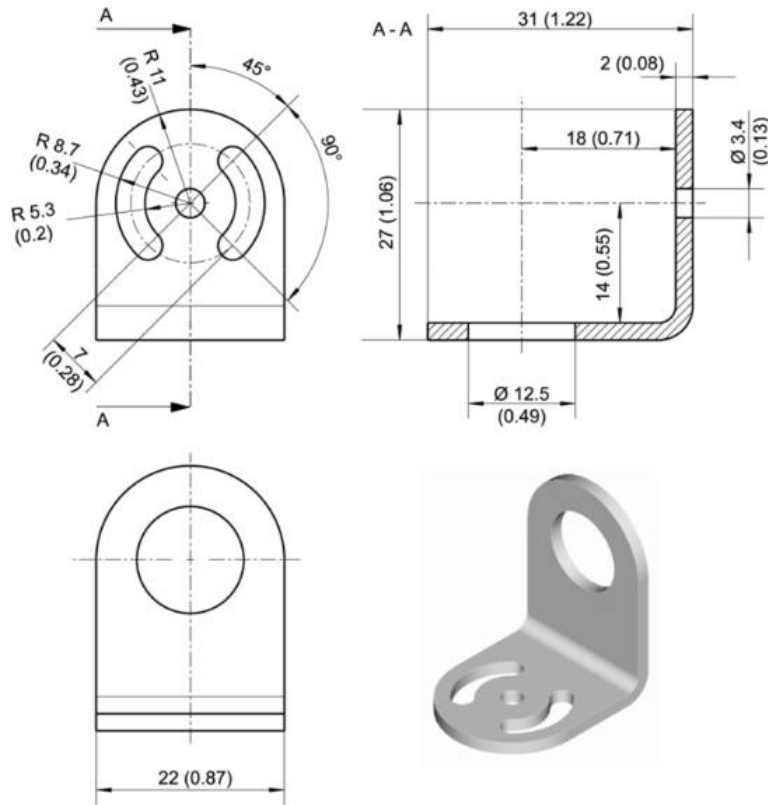
Figure 56: Fixed Mounting Bracket (XXXMIACFB)
