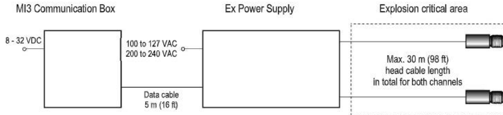
Figure 42: Basic Installation in the Explosion Critical Area
