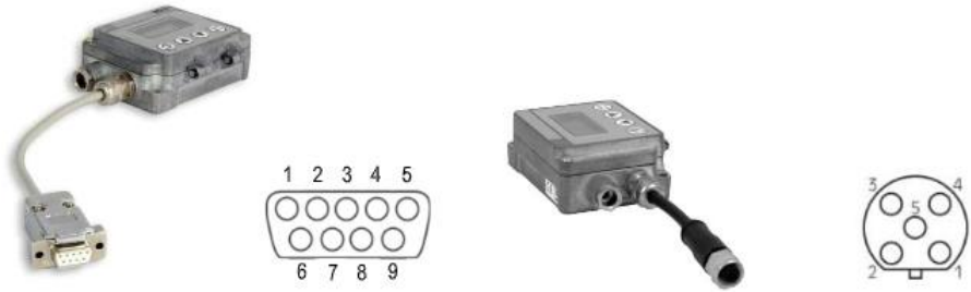
Figure 80: Sub-D Connector (...P2) and M12 Connector (...P1)
