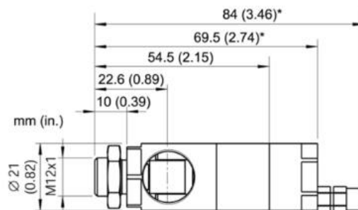
Figure 65: Right Angle Mirror (* with Air Purge)
