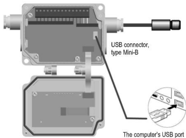
Figure 21: USB Connection via the Comm Box (metal)
