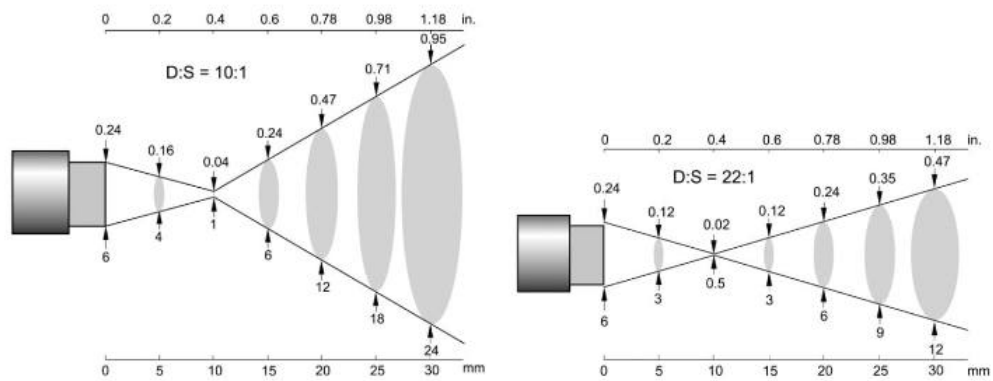
Figure 68: Spot Size Charts for Close Focus Lens
