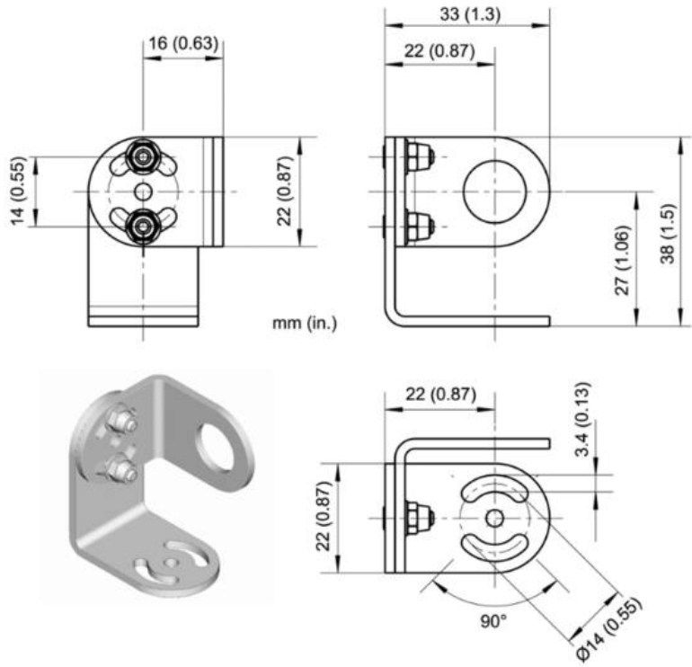
Figure 55: Adjustable Mounting Bracket (XXXMIACAB)
