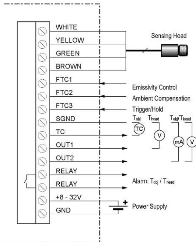
Figure 14: Terminal Wiring for the Comm Box
