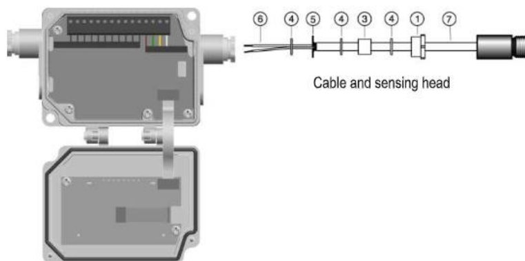
Figure 13: Sensing Head Cable to the Comm Box
