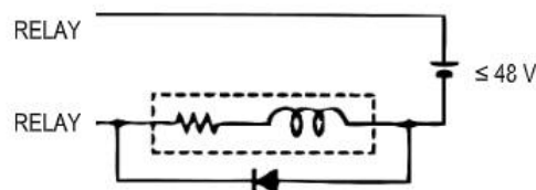
Figure 24: Spike Voltage Limitation for the Alarm Relay
