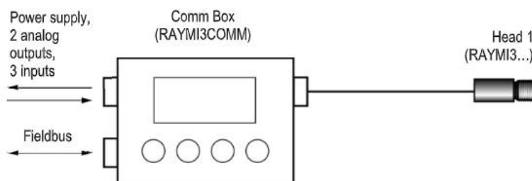
Figure 11: Single Head Configuration with Comm Box
