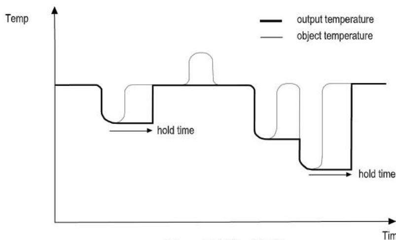
Figure 37: Valley Hold
