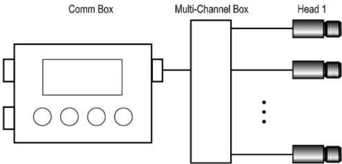
Figure 48: Multiple Head Configuration with Comm Box
