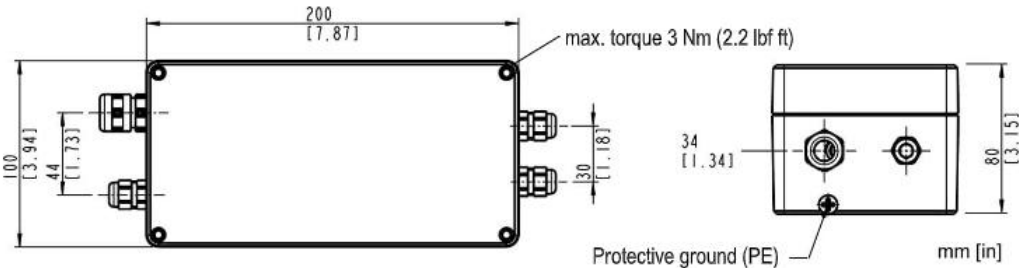
Figure 41: Dimensions of Housing for Ex Power Supply
