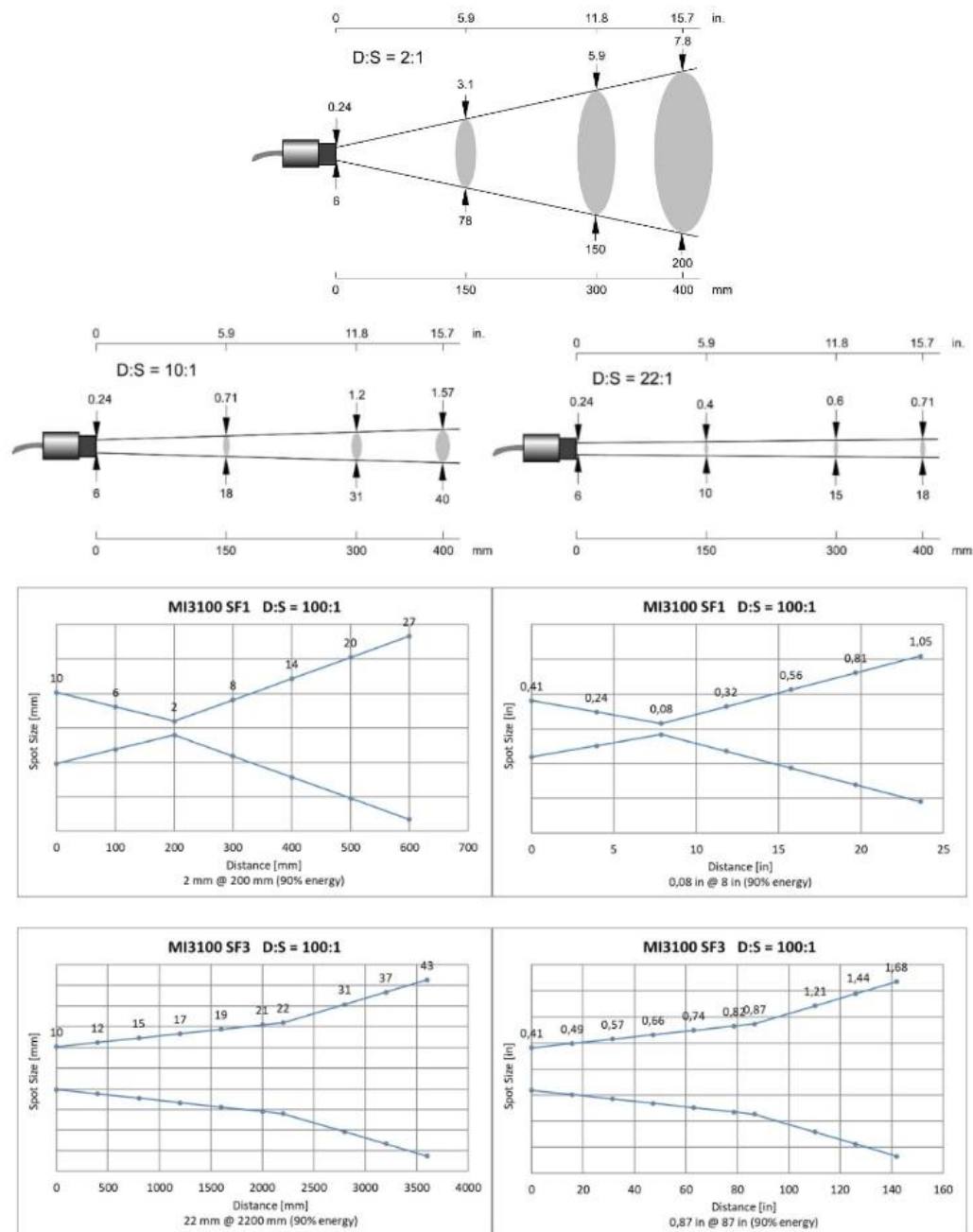
Figure 1: Spot Size Charts
