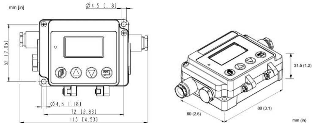
Figure 5: Dimensions of Communication Box
