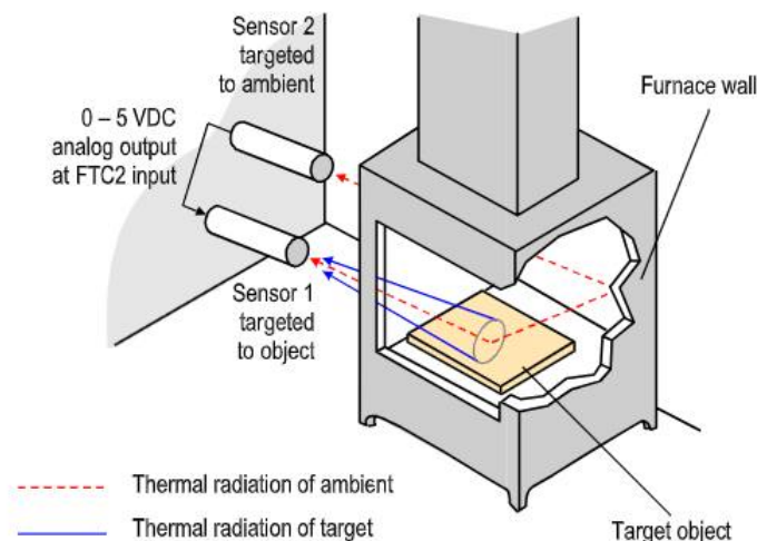
Figure 27: Principle of Ambient Background Temperature Compensation
