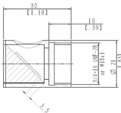
Figure 75: Dimension of Right Angle Mirror (XXXMI3100RAM)
