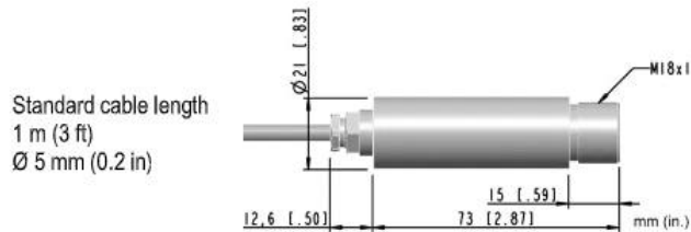
Figure 4: Dimensions of 1M, 2M Sensing Heads
