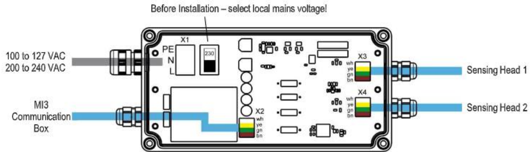
Figure 44: External Wiring of the Ex Power Supply
