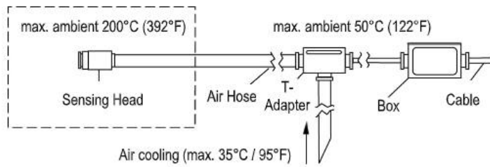
Figure 59: Air Cooling System (XXXMIACCJ)
