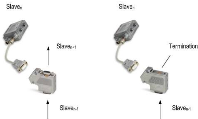
Figure 82: Exemplary Network with External Termination
