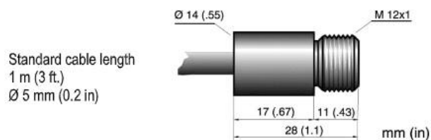
Figure 2: Dimensions of LT, G5 Sensing Heads
