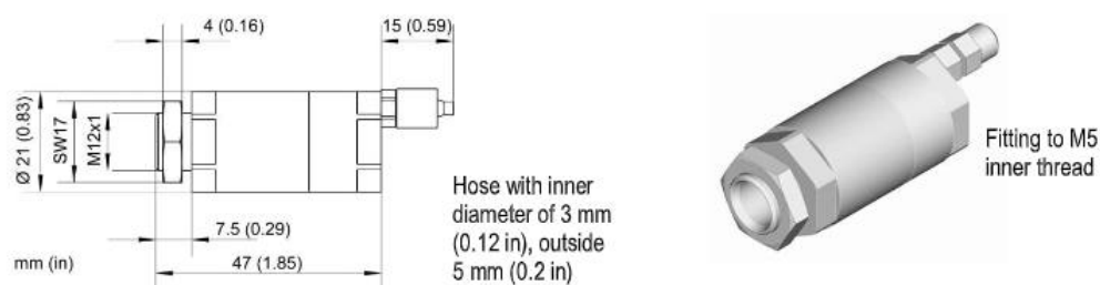
Figure 57: Air Purge Jacket (XXXMIACA)
