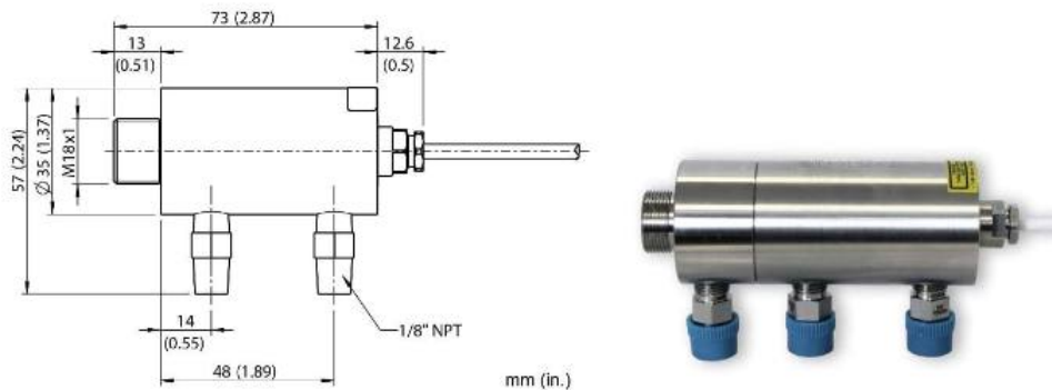
Figure 40: Water Cooled Housing
