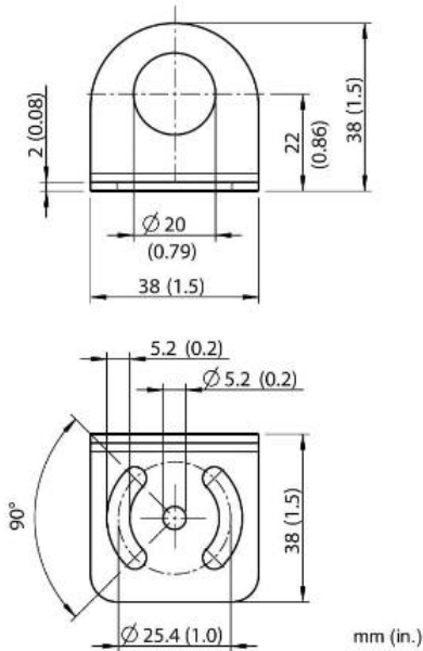
Figure 70: Dimensions of Fixed Mounting Bracket (XXXMI3100FB)
