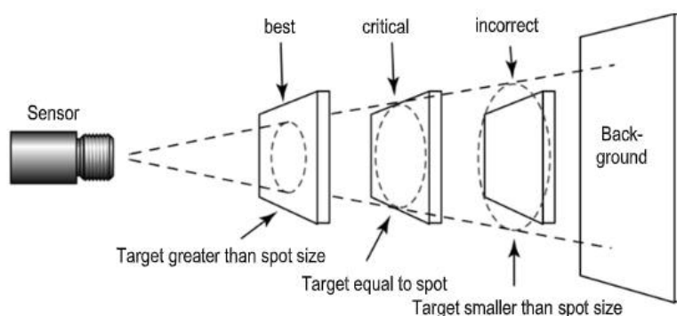
Figure 10: Proper Sensor Placement
