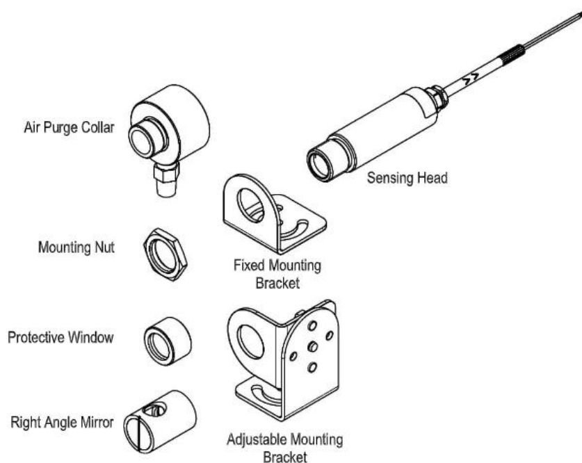
Figure 69: Overview of available accessories
