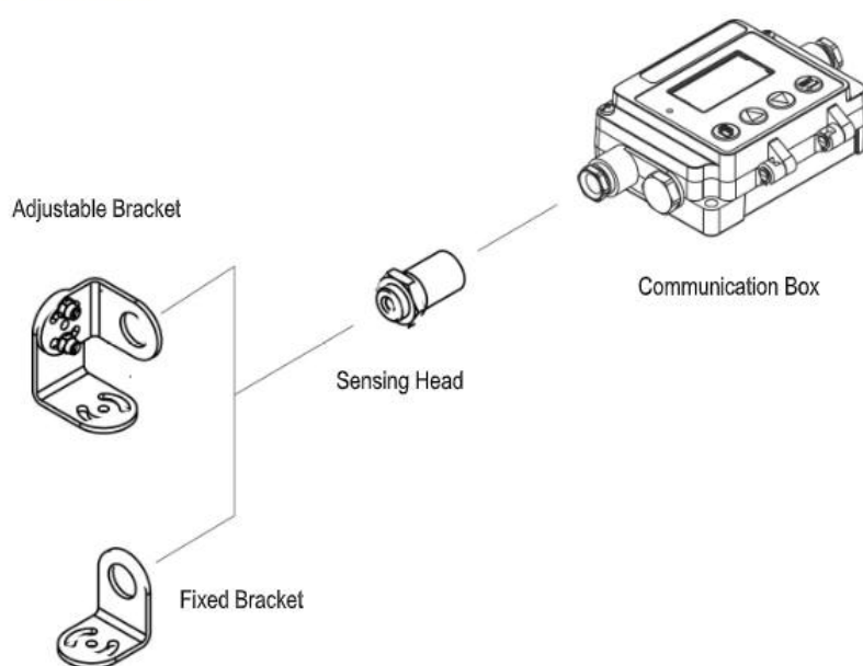
Figure 54: Standard Accessories for LT, G5 Heads
