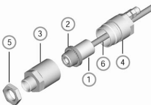
Figure 58: Mounting the Air Purge Jacket
