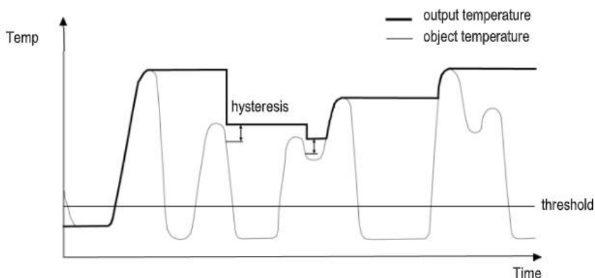
Figure 38: Advanced Peak Hold
