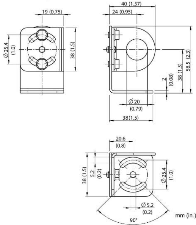
Figure 71: Dimensions of Adjustable Mounting Bracket (XXXMI3100ADJB)
