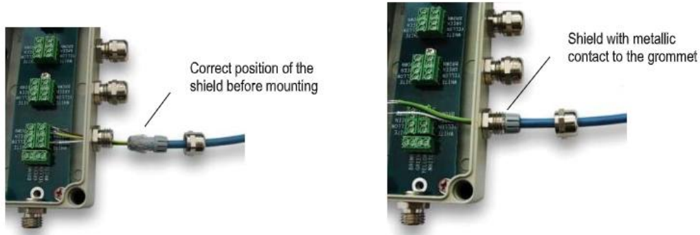
Figure 51: Correct Mounting of the Cable Shield
