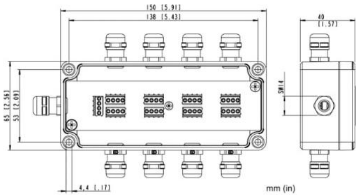
Figure 49: Dimensions
