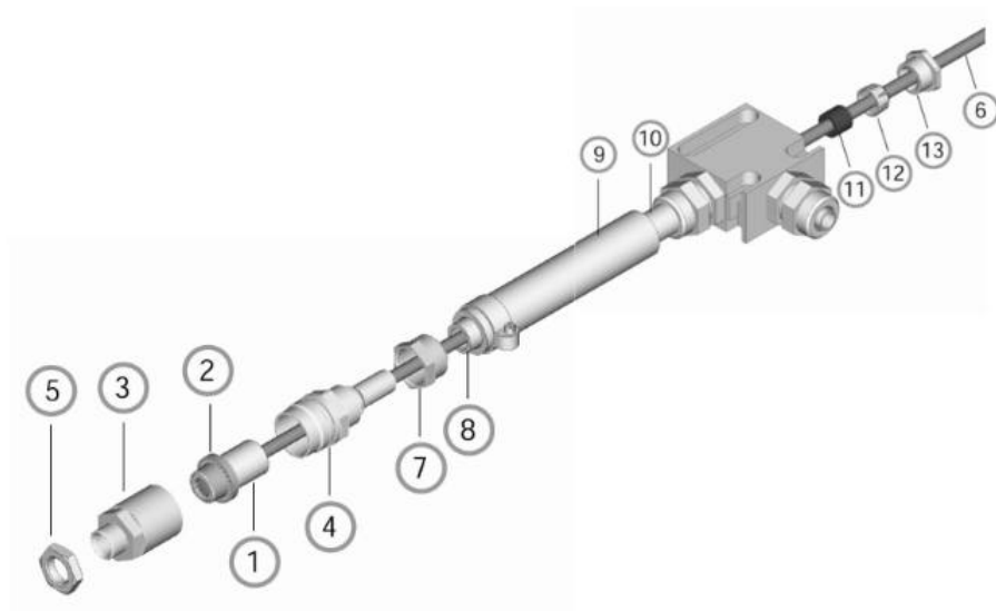
Figure 62: Air Cooling System: Purging Jacket and T-Adapter
