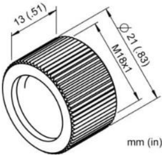
Figure 76: Protective Window
