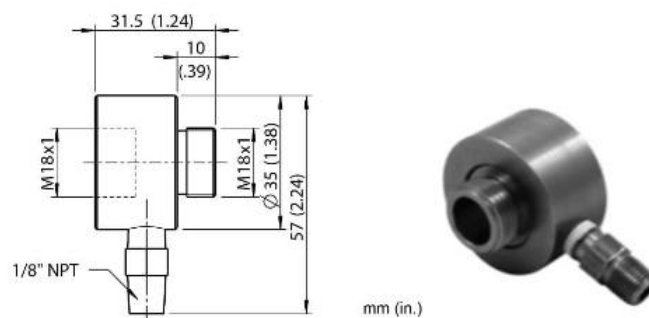
Figure 74: Dimensions of Air Purge Collar (XXXMI3100AP)
