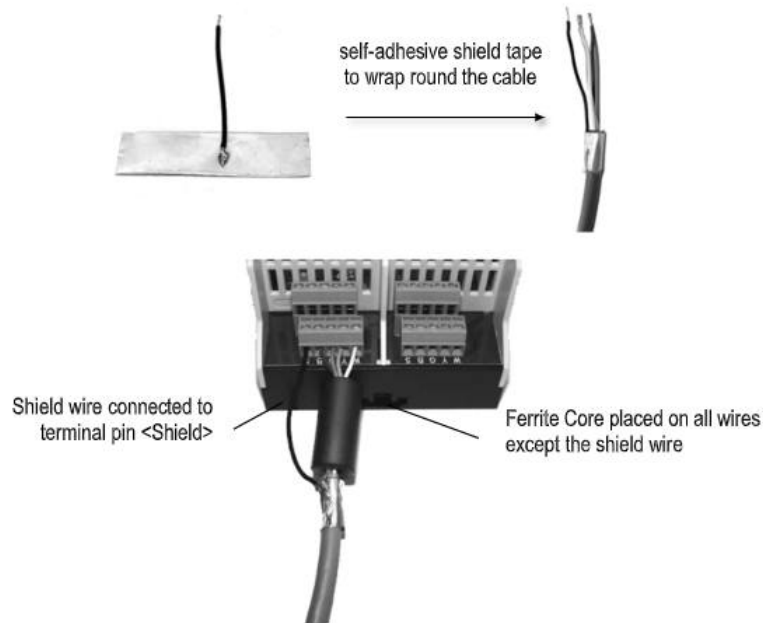
Figure 20: Mounting of Shield Wire and Ferrite Core
