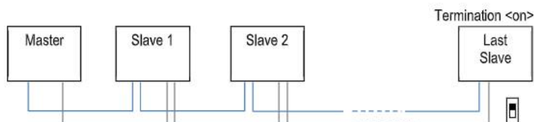
Figure 23: Network in Linear Topology (daisy chain)
