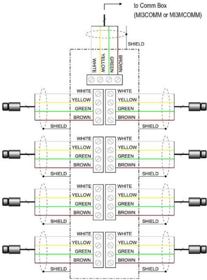
Figure 50: Wiring Diagram for 8 Heads
