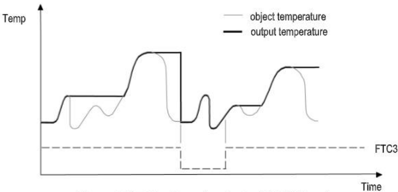
Figure 29: FTC for Resetting the Peak Hold Function
