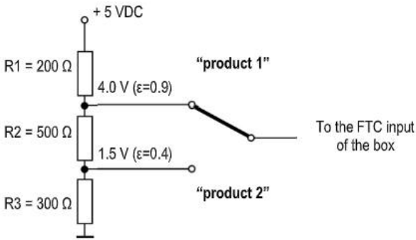
Figure 25: Adjustment of Emissivity at FTC Input (Example)
