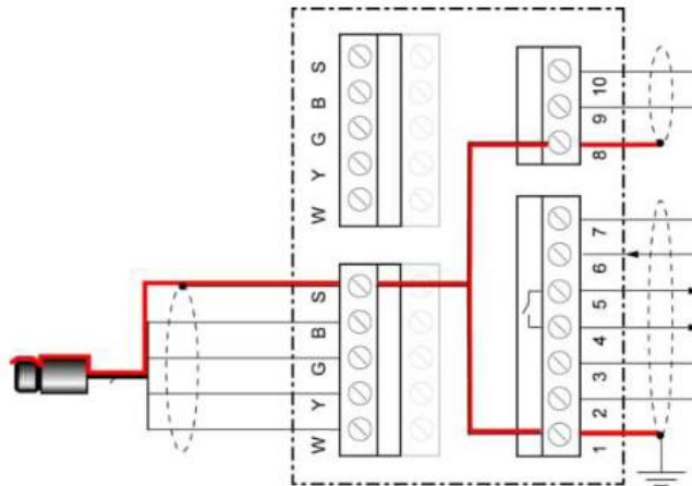
Figure 8: Shield Run for Comm Box (DIN)
