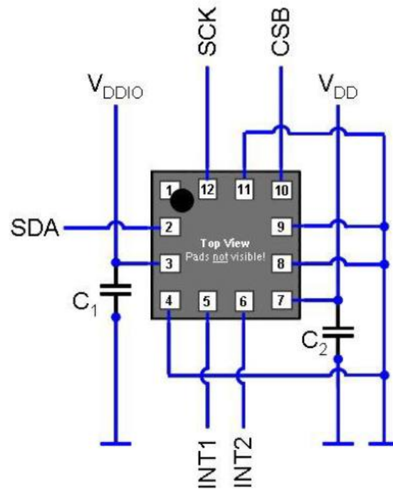
Figure 25: 3-wire SPI connection
