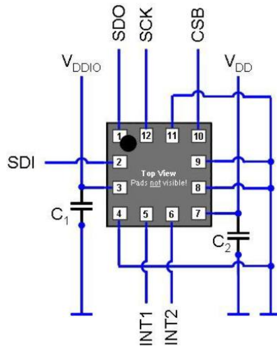
Figure 24: 4-wire SPI connection
