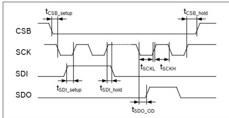
Figure 13: SPI timing diagram
