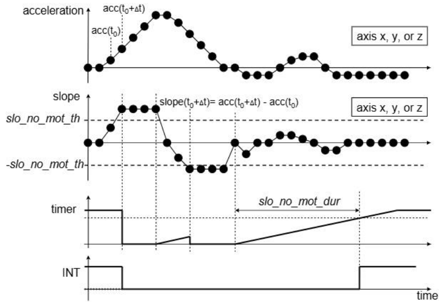
Figure 11: Timing of No-motion interrupt
