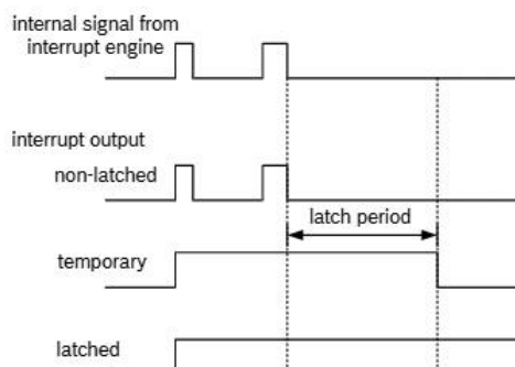
Figure 6: Interrupt modes
