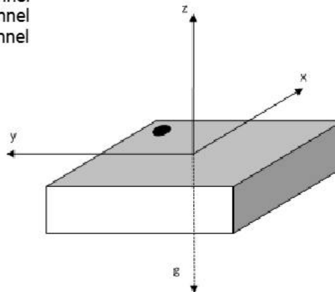
Figure 28: Orientation of sensing axis
