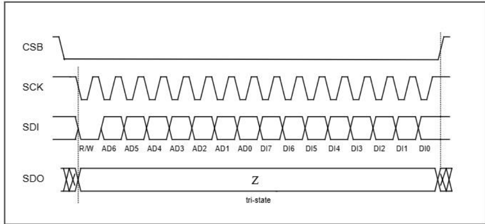
Figure 14: 4-wire basic SPI write sequence (mode '11')
