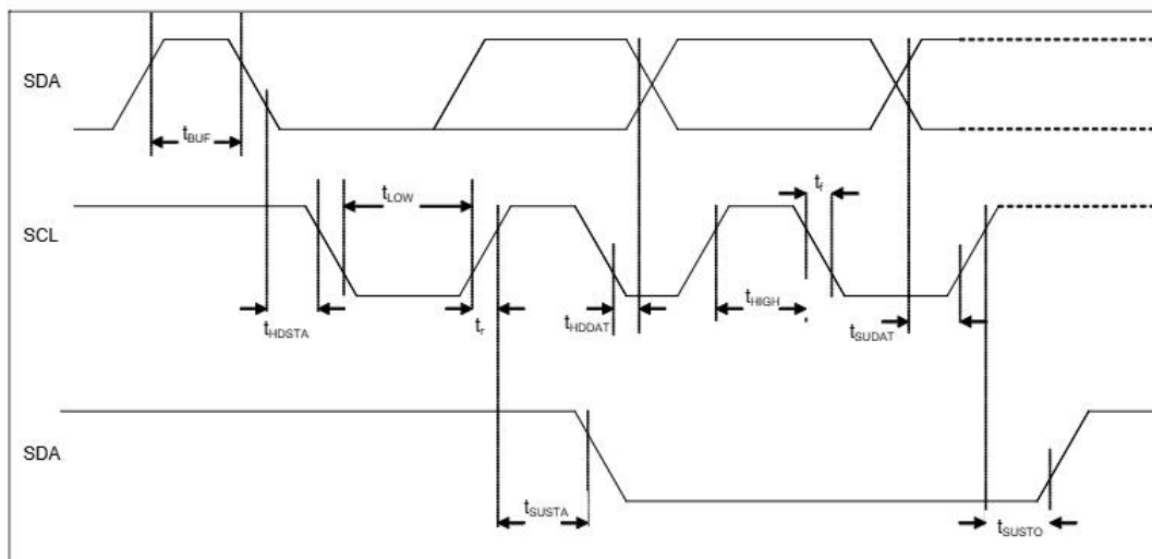
Figure 18: I 2 C timing diagram
