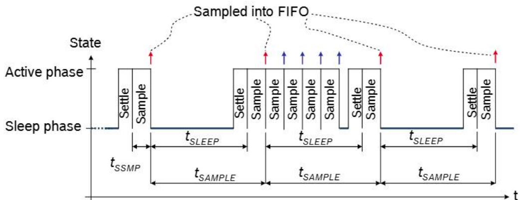
Figure 4: Timing Diagram for low-power mode 1/2, EST
