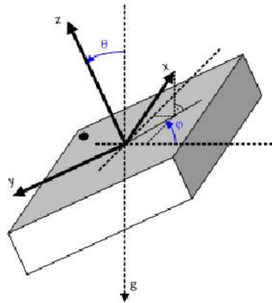
Figure 9: Definition of vector components
