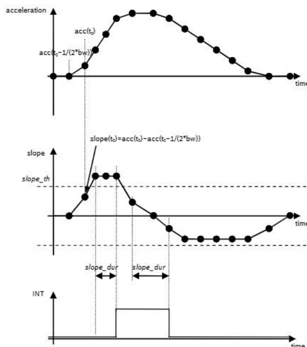
Figure 7: Principle of any-motion detection
