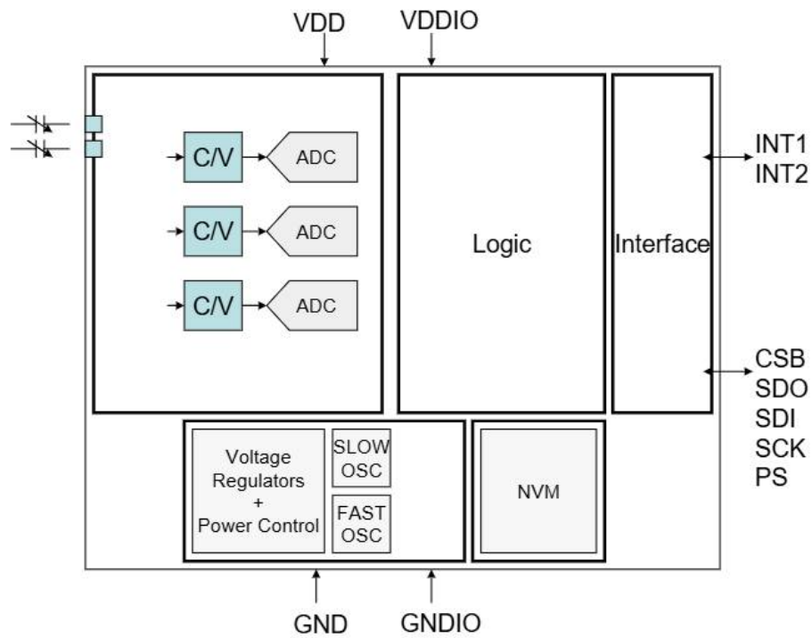
Figure 1: Block diagram of BMA250E
