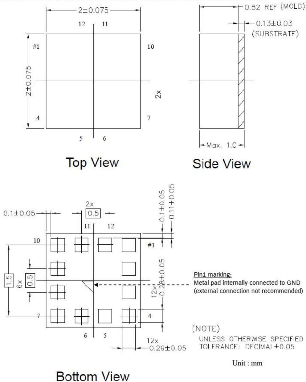
Figure 27: Package outline dimensions
