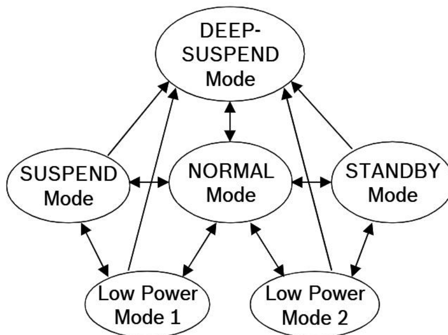
Figure 2: Power mode transition diagram
