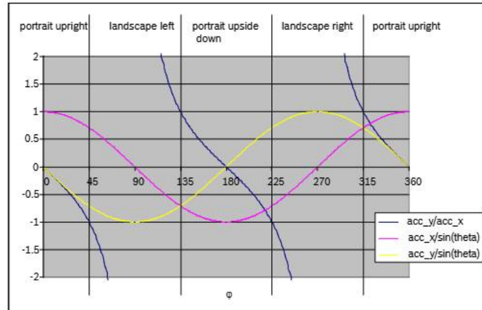
Figure 10: Typical orientation switching conditions w/o hysteresis
