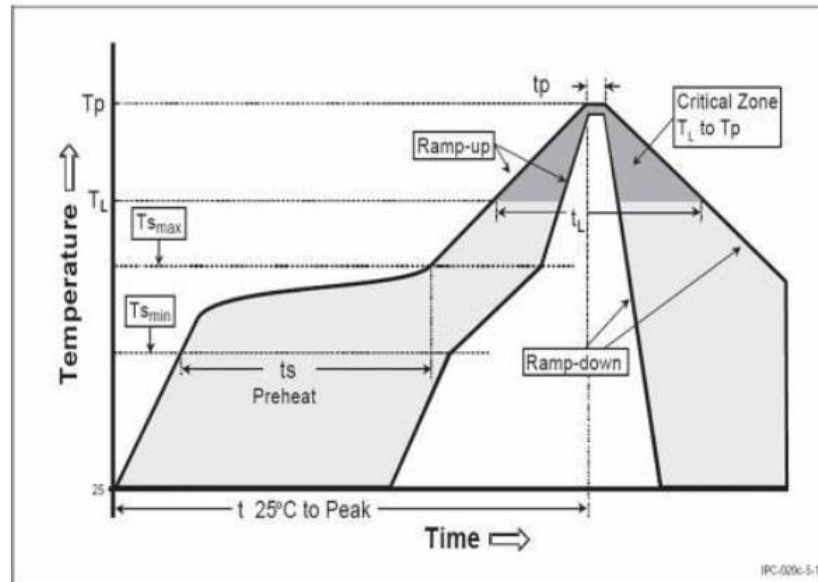
Figure 30: Soldering profile
