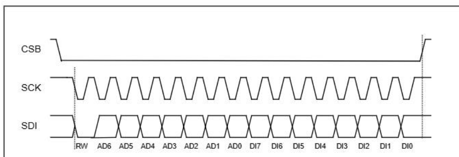
Figure 17: 3-wire basic SPI read or write sequence (mode '11')
