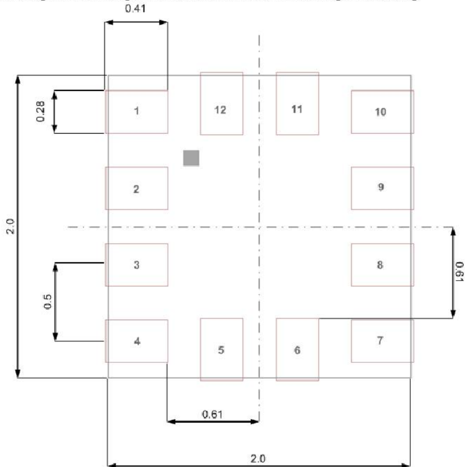
Figure 29: Landing patterns; dimensions are in mm
