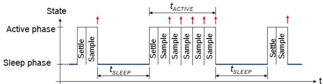
Figure 3: Timing Diagram for low-power mode 1/2, EDT
