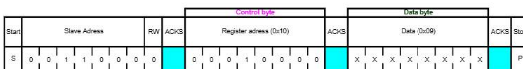
Figure 19: I 2 C write
