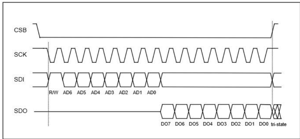
Figure 15: 4-wire basic SPI read sequence (mode '11')
