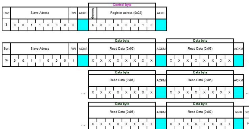
Figure 20: I 2 C multiple read
