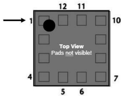
Figure 22: Pin-out top view
