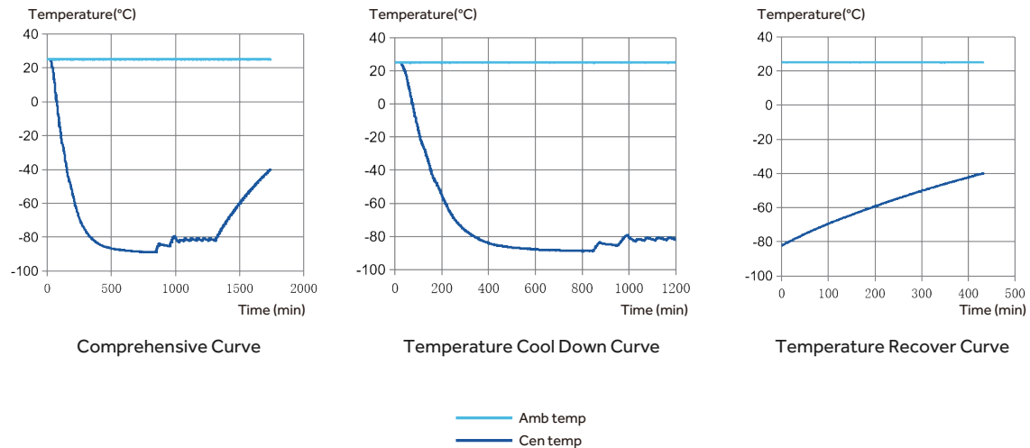
DW-86L959BPT Typical Performance Characteristics
