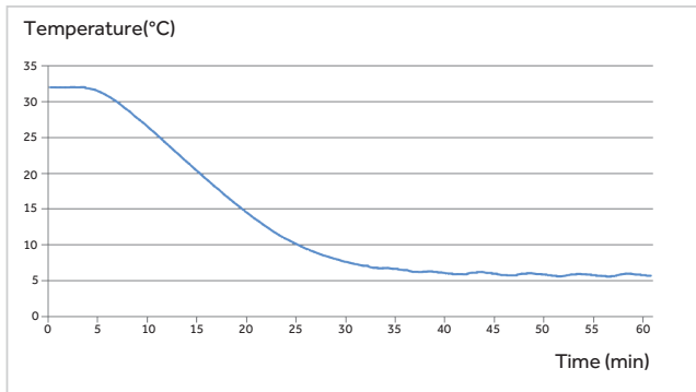
Refrigerator Stability Curve
