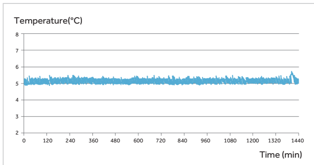
Refrigerator Stability Curve
