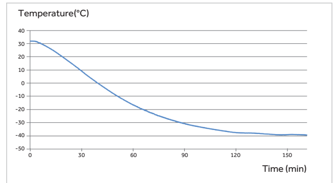
Freezer Stability Curve
