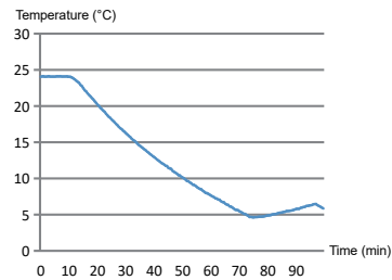
Refrigerator Running Curve
